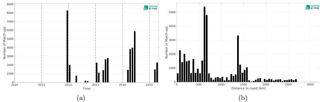
Figure 2: Number of match-ups between TSG (GOSUD-Research-vessel) and Aquarius SSS L3 OR v5 - Monthly (NASA-GSFC) SSS as a function of time (a) and as function of the distance to coast (b) over the South Atlantic Ocean Pi-MEP region and for the full satellite product period.
