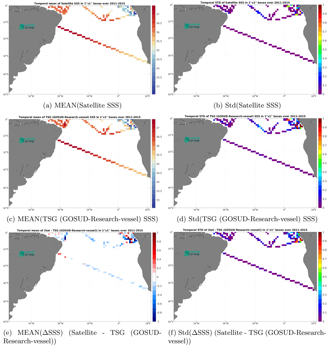
Figure 7: Temporal mean (left) and Std (right) of SSS from Aquarius SSS L3 OR v5 - Monthly (NASA-GSFC) (top), TSG (GOSUD-Research-vessel) (middle), and of \Delta SSS (Satellite - TSG (GOSUD-Research-vessel)). Only match-up pairs are used to generate these maps.
