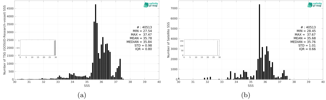
Figure 3: Histograms of SSS from TSG (GOSUD-Research-vessel) (a) and Aquarius SSS L3 OR v5 - Monthly (NASA-GSFC) (b) considering all match-up pairs per bins of 0.1 over the South Atlantic Ocean Pi-MEP region and for the full satellite product period.
