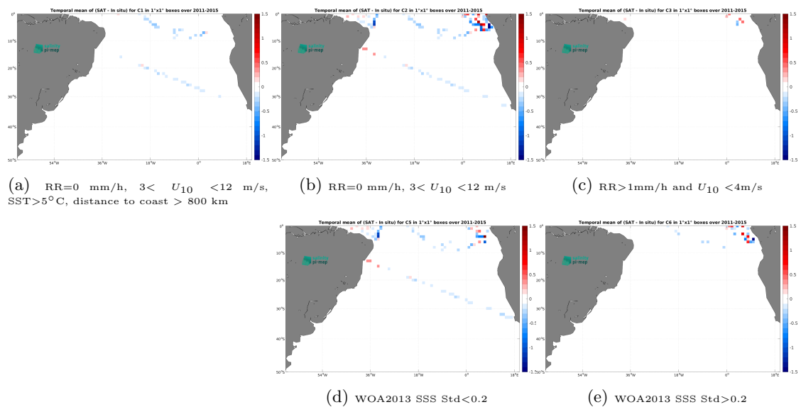
Figure 14: Temporal mean gridded over spatial boxes of size 1^\circ \times 1^\circ of \Delta SSS (Aquarius SSS L3 OR v5 - Monthly (NASA-GSFC) - TSG (GOSUD-Research-vessel)) for 5 different subdatasets corresponding to:RR=0 mm/h, 3 < U_{10} < 12 m/s, SST >5^\circ\text{C} , distance to coast > 800 km (a), RR=0 mm/h, 3 < U_{10} < 12 m/s (b), RR >1 mm/h and U_{10} < 4 m/s (c), WOA2013 SSS Std <0.2 (d), WOA2013 SSS Std >0.2 (e).
