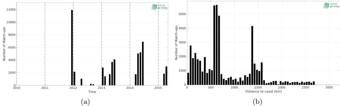
Figure 1: Number of match-ups between TSG (GOSUD-Research-vessel) and Aquarius SSS L3 OR v5 - Monthly (NASA-GSFC) SSS as a function of time (a) and as function of the distance to coast (b) over the South Atlantic Ocean Pi-MEP region and for the full satellite product period.
