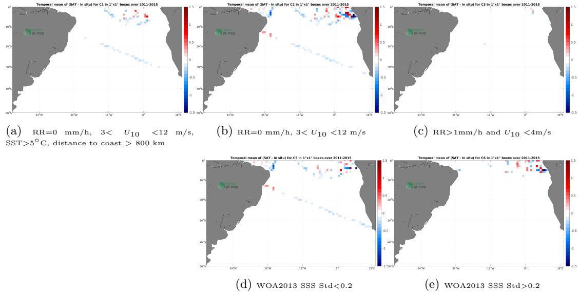
Figure 12: Temporal mean gridded over spatial boxes of size 1^{\circ}\times 1^{\circ} of \Delta SSS (Aquarius SSS L3 OR v5 - Monthly (NASA-GSFC) - TSG (GOSUD-Research-vessel)) for 5 different subdatasets corresponding to:RR=0 mm/h, 3 < U_{10} < 12 m/s, SST >5^{\circ}\text{C} , distance to coast > 800 km (a), RR=0 mm/h, 3 < U_{10} < 12 m/s (b), RR >1 mm/h and U_{10} < 4 m/s (c), WOA2013 SSS Std <0.2 (d), WOA2013 SSS Std >0.2 (e).
