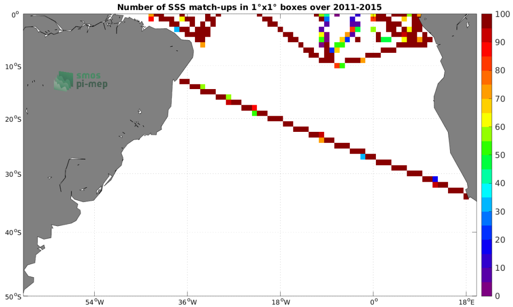
Figure 4: Number of SSS match-ups between TSG (GOSUD-Research-vessel) SSS and the Aquarius SSS L3 OR v5 - Monthly (NASA-GSFC) SSS product for the South Atlantic Ocean Pi-MEP region over 1^\circ \times 1^\circ boxes and for the full satellite product period.
