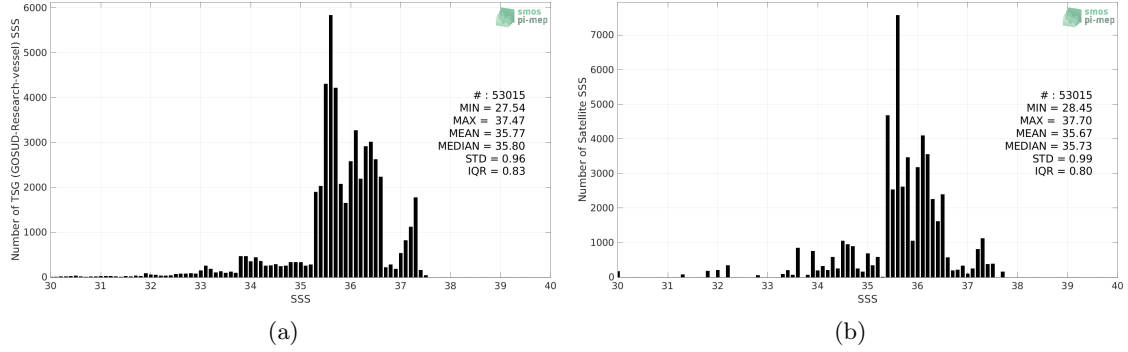
Figure 2: Histograms of SSS from TSG (GOSUD-Research-vessel) (a) and Aquarius SSS L3 OR v5 - Monthly (NASA-GSFC) (b) considering all match-up pairs per bins of 0.1 over the South Atlantic Ocean Pi-MEP region and for the full satellite product period.
