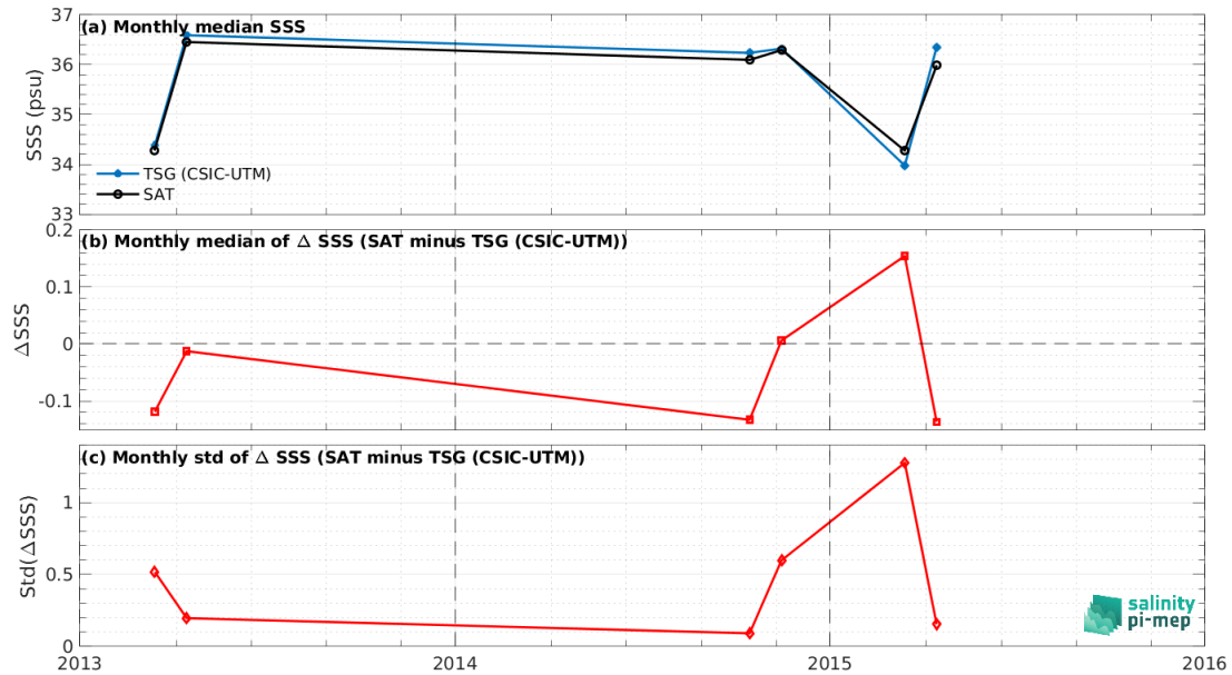
Figure 8: Time series of the monthly median SSS (top), median of \Delta\text{SSS} (Satellite - TSG (CSIC-UTM)) and Std of \Delta\text{SSS} (Satellite - TSG (CSIC-UTM)) over the South Atlantic Ocean Pi-MEP region considering all match-ups collected by the Pi-MEP.
