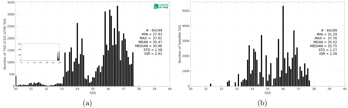
Figure 3: Histograms of SSS from TSG (CSIC-UTM) (a) and Aquarius SSS L3 OR v5 - Monthly (NASA-GSFC) (b) considering all match-up pairs per bins of 0.1 over the South Atlantic Ocean Pi-MEP region and for the full satellite product period.
