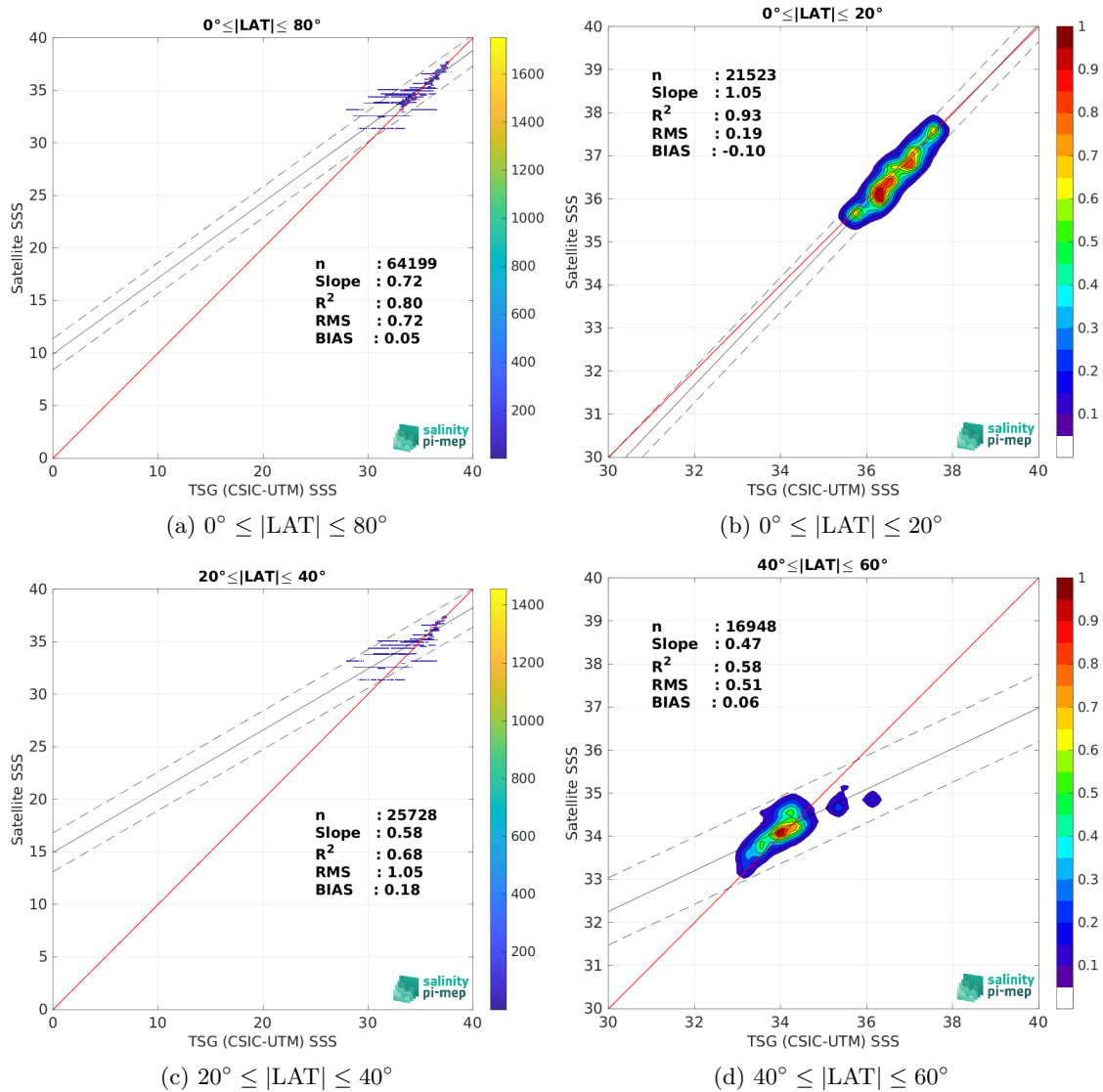
Figure 10: Contour maps of the concentration of Aquarius SSS L3 OR v5 - Monthly (NASA-GSFC) SSS ( y -axis) versus TSG (CSIC-UTM) SSS ( x -axis) at match-up pairs for different latitude bands. For each plot, the red line shows x=y . The black thin and dashed lines indicate a linear fit through the data cloud and the \pm 95\% confidence levels, respectively. The number match-up pairs n , the slope and R^2 coefficient of the linear fit, the root mean square (RMS) and the mean bias between satellite and in situ data are indicated for each latitude band in each plots.
