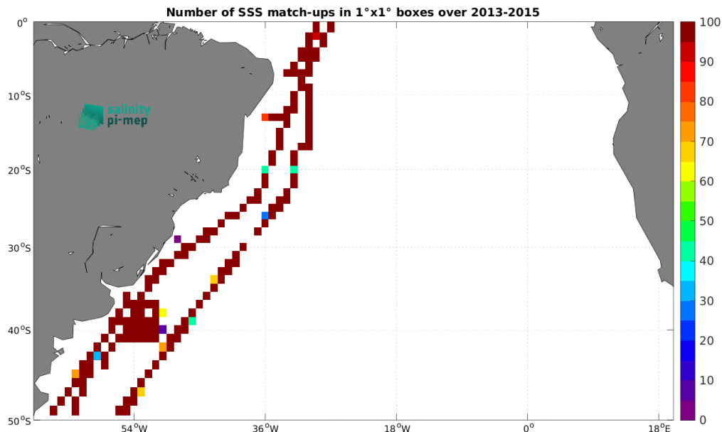
Figure 5: Number of SSS match-ups between TSG (CSIC-UTM) SSS and the Aquarius SSS L3 OR v5 - Monthly (NASA-GSFC) SSS product for the South Atlantic Ocean Pi-MEP region over 1^\circ \times 1^\circ boxes and for the full satellite product period.
