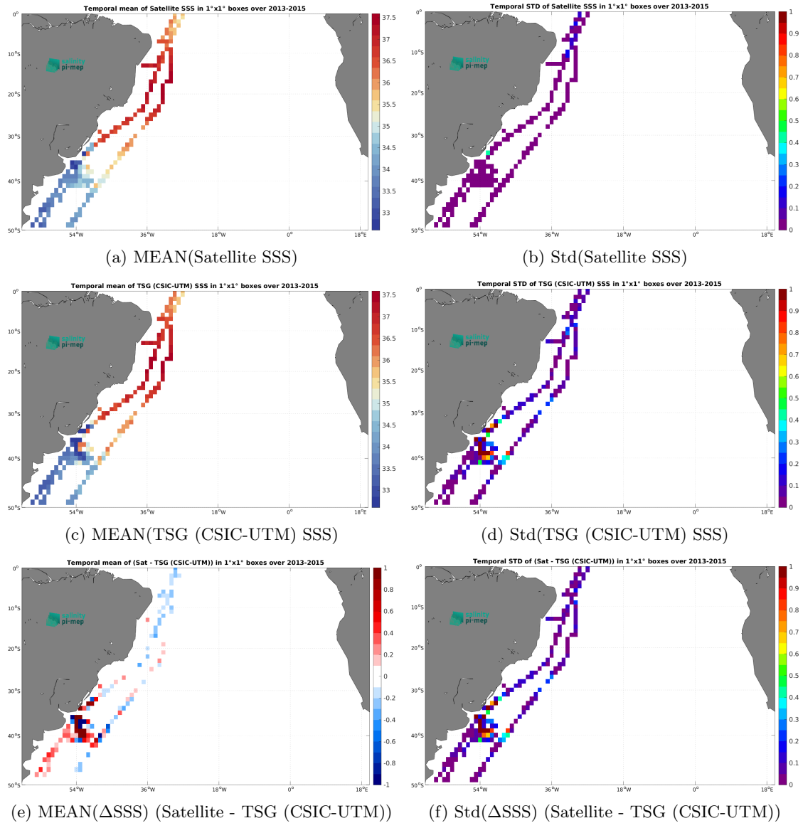
Figure 6: Temporal mean (left) and Std (right) of SSS from Aquarius SSS L3 OR v5 - Monthly (NASA-GSFC) (top), TSG (CSIC-UTM) ( in situ ) dataset (middle), and of \Delta SSS (Satellite - TSG (CSIC-UTM)). Only match-up pairs are used to generate these maps.
