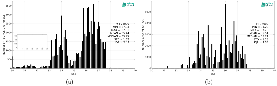
Figure 2: Histograms of SSS from TSG (CSIC-UTM) (a) and Aquarius SSS L3 OR v5 - Monthly (NASA-GSFC) (b) considering all match-up pairs per bins of 0.1 over the South Atlantic Ocean Pi-MEP region and for the full satellite product period.
