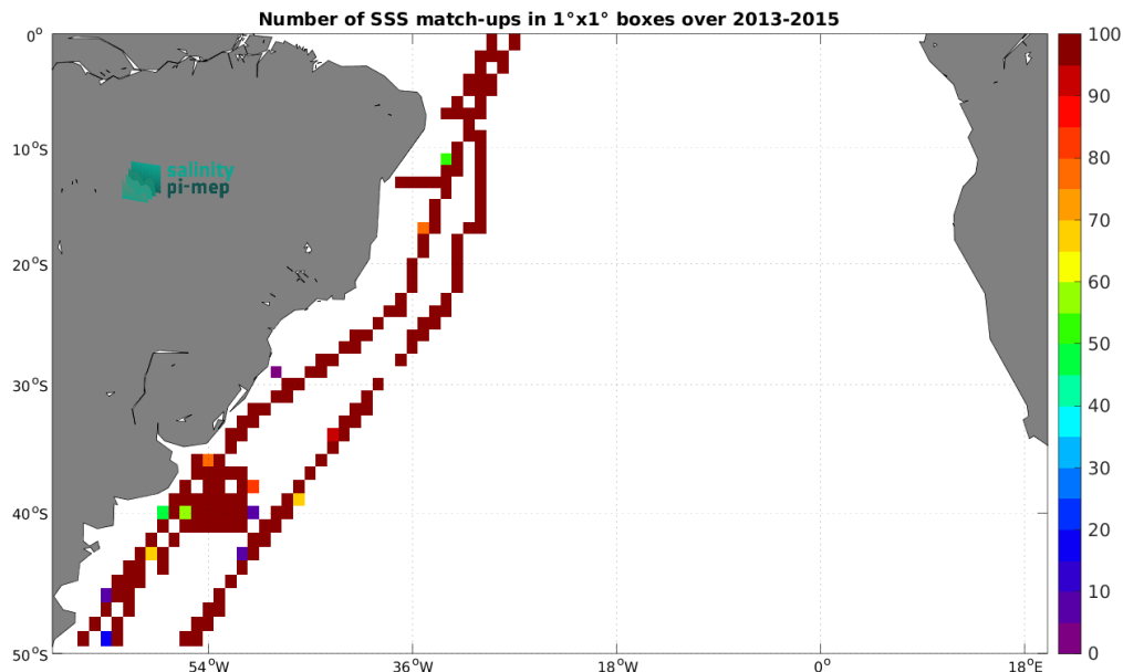
Figure 4: Number of SSS match-ups between TSG (CSIC-UTM) SSS and the Aquarius SSS L3 OR v5 - Monthly (NASA-GSFC) SSS product for the South Atlantic Ocean Pi-MEP region over 1^\circ \times 1^\circ boxes and for the full satellite product period.
