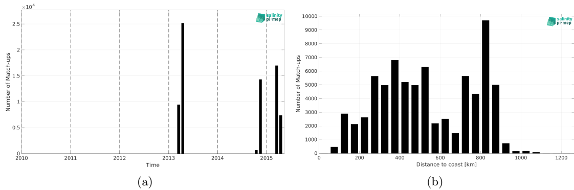
Figure 1: Number of match-ups between TSG (CSIC-UTM) and Aquarius SSS L3 OR v5 - Monthly (NASA-GSFC) SSS as a function of time (a) and as function of the distance to coast (b) over the South Atlantic Ocean Pi-MEP region and for the full satellite product period.
