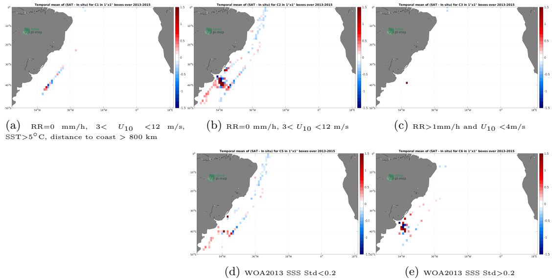
Figure 12: Temporal mean gridded over spatial boxes of size 1^\circ \times 1^\circ of \Delta SSS (Aquarius SSS L3 OR v5 - Monthly (NASA-GSFC) - TSG (CSIC-UTM)) for 5 different subdatasets corresponding to: RR=0 mm/h, 3 < U_{10} < 12 m/s, SST > 5^\circ C , distance to coast > 800 km (a), RR=0 mm/h, 3 < U_{10} < 12 m/s (b), RR > 1 mm/h and U_{10} < 4 m/s (c), WOA2013 SSS Std < 0.2 (d), WOA2013 SSS Std > 0.2 (e).
