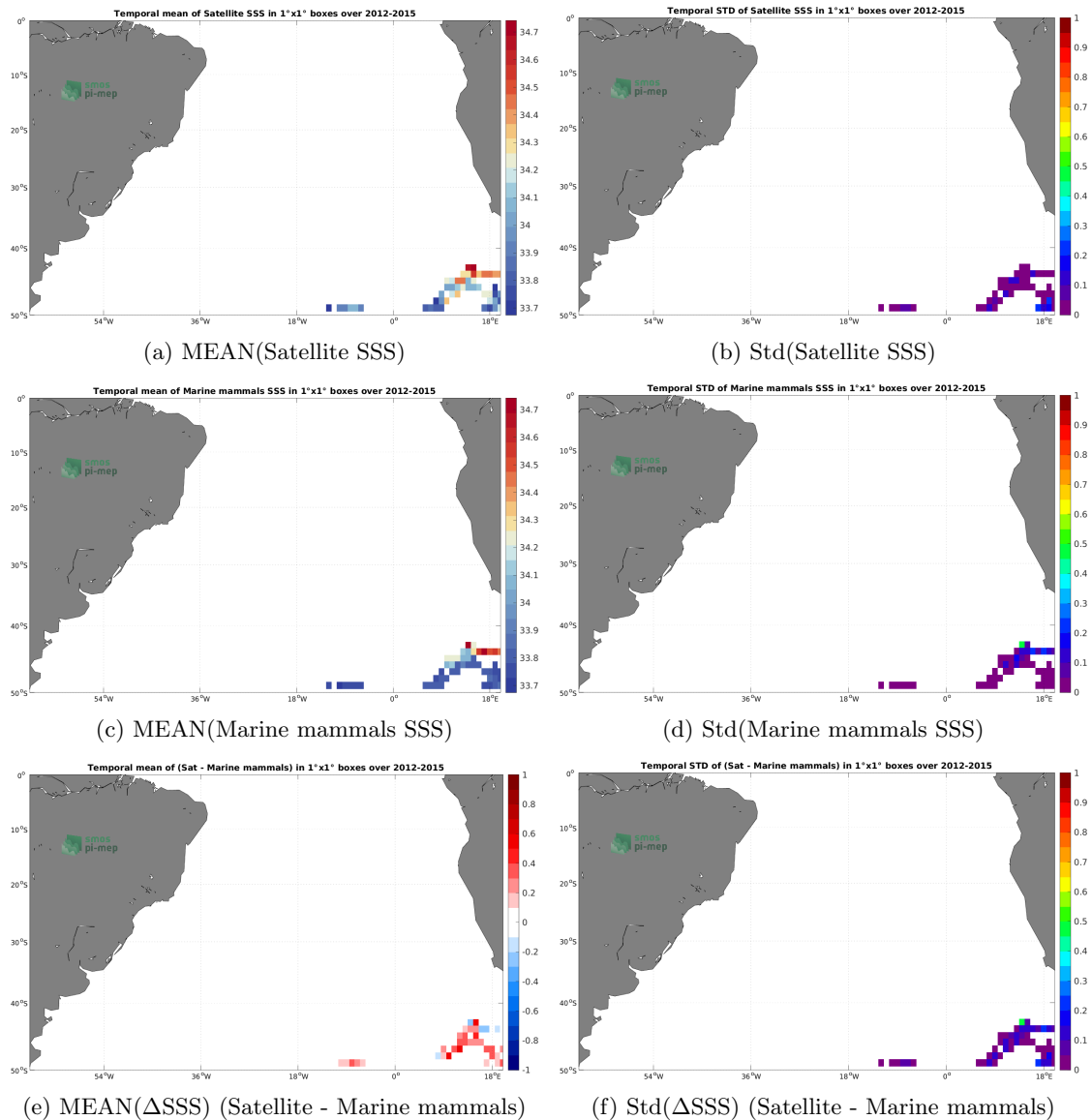
Figure 6: Temporal mean (left) and Std (right) of SSS from Aquarius SSS L3 OR v5 - Monthly (NASA-GSFC) (top), Marine mammals (middle), and of \Delta SSS (Satellite - Marine mammals). Only match-up pairs are used to generate these maps.
