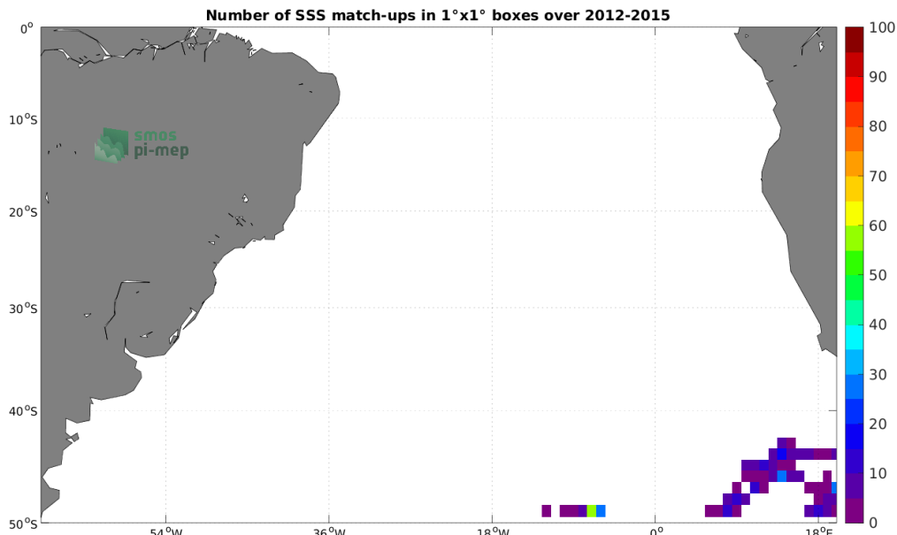
Figure 4: Number of SSS match-ups between Marine mammals SSS and the Aquarius SSS L3 OR v5 - Monthly (NASA-GSFC) SSS product for the South Atlantic Ocean Pi-MEP region over 1^\circ \times 1^\circ boxes and for the full satellite product period.
