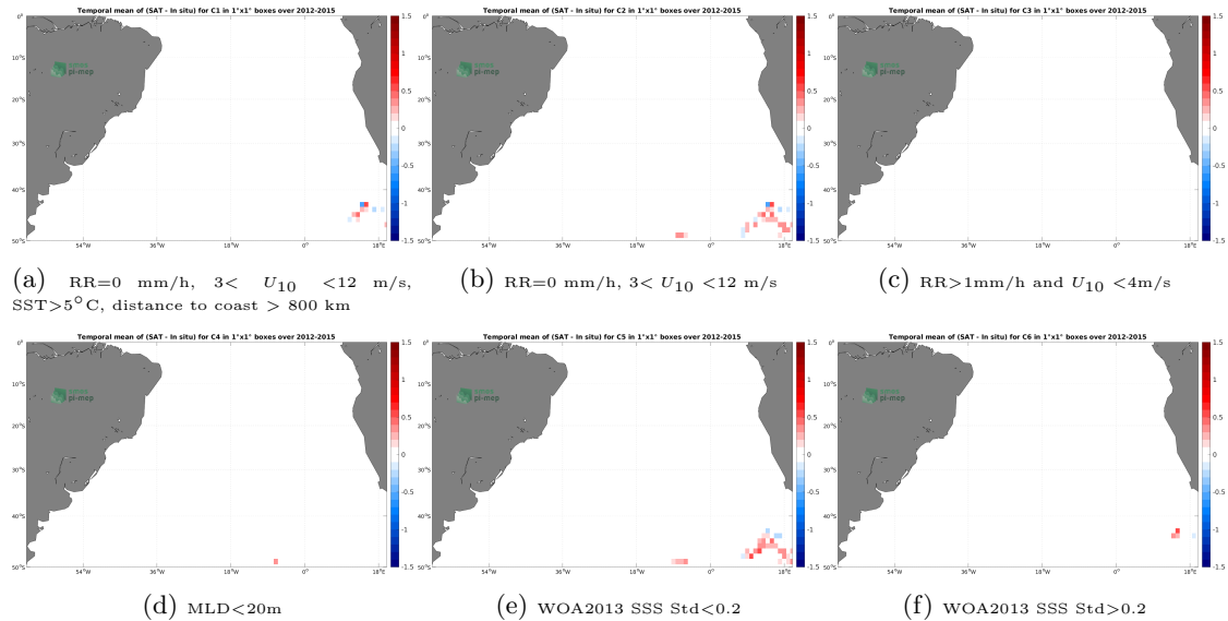
Figure 12: Temporal mean gridded over spatial boxes of size 1^{\circ}\times 1^{\circ} of \Delta\text{SSS} (Aquarius SSS L3 OR v5 - Monthly (NASA-GSFC) - Marine mammals) for 6 different subdatasets corresponding to:RR=0 mm/h, 3 < U_{10} < 12 m/s, SST >5^{\circ}\text{C} , distance to coast > 800 km (a), RR=0 mm/h, 3 < U_{10} < 12 m/s (b), RR >1 mm/h and U_{10} < 4 m/s (c),MLD <20 m (d),WOA2013 SSS Std <0.2 (e),WOA2013 SSS Std >0.2 (f).
