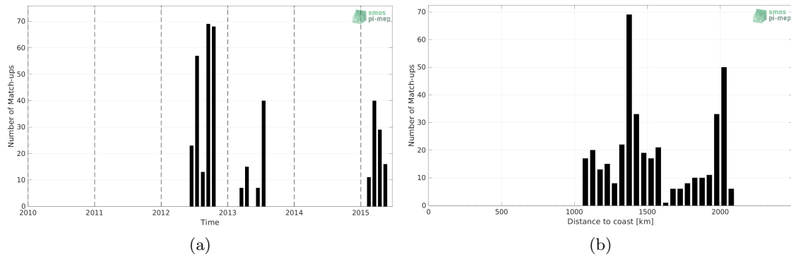
Figure 1: Number of match-ups between Marine mammals and Aquarius SSS L3 OR v5 - Monthly (NASA-GSFC) SSS as a function of time (a) and as function of the distance to coast (b) over the South Atlantic Ocean Pi-MEP region and for the full satellite product period.
