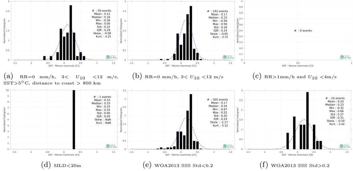
Figure 13: Normalized histogram of \Delta SSS (Aquarius SSS L3 OR v5 - Monthly (NASA-GSFC) - Marine mammals) for 6 different subdatasets corresponding to: RR=0 mm/h, 3 < U_{10} < 12 m/s, SST>5°C, distance to coast > 800 km (a), RR=0 mm/h, 3 < U_{10} < 12 m/s (b), RR>1mm/h and U_{10} < 4 m/s (c), MLD<20m (d), WOA2013 SSS Std<0.2 (e), WOA2013 SSS Std>0.2 (f).
