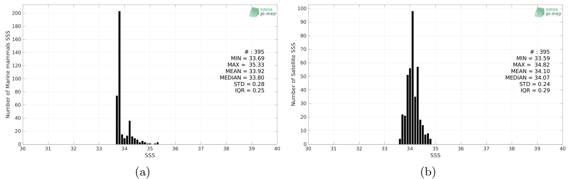
Figure 2: Histograms of SSS from Marine mammals (a) and Aquarius SSS L3 OR v5 - Monthly (NASA-GSFC) (b) considering all match-up pairs per bins of 0.1 over the South Atlantic Ocean Pi-MEP region and for the full satellite product period.
