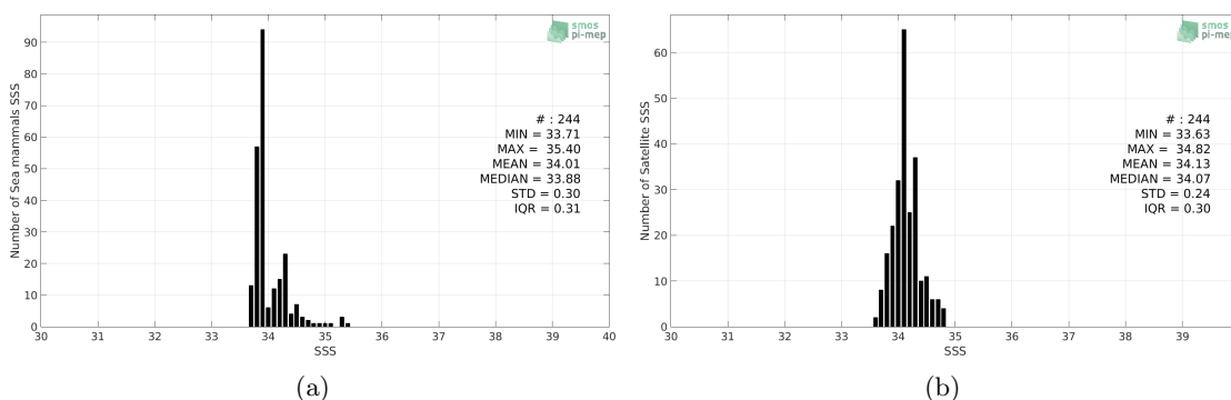
Figure 2: Histograms of SSS from Sea mammals (a) and Aquarius-L3-OR-V5-MONTHLY-1DEG (b) considering all match-up pairs per bins of 0.1 over the South Atlantic Ocean Pi-MEP region and for the full satellite product period.
