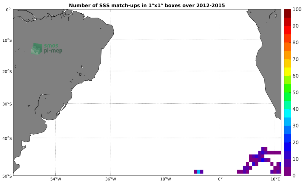
Figure 4: Number of SSS match-ups between Sea mammals SSS and the Aquarius-L3-OR-V5-MONTHLY-1DEG SSS product for the South Atlantic Ocean Pi-MEP region over 1^\circ \times 1^\circ boxes and for the full satellite product period.
