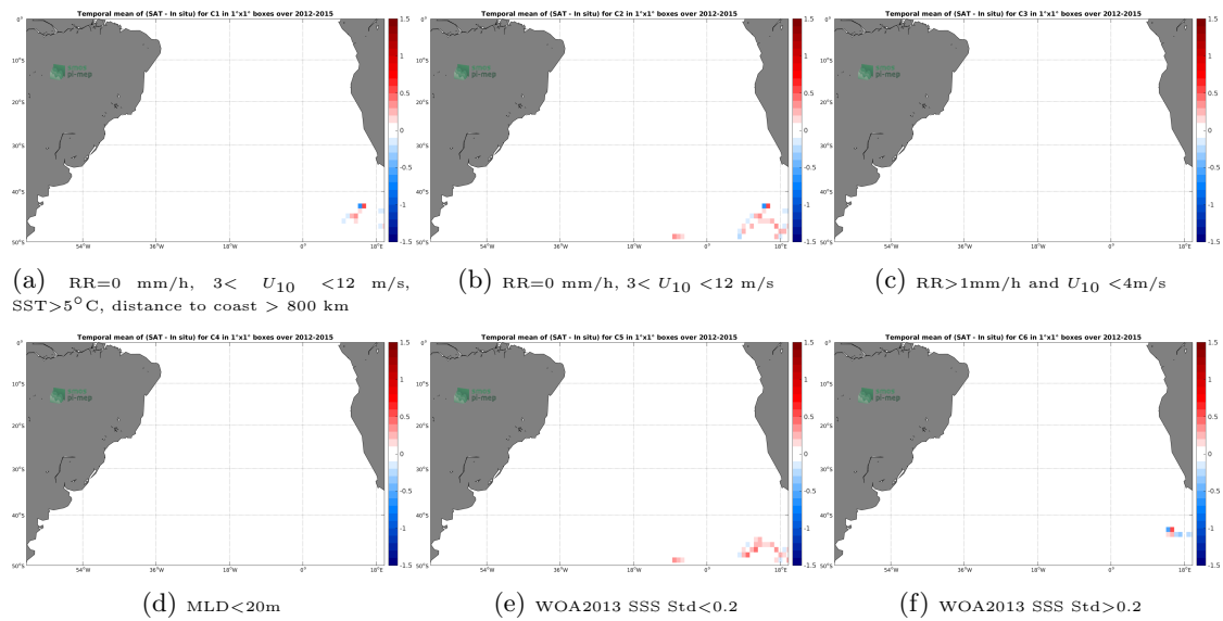
Figure 12: Temporal mean gridded over spatial boxes of size 1^\circ \times 1^\circ of \Delta SSS (Aquarius-L3-OR-V5-MONTHLY-1DEG - Sea mammals) for 6 different subdatasets corresponding to:RR=0 mm/h, 3 < U_{10} < 12 m/s, SST >5^\circ C, distance to coast > 800 km (a), RR=0 mm/h, 3 < U_{10} < 12 m/s (b), RR >1 mm/h and U_{10} < 4 m/s (c),MLD <20 m (d),WOA2013 SSS Std <0.2 (e),WOA2013 SSS Std >0.2 (f).
