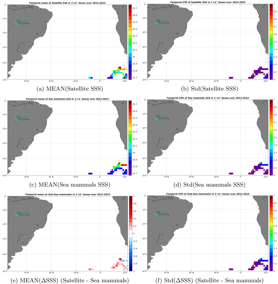
Figure 6: Temporal mean (left) and Std (right) of SSS from Aquarius-L3-OR-V5-MONTHLY-1DEG (top), Sea mammals (middle), and of \Delta SSS (Satellite - Sea mammals). Only match-up pairs are used to generate these maps.
