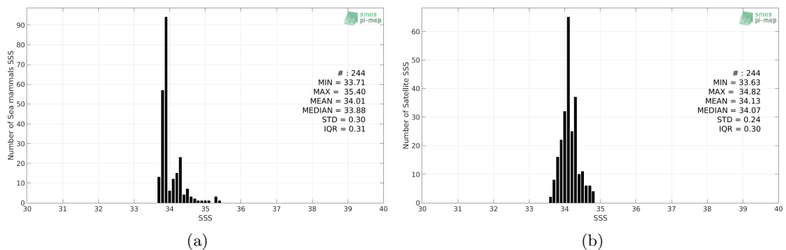
Figure 2: Histograms of SSS from Sea mammals (a) and Aquarius-L3-OR-V5-MONTHLY-1DEG (b) considering all match-up pairs per bins of 0.1 over the South Atlantic Ocean Pi-MEP region and for the full satellite product period.
