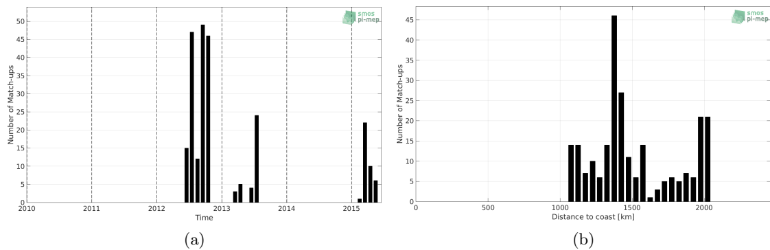
Figure 1: Number of match-ups between Sea mammals and Aquarius-L3-OR-V5-MONTHLY-1DEG SSS as a function of time (a) and as function of the distance to coast (b) over the South Atlantic Ocean Pi-MEP region and for the full satellite product period.
