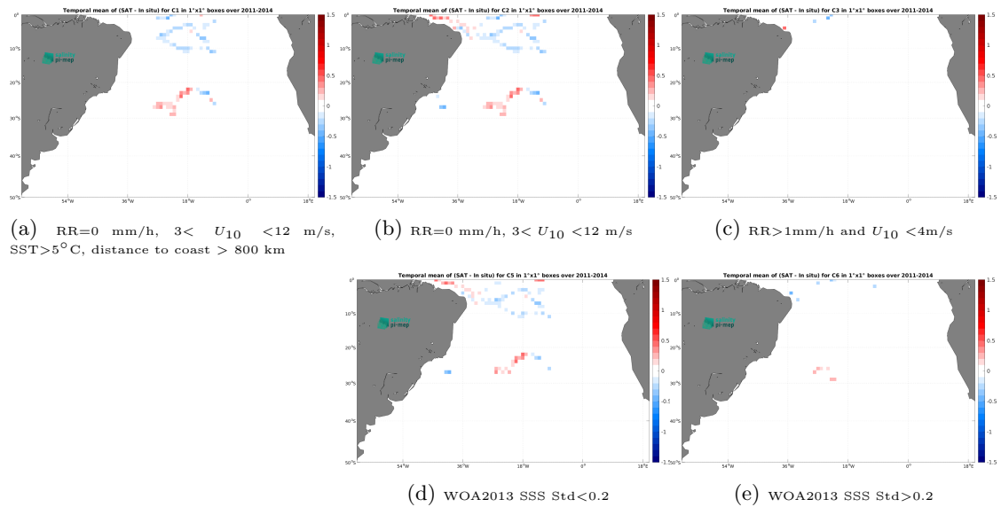
Figure 11: Temporal mean gridded over spatial boxes of size 1^\circ \times 1^\circ of \Delta\text{SSS} (Aquarius SSS L3 OR v5 - Monthly (NASA-GSFC) - Surface drifters) for 5 different subdatasets corresponding to:RR=0 mm/h, 3 < U_{10} < 12 m/s, SST >5^\circ\text{C} , distance to coast > 800 km (a), RR=0 mm/h, 3 < U_{10} < 12 m/s (b), RR >1 mm/h and U_{10} < 4 m/s (c), WOA2013 SSS Std <0.2 (d), WOA2013 SSS Std >0.2 (e).
