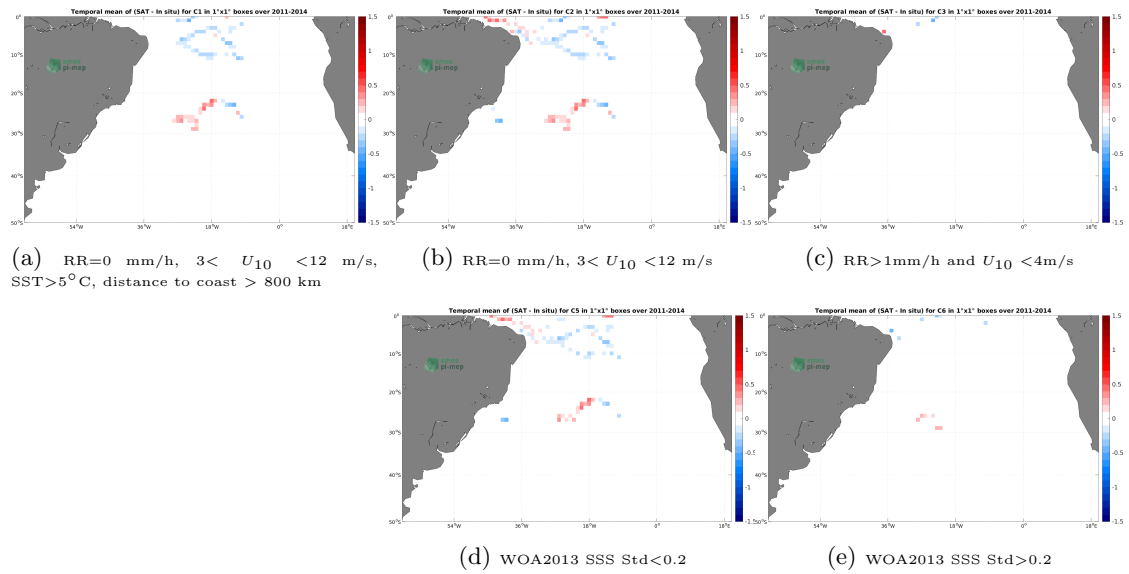
Figure 11: Temporal mean gridded over spatial boxes of size 1^\circ \times 1^\circ of \Delta SSS (Aquarius SSS L3 OR v5 - Monthly (NASA-GSFC) - Surface drifters) for 5 different subdatasets corresponding to:RR=0 mm/h, 3 < U_{10} < 12 m/s, SST >5^\circ\text{C} , distance to coast > 800 km (a), RR=0 mm/h, 3 < U_{10} < 12 m/s (b), RR >1 mm/h and U_{10} < 4 m/s (c), WOA2013 SSS Std <0.2 (d), WOA2013 SSS Std >0.2 (e).
