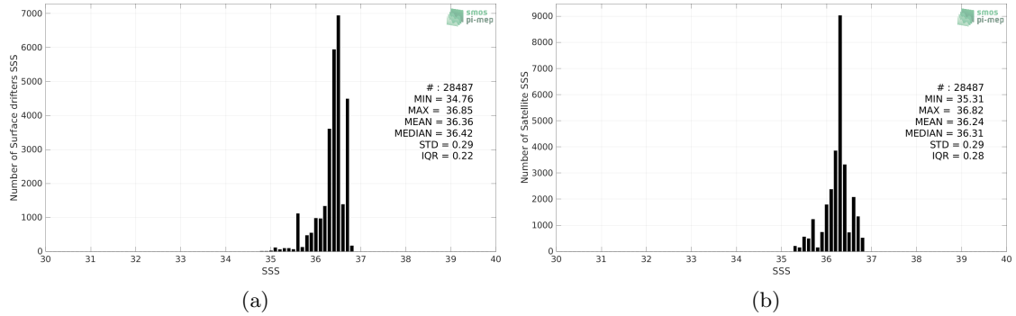
Figure 2: Histograms of SSS from Surface drifters (a) and Aquarius SSS L3 OR v5 - Monthly (NASA-GSFC) (b) considering all match-up pairs per bins of 0.1 over the South Atlantic Ocean Pi-MEP region and for the full satellite product period.
