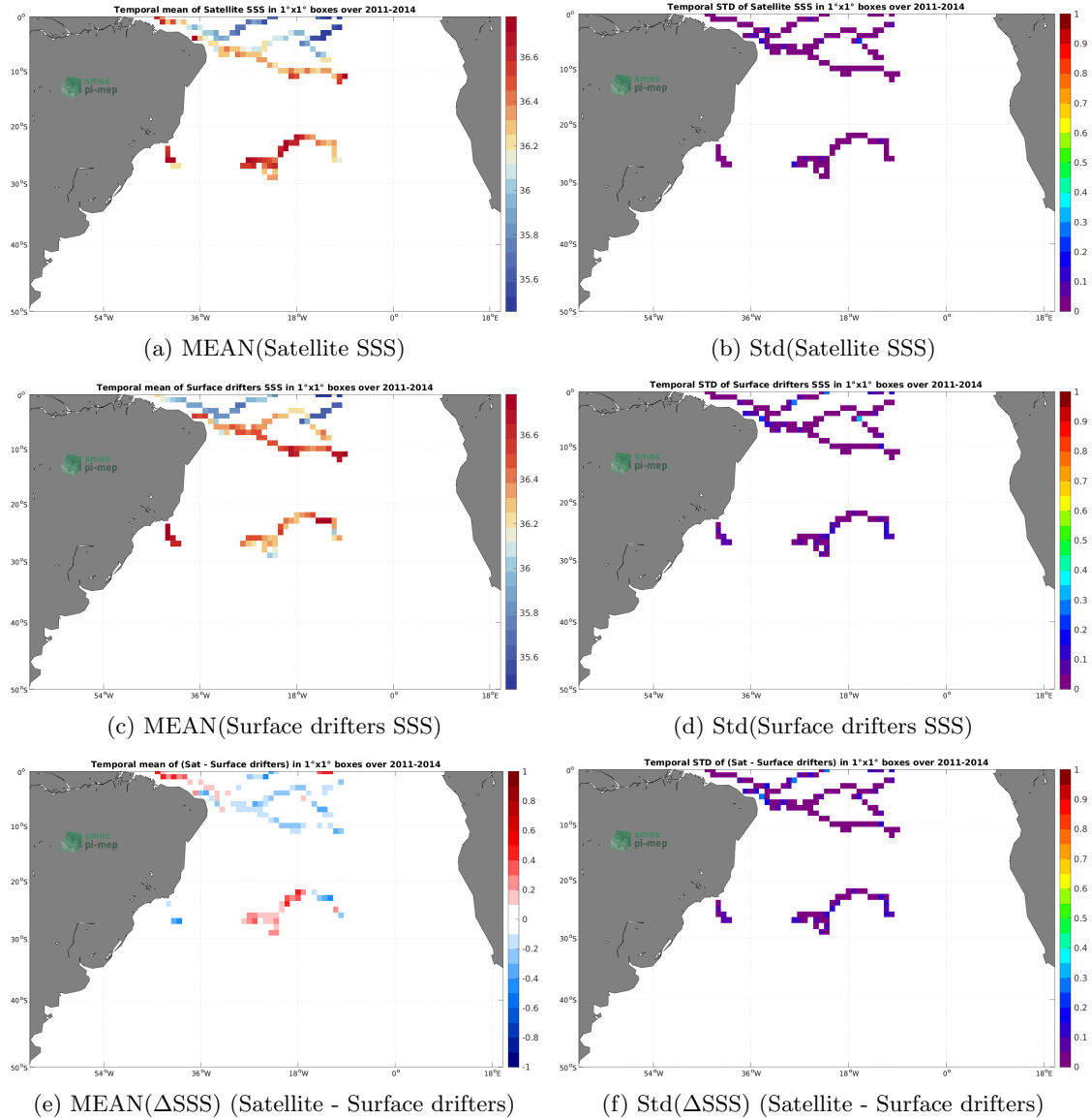
Figure 5: Temporal mean (left) and Std (right) of SSS from Aquarius SSS L3 OR v5 - Monthly (NASA-GSFC) (top), Surface drifters (middle), and of \Delta SSS (Satellite - Surface drifters). Only match-up pairs are used to generate these maps.
