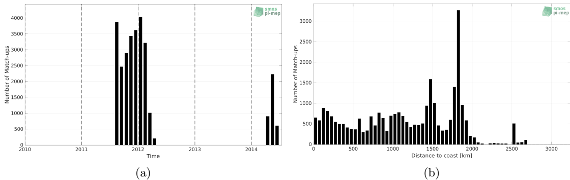
Figure 1: Number of match-ups between Surface drifters and Aquarius SSS L3 OR v5 - Monthly (NASA-GSFC) SSS as a function of time (a) and as function of the distance to coast (b) over the South Atlantic Ocean Pi-MEP region and for the full satellite product period.
