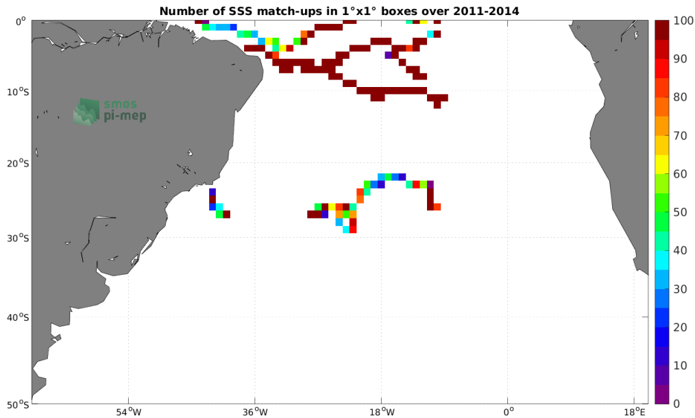
Figure 3: Number of SSS match-ups between Surface drifters SSS and the Aquarius SSS L3 OR v5 - Monthly (NASA-GSFC) SSS product for the South Atlantic Ocean Pi-MEP region over 1^\circ \times 1^\circ boxes and for the full satellite product period.
