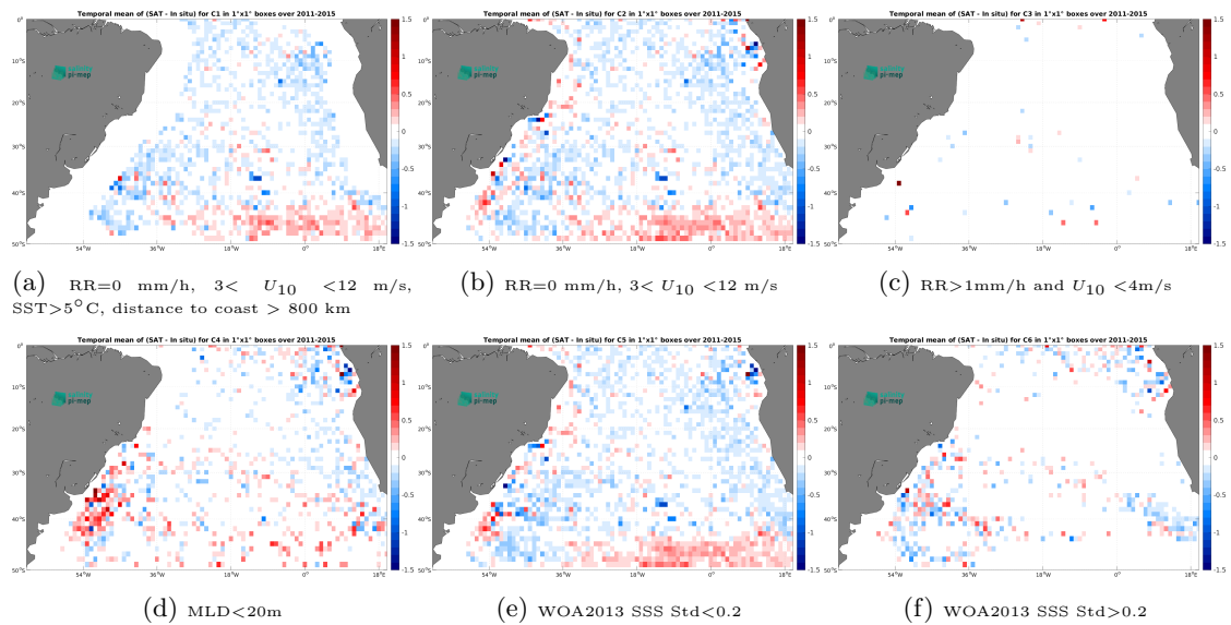
Figure 14: Temporal mean gridded over spatial boxes of size 1^\circ \times 1^\circ of \Delta\text{SSS} (Aquarius SSS L3 OR v5 - Monthly (NASA-GSFC) - Argo) for 6 different subdatasets corresponding to: RR=0 mm/h, 3 < U_{10} < 12 m/s, SST > 5°C, distance to coast > 800 km (a), RR=0 mm/h, 3 < U_{10} < 12 m/s (b), RR > 1mm/h and U_{10} < 4 m/s (c), MLD < 20m (d), WOA2013 SSS Std < 0.2 (e), WOA2013 SSS Std > 0.2 (f).
