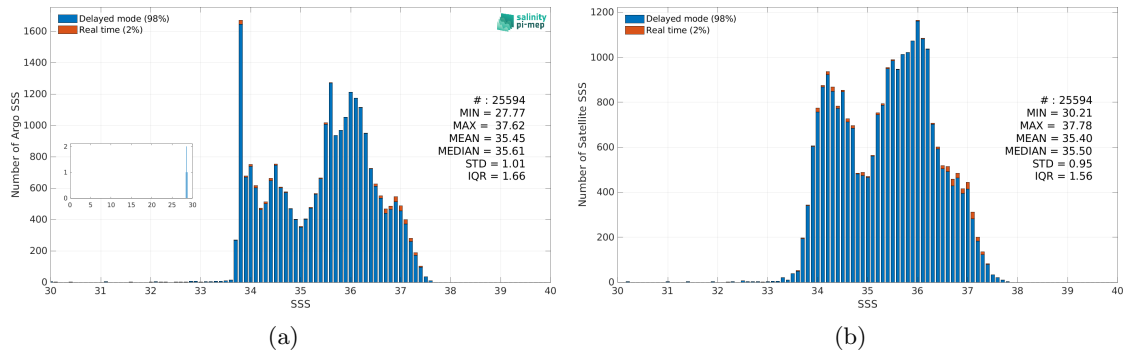
Figure 3: Histograms of SSS from Argo (a) and Aquarius SSS L3 OR v5 - Monthly (NASA-GSFC) (b) considering all match-up pairs per bins of 0.1 over the South Atlantic Ocean Pi-MEP region and for the full satellite product period.
