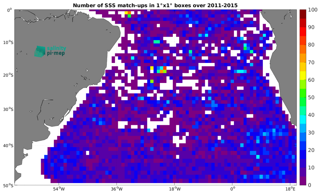
Figure 5: Number of SSS match-ups between Argo SSS and the Aquarius SSS L3 OR v5 - Monthly (NASA-GSFC) SSS product for the South Atlantic Ocean Pi-MEP region over 1^\circ \times 1^\circ boxes and for the full satellite product period.
