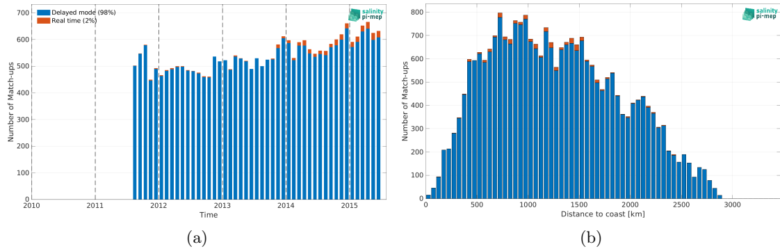
Figure 2: Number of match-ups between Argo and Aquarius SSS L3 OR v5 - Monthly (NASA-GSFC) SSS as a function of time (a) and as function of the distance to coast (b) over the South Atlantic Ocean Pi-MEP region and for the full satellite product period.
