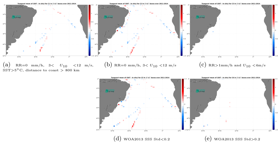
Figure 14: Temporal mean gridded over spatial boxes of size 1^\circ \times 1^\circ of \Delta\text{SSS} (Aquarius SSS L3 OR v5 - Monthly - Rain mask (NASA-GSFC) - TSG (SAMOS)) for 5 different subdatasets corresponding to:RR=0 mm/h, 3 < U_{10} < 12 m/s, SST>5°C, distance to coast > 800 km (a), RR=0 mm/h, 3 < U_{10} < 12 m/s (b), RR>1mm/h and U_{10} < 4 m/s (c), WOA2013 SSS Std<0.2 (d), WOA2013 SSS Std>0.2 (e).
