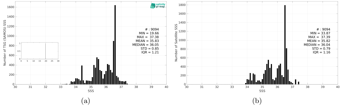
Figure 3: Histograms of SSS from TSG (SAMOS) (a) and Aquarius SSS L3 OR v5 - Monthly - Rain mask (NASA-GSFC) (b) considering all match-up pairs per bins of 0.1 over the South Atlantic Ocean Pi-MEP region and for the full satellite product period.
