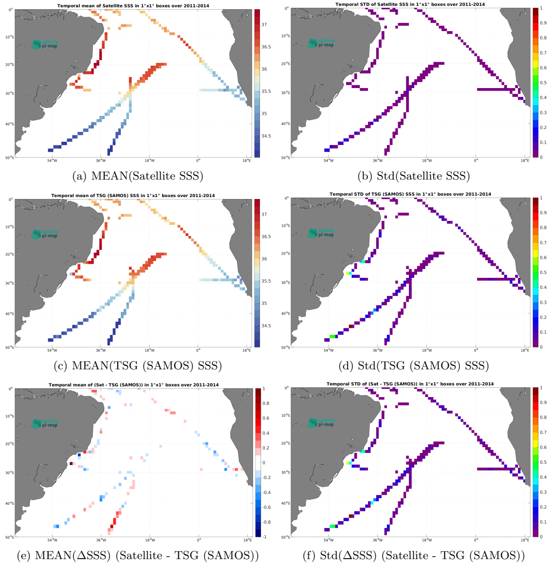
Figure 7: Temporal mean (left) and Std (right) of SSS from Aquarius SSS L3 OR v5 - Monthly - Rain mask (NASA-GSFC) (top), TSG (SAMOS) (middle), and of \Delta SSS (Satellite - TSG (SAMOS)). Only match-up pairs are used to generate these maps.
