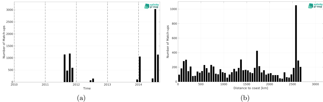
Figure 2: Number of match-ups between TSG (SAMOS) and Aquarius SSS L3 OR v5 - Monthly - Rain mask (NASA-GSFC) SSS as a function of time (a) and as function of the distance to coast (b) over the South Atlantic Ocean Pi-MEP region and for the full satellite product period.
