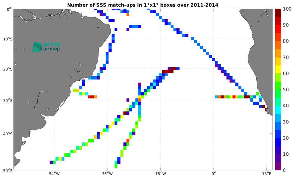
Figure 5: Number of SSS match-ups between TSG (SAMOS) SSS and the Aquarius SSS L3 OR v5 - Monthly - Rain mask (NASA-GSFC) SSS product for the South Atlantic Ocean Pi-MEP region over 1^\circ \times 1^\circ boxes and for the full satellite product period.
