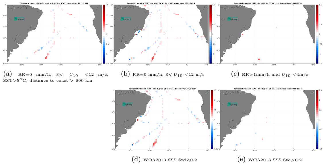
Figure 12: Temporal mean gridded over spatial boxes of size 1^\circ \times 1^\circ of \Delta\text{SSS} (Aquarius SSS L3 OR v5 - Monthly - Rain mask (NASA-GSFC) - TSG (SAMOS)) for 5 different subdatasets corresponding to:RR=0 mm/h, 3 < U_{10} < 12 m/s, SST >5^\circ\text{C} , distance to coast > 800 km (a), RR=0 mm/h, 3 < U_{10} < 12 m/s (b), RR >1 mm/h and U_{10} < 4 m/s (c), WOA2013 SSS Std <0.2 (d), WOA2013 SSS Std >0.2 (e).
