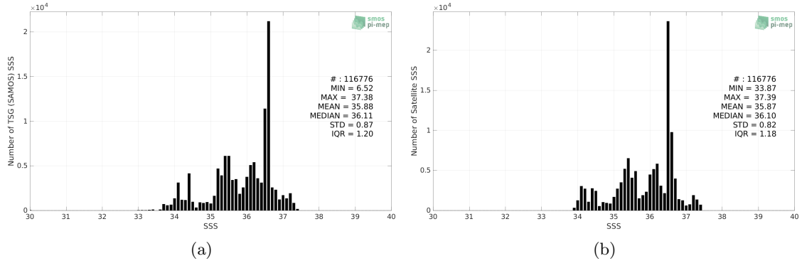
Figure 2: Histograms of SSS from TSG (SAMOS) (a) and Aquarius SSS L3 OR v5 - Monthly - Rain mask (NASA-GSFC) (b) considering all match-up pairs per bins of 0.1 over the South Atlantic Ocean Pi-MEP region and for the full satellite product period.
