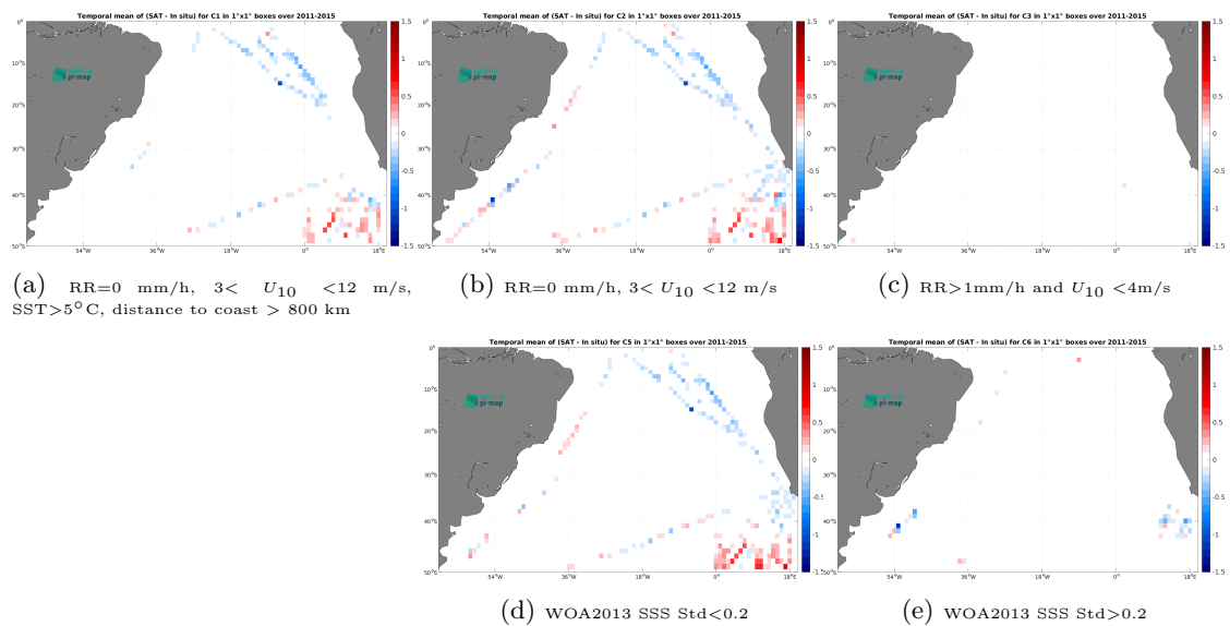
Figure 14: Temporal mean gridded over spatial boxes of size 1^\circ \times 1^\circ of \Delta\text{SSS} (Aquarius SSS L3 OR v5 - Monthly - Rain mask (NASA-GSFC) - TSG (Polarstern)) for 5 different subdatasets corresponding to:RR=0 mm/h, 3 < U_{10} < 12 m/s, SST >5^\circ\text{C} , distance to coast > 800 km (a), RR=0 mm/h, 3 < U_{10} < 12 m/s (b), RR >1 mm/h and U_{10} < 4 m/s (c), WOA2013 SSS Std <0.2 (d), WOA2013 SSS Std >0.2 (e).
