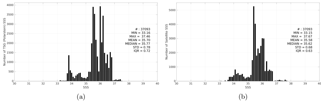
Figure 3: Histograms of SSS from TSG (Polarstern) (a) and Aquarius SSS L3 OR v5 - Monthly - Rain mask (NASA-GSFC) (b) considering all match-up pairs per bins of 0.1 over the South Atlantic Ocean Pi-MEP region and for the full satellite product period.
