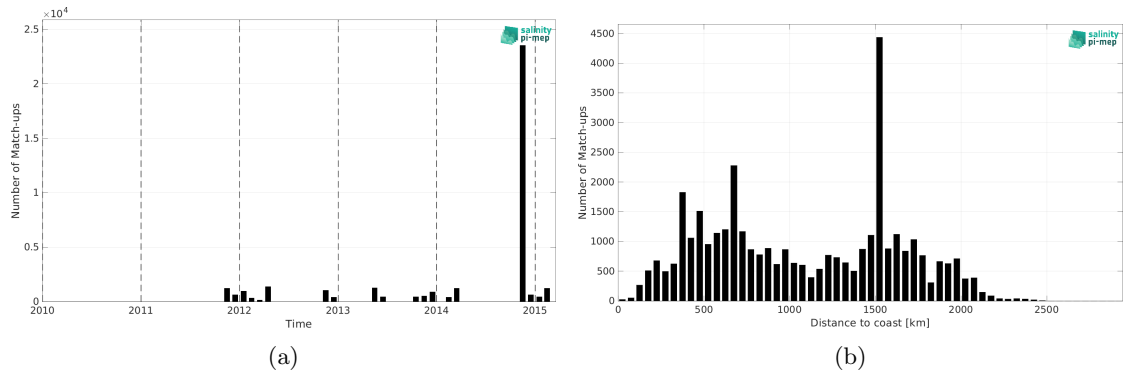
Figure 2: Number of match-ups between TSG (Polarstern) and Aquarius SSS L3 OR v5 - Monthly - Rain mask (NASA-GSFC) SSS as a function of time (a) and as function of the distance to coast (b) over the South Atlantic Ocean Pi-MEP region and for the full satellite product period.
