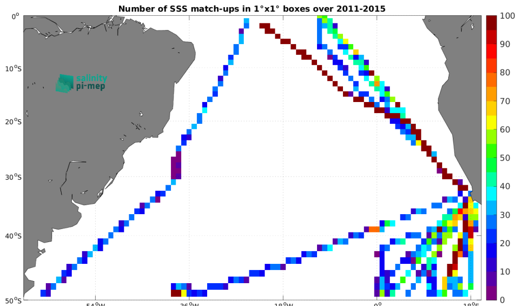
Figure 5: Number of SSS match-ups between TSG (Polarstern) SSS and the Aquarius SSS L3 OR v5 - Monthly - Rain mask (NASA-GSFC) SSS product for the South Atlantic Ocean Pi-MEP region over 1^\circ \times 1^\circ boxes and for the full satellite product period.
