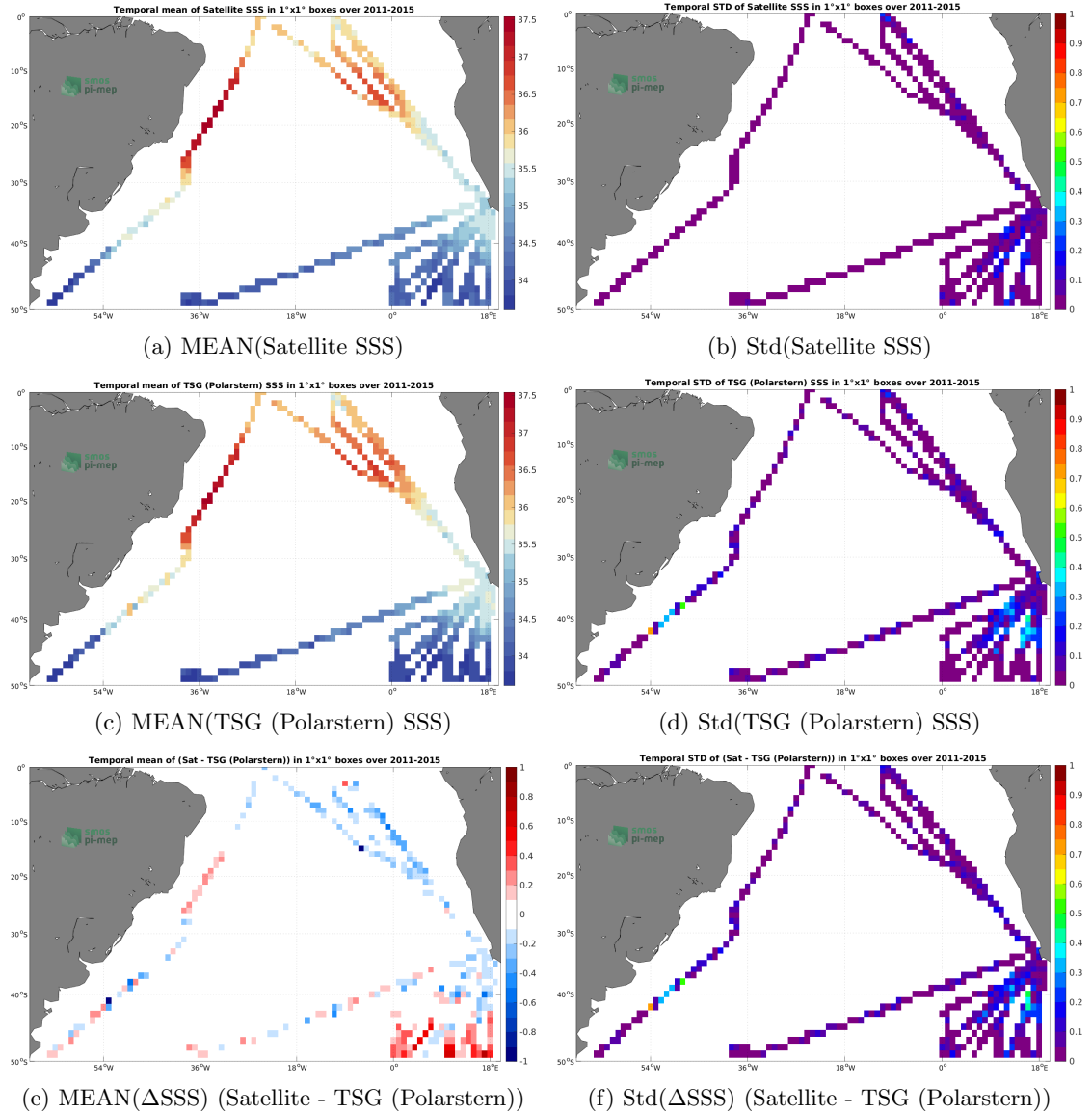
Figure 6: Temporal mean (left) and Std (right) of SSS from Aquarius SSS L3 OR v5 - Monthly - Rain mask (NASA-GSFC) (top), TSG (Polarstern) (middle), and of \Delta SSS (Satellite - TSG (Polarstern)). Only match-up pairs are used to generate these maps.
