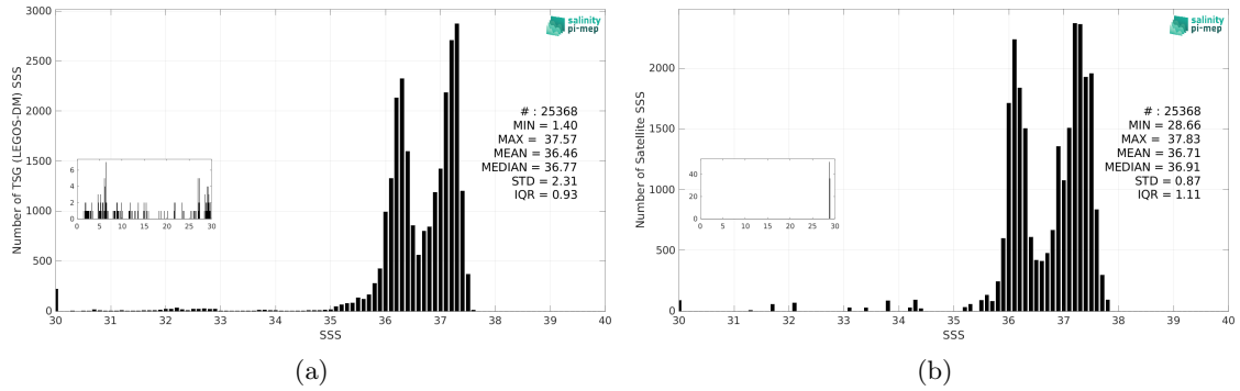
Figure 3: Histograms of SSS from TSG (LEGOS-DM) (a) and Aquarius SSS L3 OR v5 - Monthly - Rain mask (NASA-GSFC) (b) considering all match-up pairs per bins of 0.1 over the South Atlantic Ocean Pi-MEP region and for the full satellite product period.
