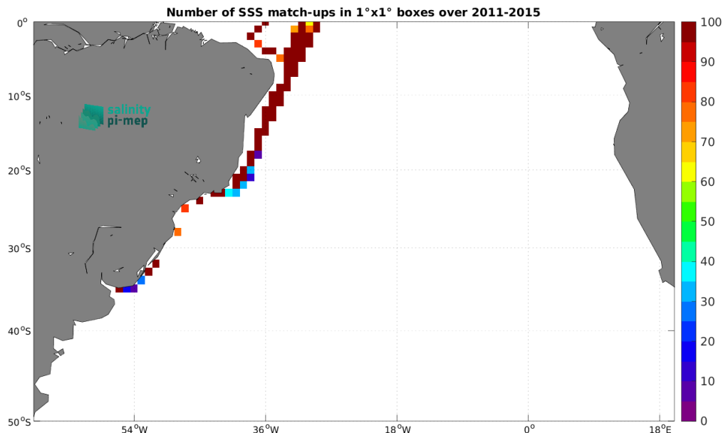
Figure 5: Number of SSS match-ups between TSG (LEGOS-DM) SSS and the Aquarius SSS L3 OR v5 - Monthly - Rain mask (NASA-GSFC) SSS product for the South Atlantic Ocean Pi-MEP region over 1^{\circ} \times 1^{\circ} boxes and for the full satellite product period.
