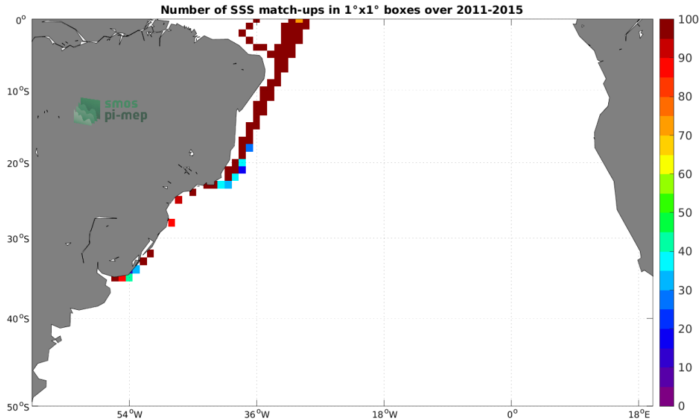
Figure 4: Number of SSS match-ups between TSG (LEGOS-DM) SSS and the Aquarius SSS L3 OR v5 - Monthly - Rain mask (NASA-GSFC) SSS product for the South Atlantic Ocean Pi-MEP region over 1^{\circ} \times 1^{\circ} boxes and for the full satellite product period.
