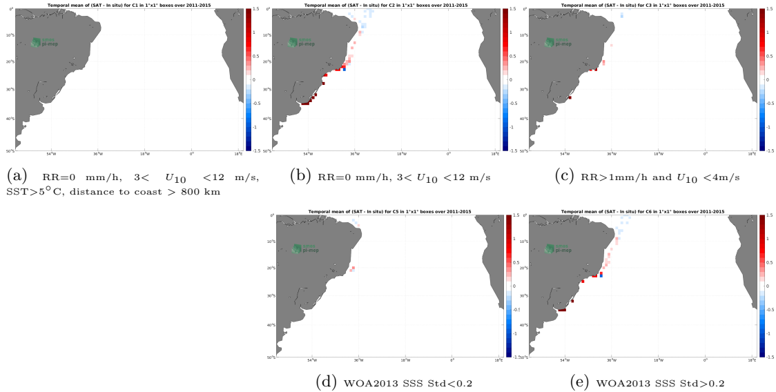
Figure 12: Temporal mean gridded over spatial boxes of size 1^{\circ}\times 1^{\circ} of \Delta\text{SSS} (Aquarius SSS L3 OR v5 - Monthly - Rain mask (NASA-GSFC) - TSG (LEGOS-DM)) for 5 different subdatasets corresponding to: \text{RR}=0 mm/h, 3 < U_{10} < 12 m/s, \text{SST} > 5^{\circ}\text{C} , distance to coast > 800 km (a), \text{RR}=0 mm/h, 3 < U_{10} < 12 m/s (b), \text{RR} > 1\text{mm/h} and U_{10} < 4\text{m/s} (c), WOA2013 SSS Std < 0.2 (d), WOA2013 SSS Std > 0.2 (e).
