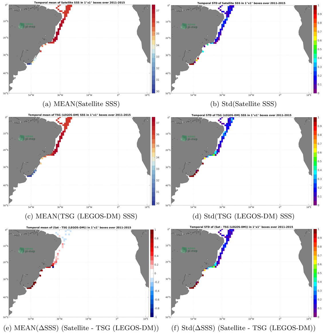
Figure 6: Temporal mean (left) and Std (right) of SSS from Aquarius SSS L3 OR v5 - Monthly - Rain mask (NASA-GSFC) (top), TSG (LEGOS-DM) (middle), and of \Delta SSS (Satellite - TSG (LEGOS-DM)). Only match-up pairs are used to generate these maps.
