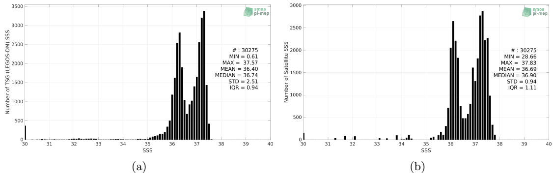
Figure 2: Histograms of SSS from TSG (LEGOS-DM) (a) and Aquarius SSS L3 OR v5 - Monthly - Rain mask (NASA-GSFC) (b) considering all match-up pairs per bins of 0.1 over the South Atlantic Ocean Pi-MEP region and for the full satellite product period.
