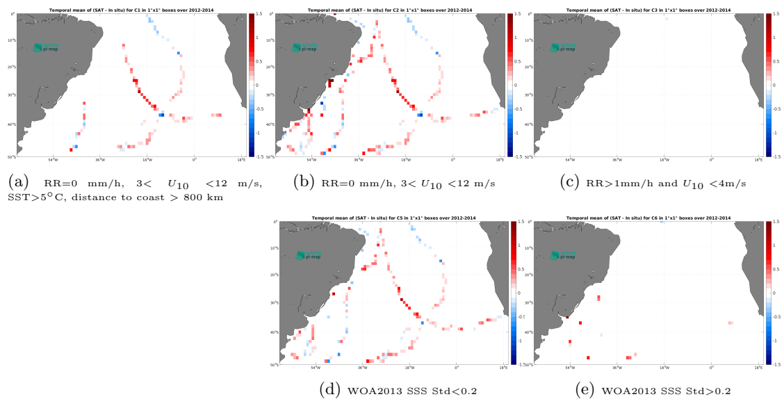
Figure 14: Temporal mean gridded over spatial boxes of size 1^\circ \times 1^\circ of \Delta\text{SSS} (Aquarius SSS L3 OR v5 - Monthly - Rain mask (NASA-GSFC) - TSG (GOSUD-Sailing-ship)) for 5 different subdatasets corresponding to:RR=0 mm/h, 3 < U_{10} < 12 m/s, SST >5^\circ\text{C} , distance to coast > 800 km (a), RR=0 mm/h, 3 < U_{10} < 12 m/s (b), RR >1 mm/h and U_{10} < 4 m/s (c), WOA2013 SSS Std <0.2 (d), WOA2013 SSS Std >0.2 (e).
