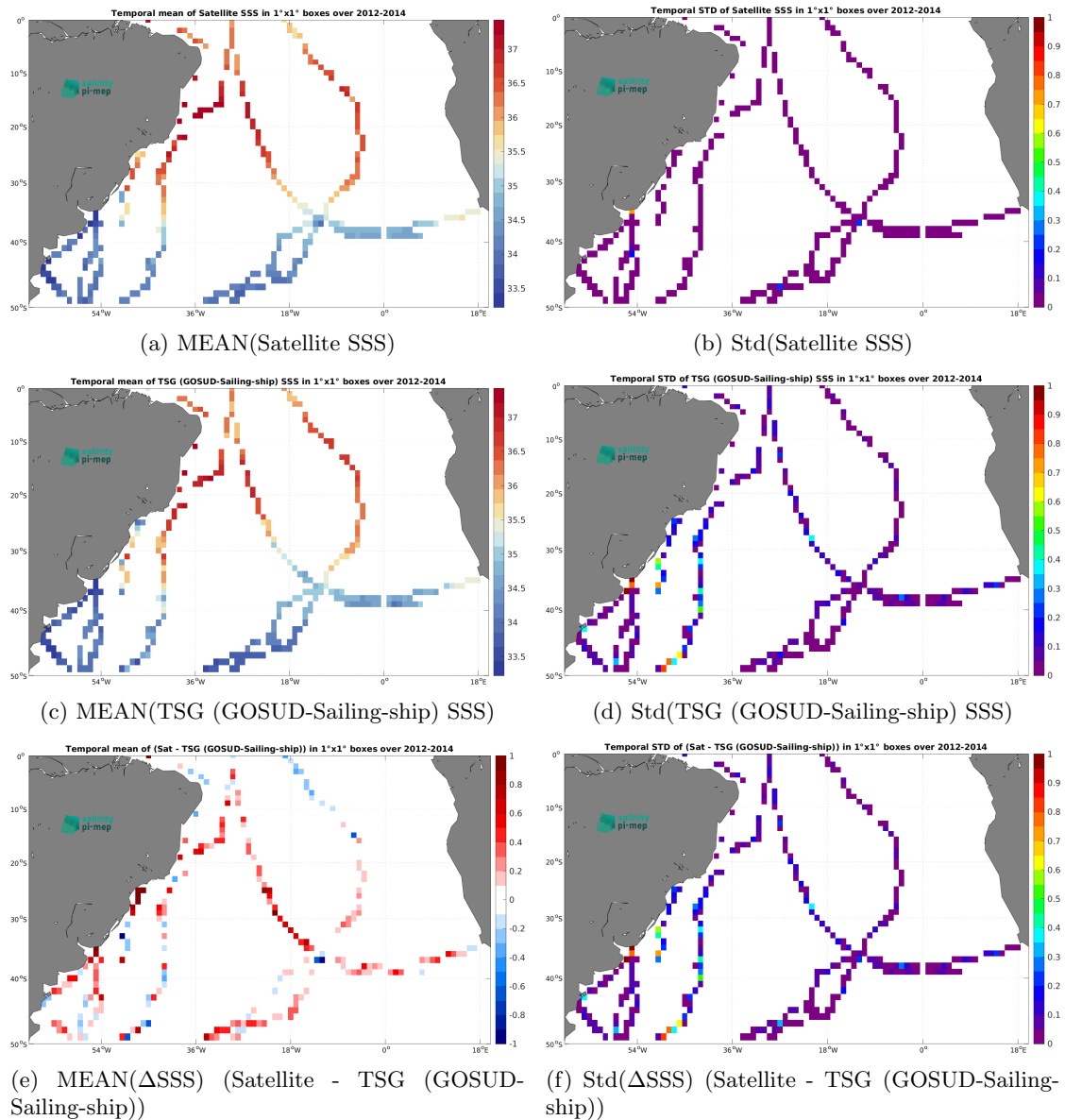
Figure 7: Temporal mean (left) and Std (right) of SSS from Aquarius SSS L3 OR v5 - Monthly - Rain mask (NASA-GSFC) (top), TSG (GOSUD-Sailing-ship) (middle), and of \Delta SSS (Satellite - TSG (GOSUD-Sailing-ship)). Only match-up pairs are used to generate these maps.
