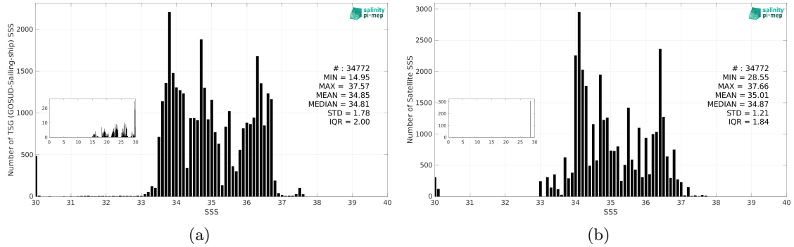
Figure 3: Histograms of SSS from TSG (GOSUD-Sailing-ship) (a) and Aquarius SSS L3 OR v5 - Monthly - Rain mask (NASA-GSFC) (b) considering all match-up pairs per bins of 0.1 over the South Atlantic Ocean Pi-MEP region and for the full satellite product period.
