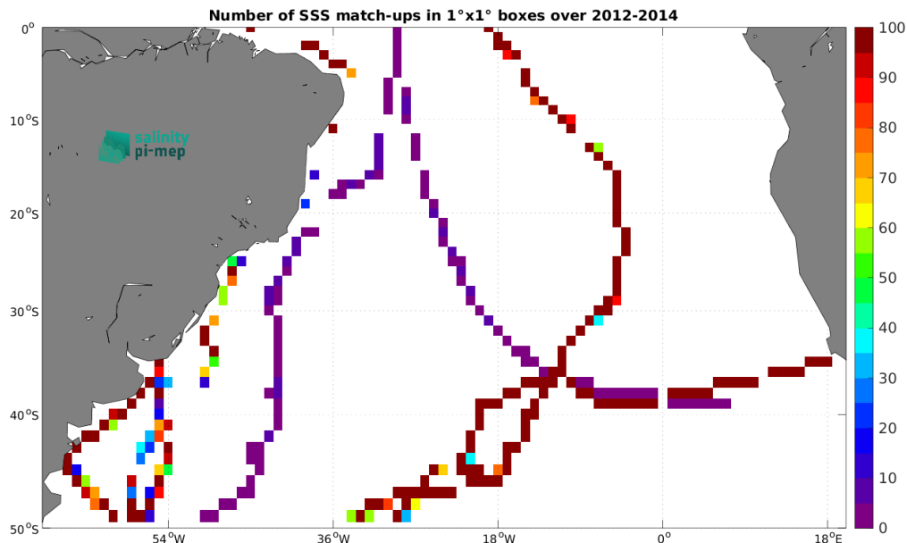
Figure 5: Number of SSS match-ups between TSG (GOSUD-Sailing-ship) SSS and the Aquarius SSS L3 OR v5 - Monthly - Rain mask (NASA-GSFC) SSS product for the South Atlantic Ocean Pi-MEP region over 1^\circ \times 1^\circ boxes and for the full satellite product period.
