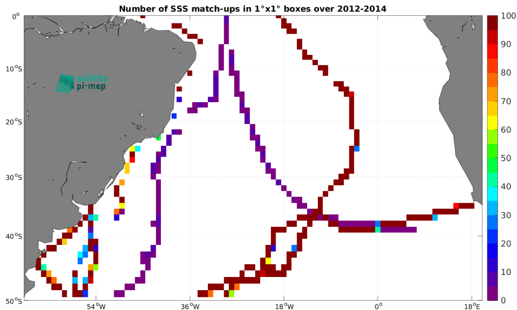
Figure 4: Number of SSS match-ups between TSG (GOSUD-Sailing-ship) SSS and the Aquarius SSS L3 OR v5 - Monthly - Rain mask (NASA-GSFC) SSS product for the South Atlantic Ocean Pi-MEP region over 1^\circ \times 1^\circ boxes and for the full satellite product period.
