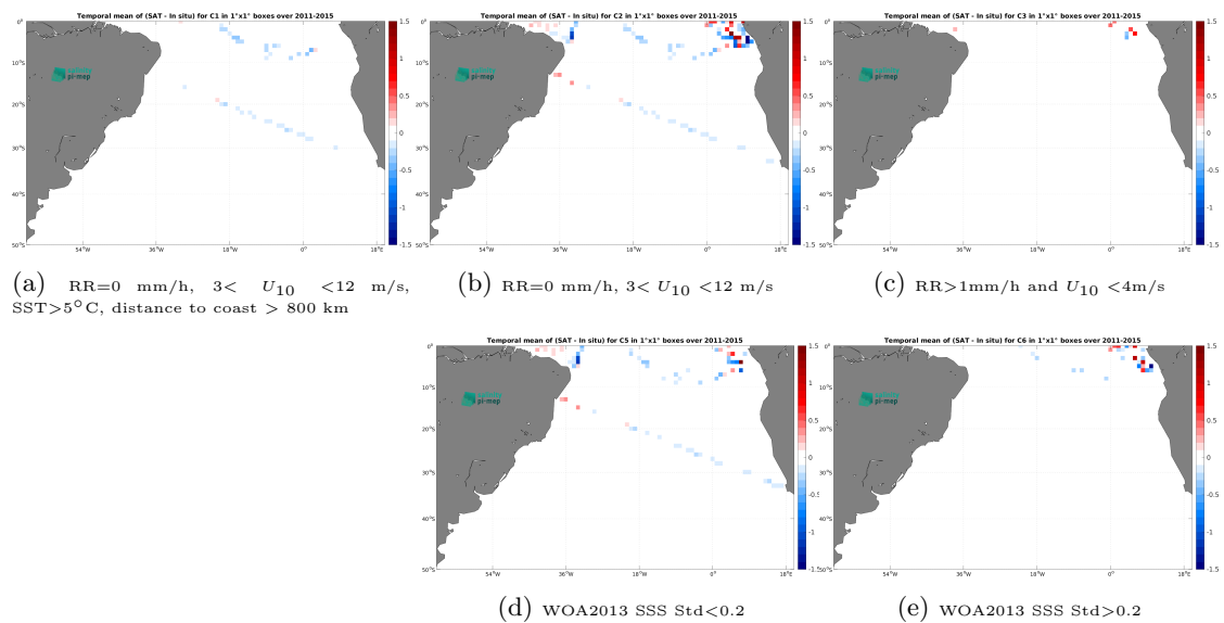
Figure 14: Temporal mean gridded over spatial boxes of size 1^\circ \times 1^\circ of \Delta SSS (Aquarius SSS L3 OR v5 - Monthly - Rain mask (NASA-GSFC) - TSG (GOSUD-Research-vessel)) for 5 different subdatasets corresponding to:RR=0 mm/h, 3 < U_{10} < 12 m/s, SST >5^\circ\text{C} , distance to coast > 800 km (a), RR=0 mm/h, 3 < U_{10} < 12 m/s (b), RR >1 mm/h and U_{10} < 4 m/s (c), WOA2013 SSS Std <0.2 (d), WOA2013 SSS Std >0.2 (e).
