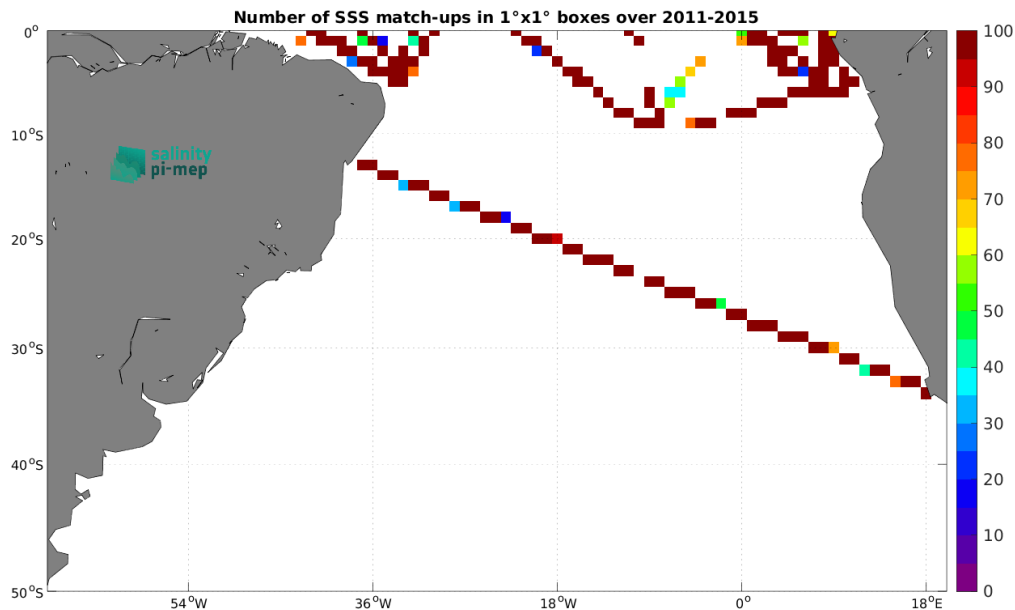
Figure 5: Number of SSS match-ups between TSG (GOSUD-Research-vessel) SSS and the Aquarius SSS L3 OR v5 - Monthly - Rain mask (NASA-GSFC) SSS product for the South Atlantic Ocean Pi-MEP region over 1^\circ \times 1^\circ boxes and for the full satellite product period.
