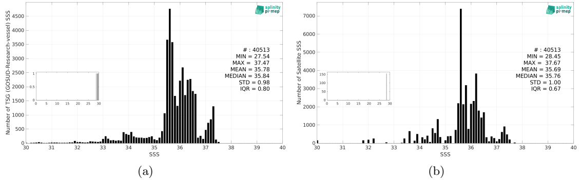
Figure 3: Histograms of SSS from TSG (GOSUD-Research-vessel) (a) and Aquarius SSS L3 OR v5 - Monthly - Rain mask (NASA-GSFC) (b) considering all match-up pairs per bins of 0.1 over the South Atlantic Ocean Pi-MEP region and for the full satellite product period.
