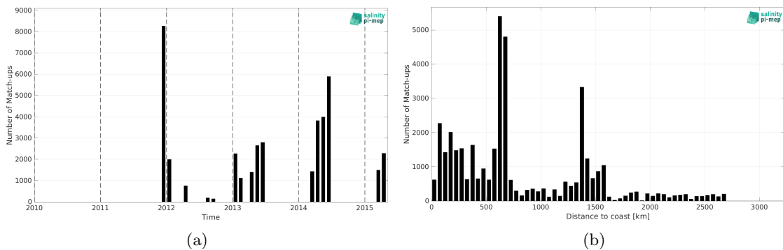
Figure 2: Number of match-ups between TSG (GOSUD-Research-vessel) and Aquarius SSS L3 OR v5 - Monthly - Rain mask (NASA-GSFC) SSS as a function of time (a) and as function of the distance to coast (b) over the South Atlantic Ocean Pi-MEP region and for the full satellite product period.
