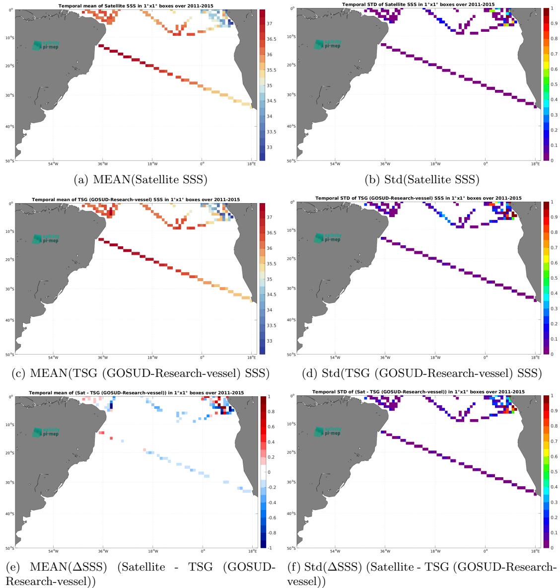
Figure 7: Temporal mean (left) and Std (right) of SSS from Aquarius SSS L3 OR v5 - Monthly - Rain mask (NASA-GSFC) (top), TSG (GOSUD-Research-vessel) (middle), and of \Delta SSS (Satellite - TSG (GOSUD-Research-vessel)). Only match-up pairs are used to generate these maps.
