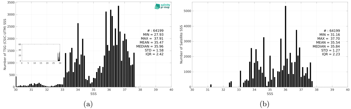
Figure 3: Histograms of SSS from TSG (CSIC-UTM) (a) and Aquarius SSS L3 OR v5 - Monthly - Rain mask (NASA-GSFC) (b) considering all match-up pairs per bins of 0.1 over the South Atlantic Ocean Pi-MEP region and for the full satellite product period.
