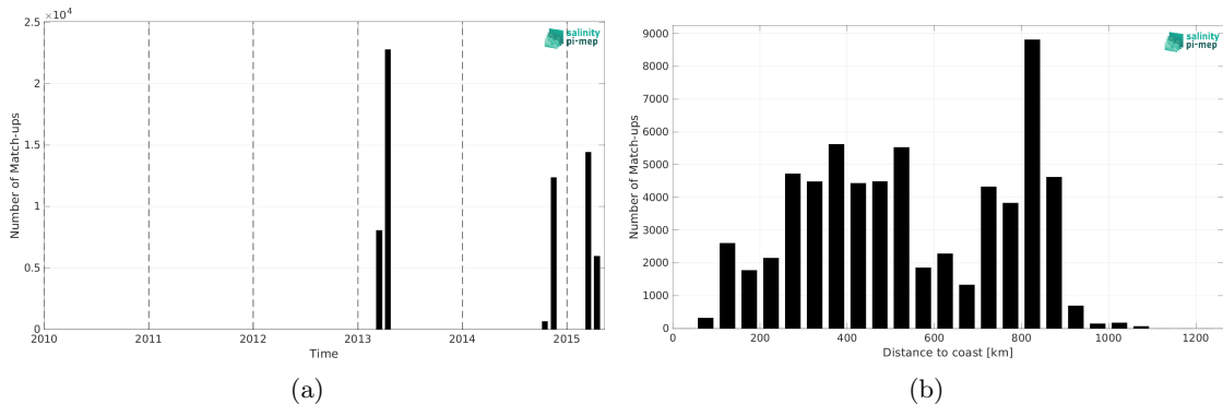
Figure 2: Number of match-ups between TSG (CSIC-UTM) and Aquarius SSS L3 OR v5 - Monthly - Rain mask (NASA-GSFC) SSS as a function of time (a) and as function of the distance to coast (b) over the South Atlantic Ocean Pi-MEP region and for the full satellite product period.
