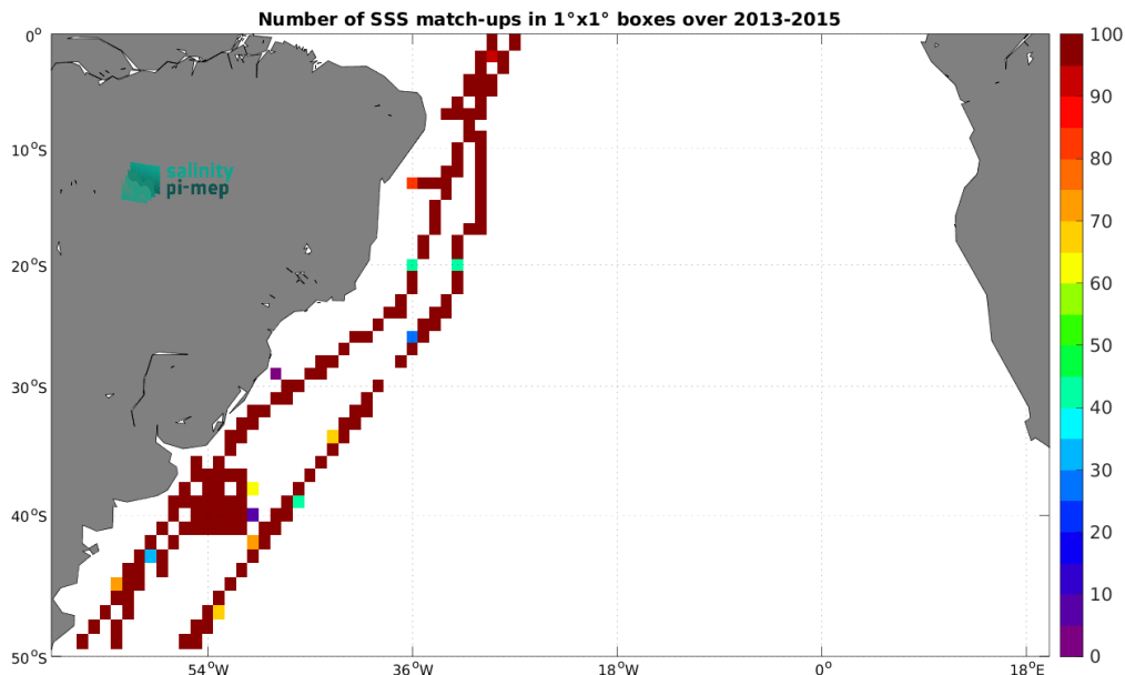
Figure 5: Number of SSS match-ups between TSG (CSIC-UTM) SSS and the Aquarius SSS L3 OR v5 - Monthly - Rain mask (NASA-GSFC) SSS product for the South Atlantic Ocean Pi-MEP region over 1^\circ \times 1^\circ boxes and for the full satellite product period.
