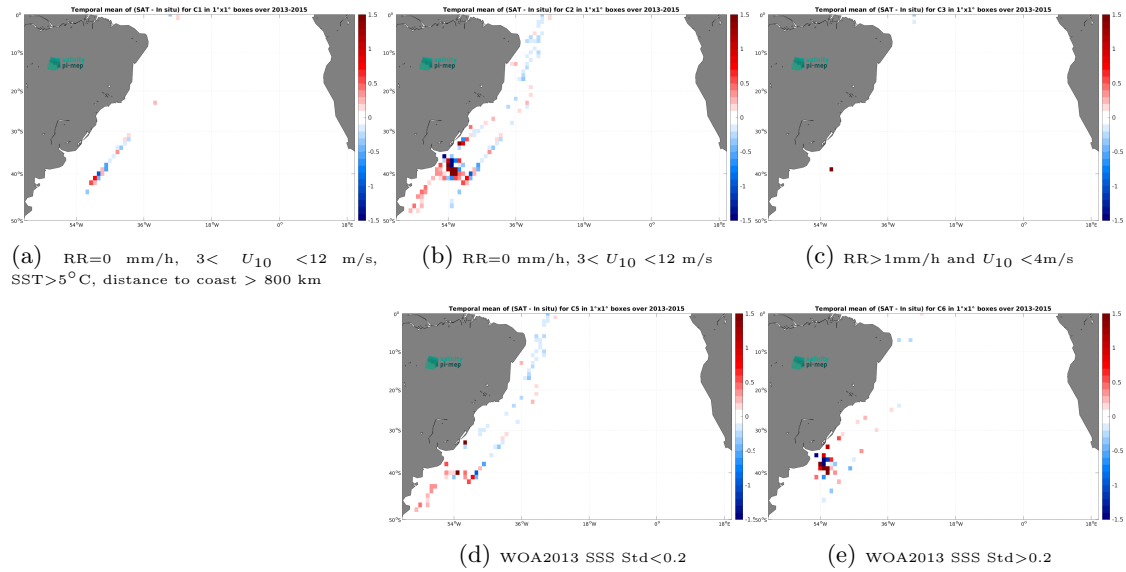
Figure 12: Temporal mean gridded over spatial boxes of size 1^\circ \times 1^\circ of \Delta\text{SSS} (Aquarius SSS L3 OR v5 - Monthly - Rain mask (NASA-GSFC) - TSG (CSIC-UTM)) for 5 different subdatasets corresponding to:RR=0 mm/h, 3 < U_{10} < 12 m/s, SST >5^\circ\text{C} , distance to coast > 800 km (a), RR=0 mm/h, 3 < U_{10} < 12 m/s (b), RR >1 mm/h and U_{10} < 4 m/s (c), WOA2013 SSS Std <0.2 (d), WOA2013 SSS Std >0.2 (e).
