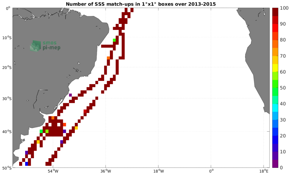
Figure 4: Number of SSS match-ups between TSG (CSIC-UTM) SSS and the Aquarius SSS L3 OR v5 - Monthly - Rain mask (NASA-GSFC) SSS product for the South Atlantic Ocean Pi-MEP region over 1°x1° boxes and for the full satellite product period.
