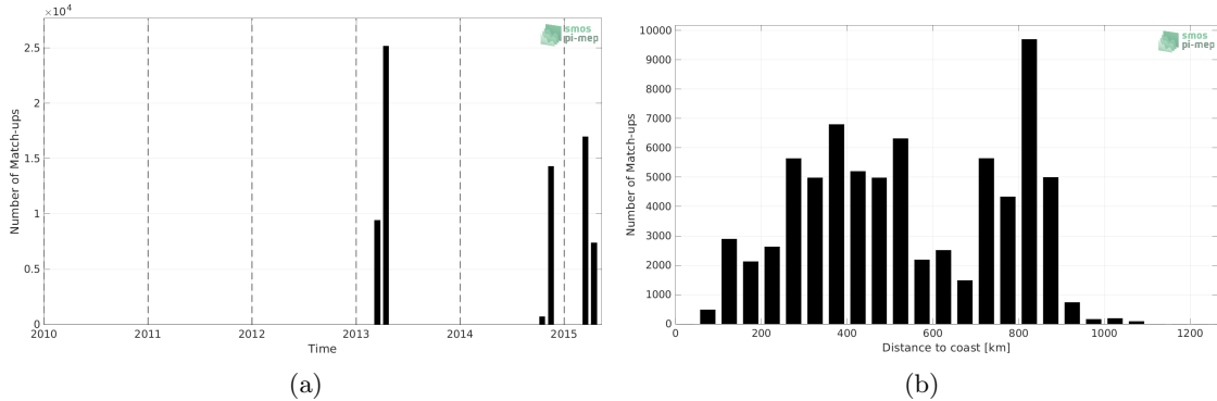
Figure 1: Number of match-ups between TSG (CSIC-UTM) and Aquarius SSS L3 OR v5 - Monthly - Rain mask (NASA-GSFC) SSS as a function of time (a) and as function of the distance to coast (b) over the South Atlantic Ocean Pi-MEP region and for the full satellite product period.
