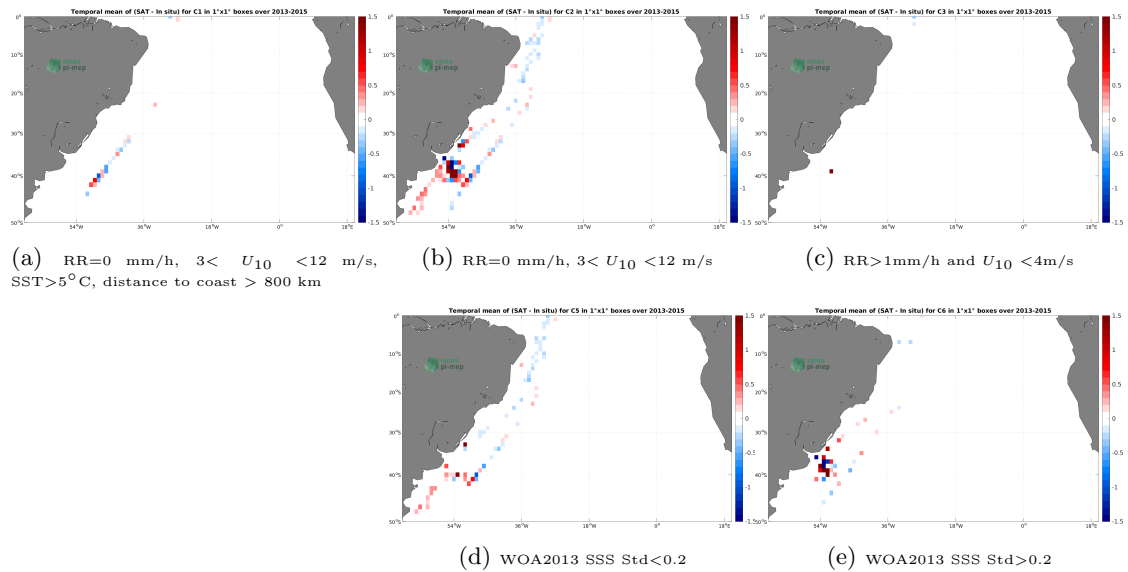
Figure 12: Temporal mean gridded over spatial boxes of size 1^\circ \times 1^\circ of \Delta SSS (Aquarius SSS L3 OR v5 - Monthly - Rain mask (NASA-GSFC) - TSG (CSIC-UTM)) for 5 different subdatasets corresponding to: RR=0 mm/h, 3 < U_{10} < 12 m/s, SST > 5^\circ C , distance to coast > 800 km (a), RR=0 mm/h, 3 < U_{10} < 12 m/s (b), RR > 1 mm/h and U_{10} < 4 m/s (c), WOA2013 SSS Std < 0.2 (d), WOA2013 SSS Std > 0.2 (e).
