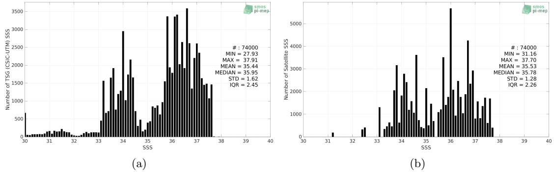
Figure 2: Histograms of SSS from TSG (CSIC-UTM) (a) and Aquarius SSS L3 OR v5 - Monthly - Rain mask (NASA-GSFC) (b) considering all match-up pairs per bins of 0.1 over the South Atlantic Ocean Pi-MEP region and for the full satellite product period.
