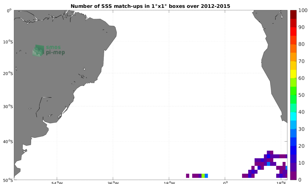
Figure 4: Number of SSS match-ups between Marine mammals SSS and the Aquarius SSS L3 OR v5 - Monthly - Rain mask (NASA-GSFC) SSS product for the South Atlantic Ocean Pi-MEP region over 1^\circ \times 1^\circ boxes and for the full satellite product period.
