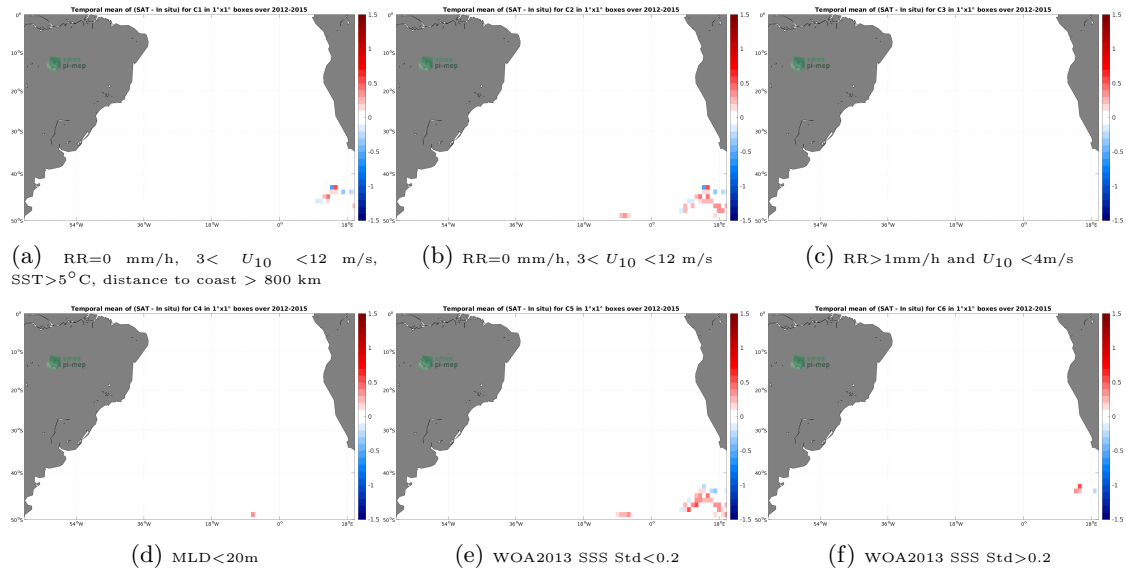
Figure 12: Temporal mean gridded over spatial boxes of size 1^{\circ}\times 1^{\circ} of \Delta\text{SSS} (Aquarius SSS L3 OR v5 - Monthly - Rain mask (NASA-GSFC) - Marine mammals) for 6 different subdatasets corresponding to:RR=0 mm/h, 3 < U_{10} < 12 m/s, SST > 5^{\circ}\text{C} , distance to coast > 800 km (a), RR=0 mm/h, 3 < U_{10} < 12 m/s (b), RR > 1\text{mm/h} and U_{10} < 4\text{m/s} (c),MLD < 20\text{m} (d),WOA2013 SSS Std < 0.2 (e),WOA2013 SSS Std > 0.2 (f).
