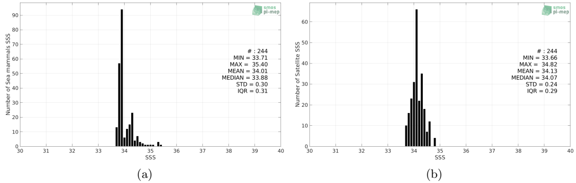
Figure 2: Histograms of SSS from Marine mammals (a) and Aquarius SSS L3 OR v5 - Monthly - Rain mask (NASA-GSFC) (b) considering all match-up pairs per bins of 0.1 over the South Atlantic Ocean Pi-MEP region and for the full satellite product period.
