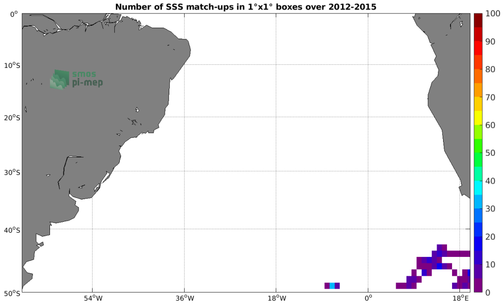
Figure 4: Number of SSS match-ups between Marine mammals SSS and the Aquarius SSS L3 OR v5 - Monthly - Rain mask (NASA-GSFC) SSS product for the South Atlantic Ocean Pi-MEP region over 1^{\circ} \times 1^{\circ} boxes and for the full satellite product period.
