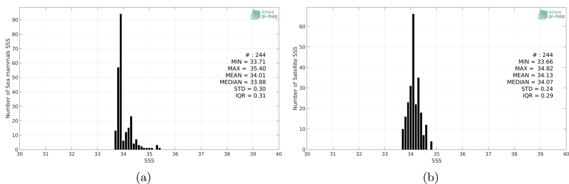
Figure 2: Histograms of SSS from Sea mammals (a) and Aquarius-L3-OR-V5-MONTHLY-RAIN-MASK-1DEG (b) considering all match-up pairs per bins of 0.1 over the South Atlantic Ocean Pi-MEP region and for the full satellite product period.
