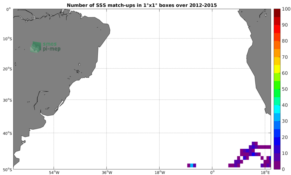
Figure 4: Number of SSS match-ups between Sea mammals SSS and the Aquarius-L3-OR-V5-MONTHLY-RAIN-MASK-1DEG SSS product for the South Atlantic Ocean Pi-MEP region over 1^\circ \times 1^\circ boxes and for the full satellite product period.
