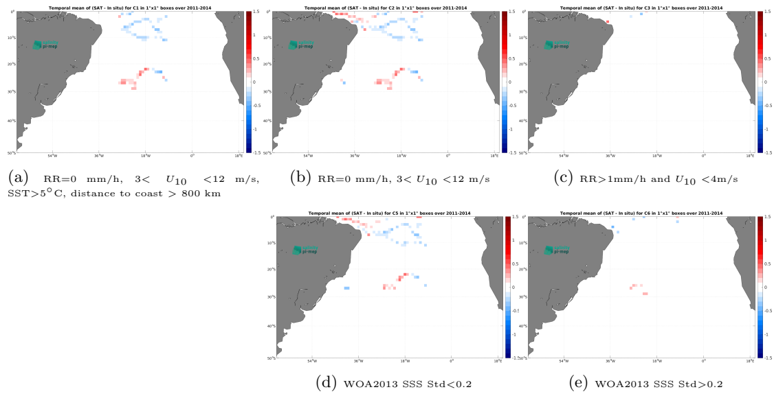
Figure 13: Temporal mean gridded over spatial boxes of size 1^\circ \times 1^\circ of \Delta\text{SSS} (Aquarius SSS L3 OR v5 - Monthly - Rain mask (NASA-GSFC) - Surface drifters) for 5 different subdatasets corresponding to:RR=0 mm/h, 3 < U_{10} < 12 m/s, SST >5^\circ\text{C} , distance to coast > 800 km (a), RR=0 mm/h, 3 < U_{10} < 12 m/s (b), RR >1 mm/h and U_{10} < 4 m/s (c), WOA2013 SSS Std <0.2 (d), WOA2013 SSS Std >0.2 (e).
