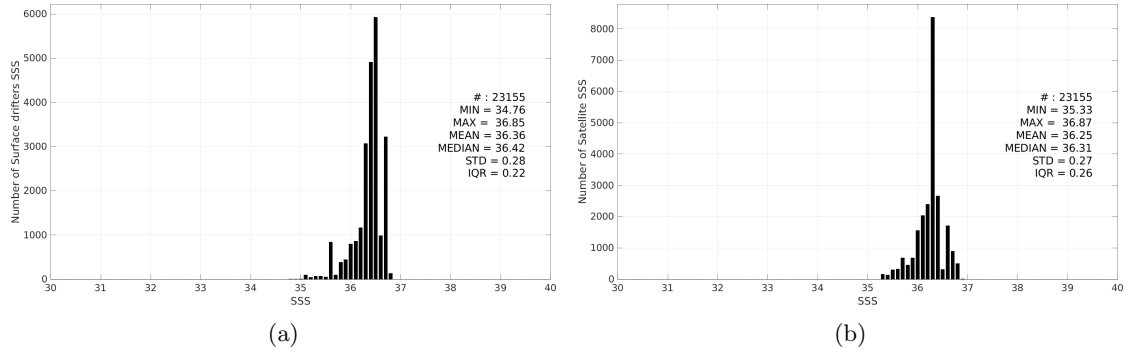
Figure 3: Histograms of SSS from Surface drifters (a) and Aquarius SSS L3 OR v5 - Monthly - Rain mask (NASA-GSFC) (b) considering all match-up pairs per bins of 0.1 over the South Atlantic Ocean Pi-MEP region and for the full satellite product period.
