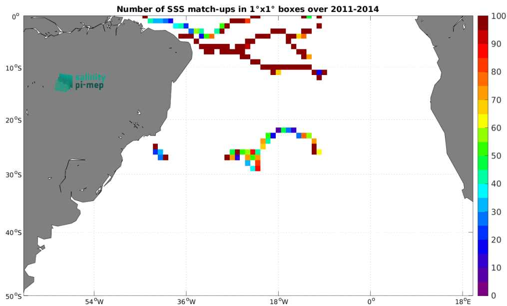
Figure 4: Number of SSS match-ups between Surface drifters SSS and the Aquarius SSS L3 OR v5 - Monthly - Rain mask (NASA-GSFC) SSS product for the South Atlantic Ocean Pi-MEP region over 1^\circ \times 1^\circ boxes and for the full satellite product period.
