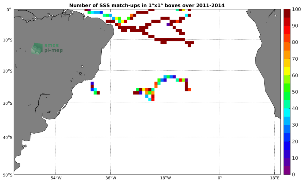
Figure 3: Number of SSS match-ups between Surface drifters SSS and the Aquarius-L3-OR-V5-MONTHLY-RAIN-MASK-1DEG SSS product for the South Atlantic Ocean Pi-MEP region over 1°x1° boxes and for the full satellite product period.
