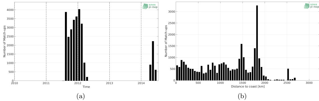
Figure 1: Number of match-ups between Surface drifters and Aquarius-L3-OR-V5-MONTHLY-RAIN-MASK-1DEG SSS as a function of time (a) and as function of the distance to coast (b) over the South Atlantic Ocean Pi-MEP region and for the full satellite product period.
