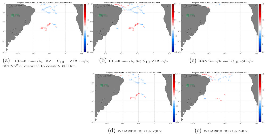
Figure 11: Temporal mean gridded over spatial boxes of size 1^\circ \times 1^\circ of \Delta SSS (Aquarius-L3-OR-V5-MONTHLY-RAIN-MASK-1DEG - Surface drifters) for 5 different subdatasets corresponding to:RR=0 mm/h, 3 < U_{10} < 12 m/s, SST >5^\circ\text{C} , distance to coast > 800 km (a), RR=0 mm/h, 3 < U_{10} < 12 m/s (b), RR >1 mm/h and U_{10} < 4 m/s (c), WOA2013 SSS Std <0.2 (d), WOA2013 SSS Std >0.2 (e).
