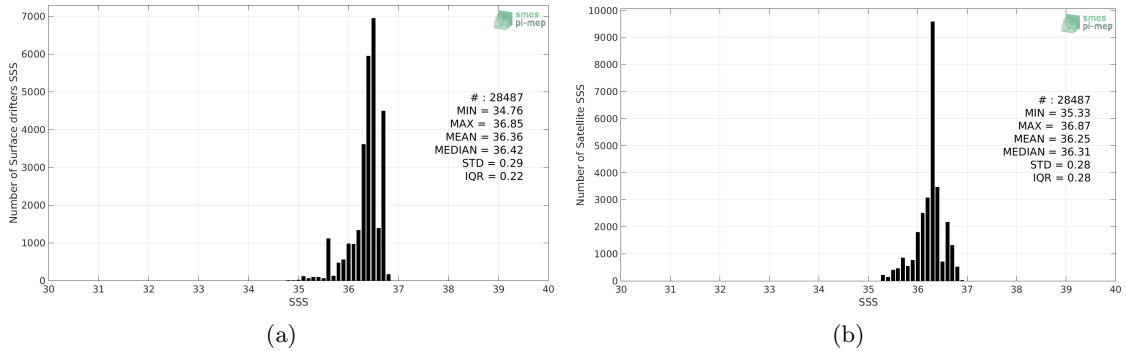
Figure 2: Histograms of SSS from Surface drifters (a) and Aquarius-L3-OR-V5-MONTHLY-RAIN-MASK-1DEG (b) considering all match-up pairs per bins of 0.1 over the South Atlantic Ocean Pi-MEP region and for the full satellite product period.
