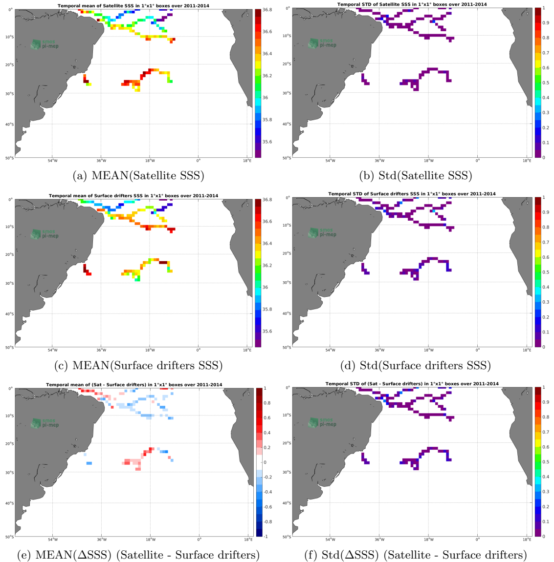
Figure 5: Temporal mean (left) and Std (right) of SSS from Aquarius-L3-OR-V5-MONTHLY-RAIN-MASK-1DEG (top), Surface drifters (middle), and of \Delta SSS (Satellite - Surface drifters). Only match-up pairs are used to generate these maps.
