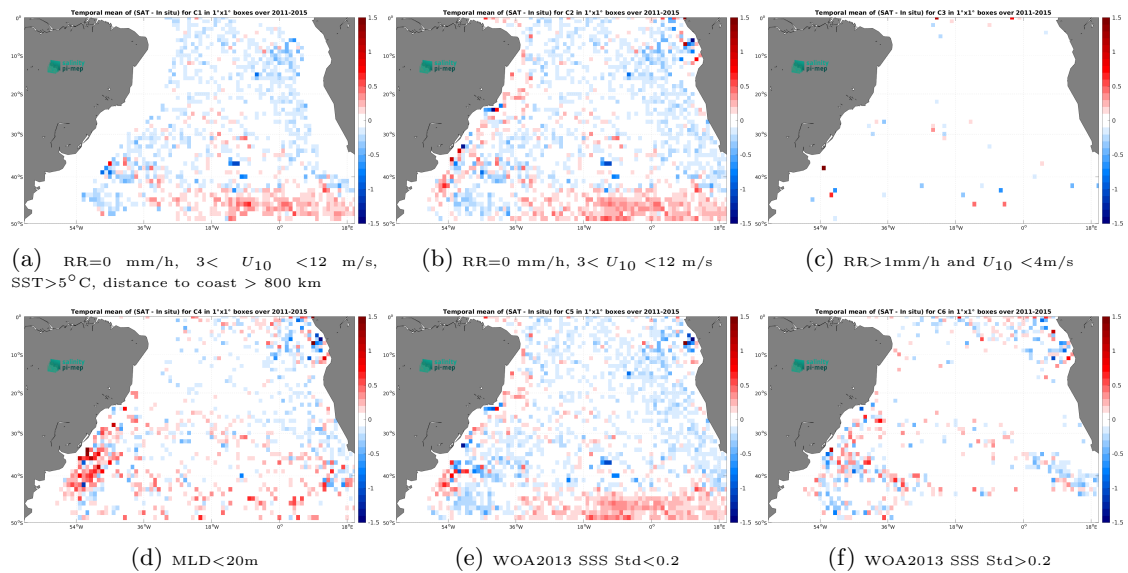
Figure 14: Temporal mean gridded over spatial boxes of size 1^\circ \times 1^\circ of \Delta SSS (Aquarius SSS L3 OR v5 - Monthly - Rain mask (NASA-GSFC) - Argo) for 6 different subdatasets corresponding to:RR=0 mm/h, 3 < U_{10} < 12 m/s, SST >5^\circ C, distance to coast > 800 km (a), RR=0 mm/h, 3 < U_{10} < 12 m/s (b), RR >1 mm/h and U_{10} < 4 m/s (c),MLD <20 m (d),WOA2013 SSS Std <0.2 (e),WOA2013 SSS Std >0.2 (f).
