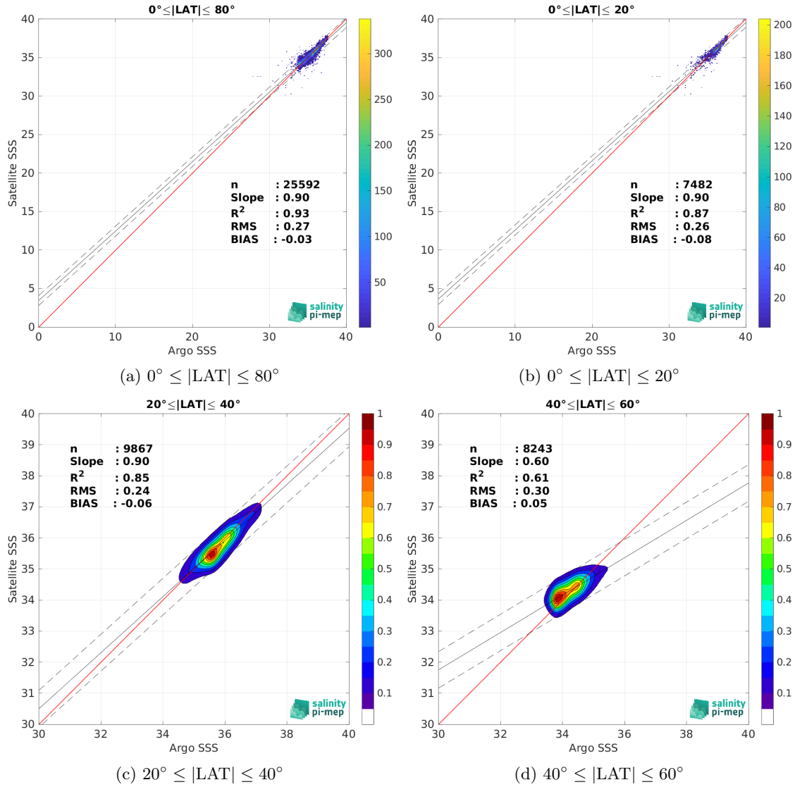
Figure 10: Contour maps of the concentration of Aquarius SSS L3 OR v5 - Monthly - Rain mask (NASA-GSFC) SSS ( y -axis) versus Argo SSS ( x -axis) at match-up pairs for different latitude bands. For each plot, the red line shows x=y . The black thin and dashed lines indicate a linear fit through the data cloud and the \pm 95\% confidence levels, respectively. The number match-up pairs n , the slope and R^2 coefficient of the linear fit, the root mean square (RMS) and the mean bias between satellite and in situ data are indicated for each latitude band in each plots.
