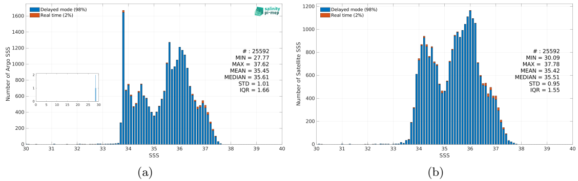
Figure 3: Histograms of SSS from Argo (a) and Aquarius SSS L3 OR v5 - Monthly - Rain mask (NASA-GSFC) (b) considering all match-up pairs per bins of 0.1 over the South Atlantic Ocean Pi-MEP region and for the full satellite product period.
