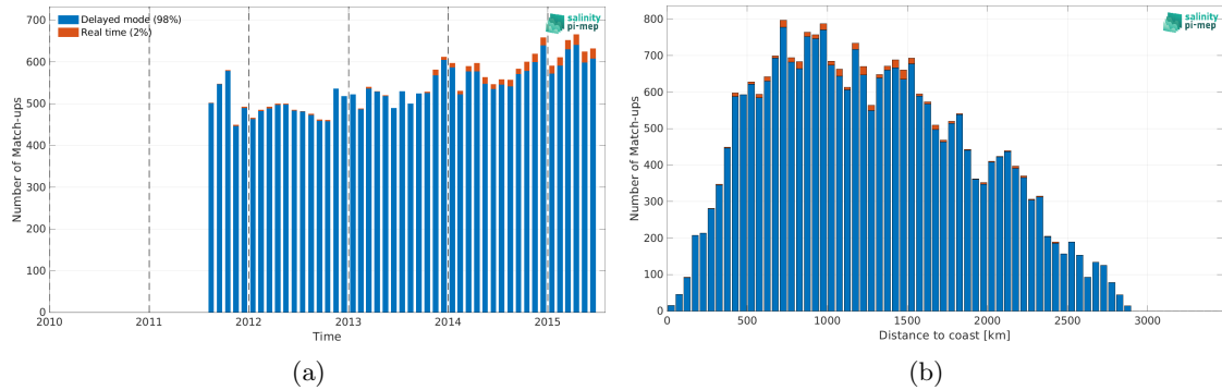
Figure 2: Number of match-ups between Argo and Aquarius SSS L3 OR v5 - Monthly - Rain mask (NASA-GSFC) SSS as a function of time (a) and as function of the distance to coast (b) over the South Atlantic Ocean Pi-MEP region and for the full satellite product period.
