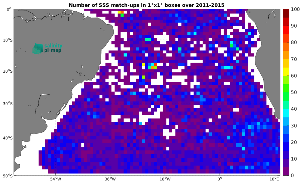
Figure 5: Number of SSS match-ups between Argo SSS and the Aquarius SSS L3 OR v5 - Monthly - Rain mask (NASA-GSFC) SSS product for the South Atlantic Ocean Pi-MEP region over 1^\circ \times 1^\circ boxes and for the full satellite product period.
