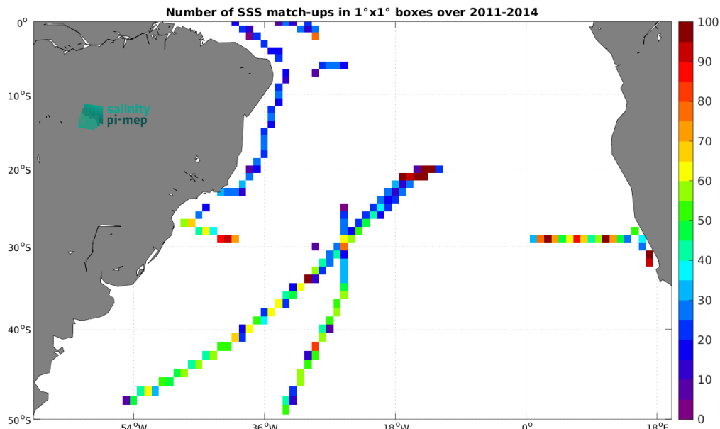
Figure 5: Number of SSS match-ups between TSG (SAMOS) SSS and the Aquarius SSS L3 CAP v5 - 7-Day running (JPL) SSS product for the South Atlantic Ocean Pi-MEP region over 1^\circ \times 1^\circ boxes and for the full satellite product period.
