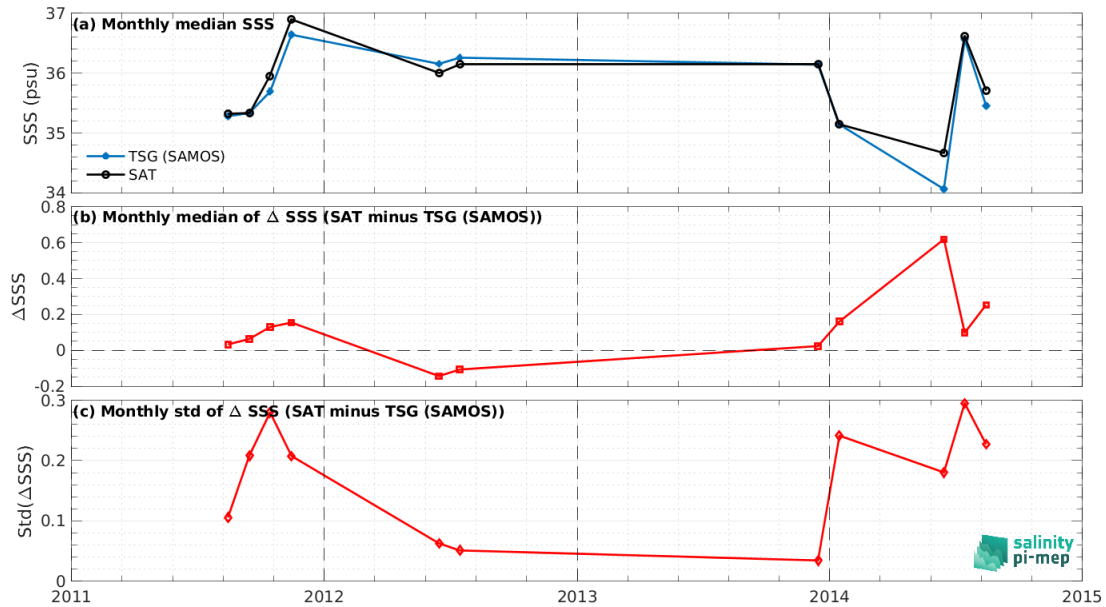
Figure 8: Time series of the monthly median SSS (top), median of \Delta\text{SSS} (Satellite - TSG (SAMOS)) and Std of \Delta\text{SSS} (Satellite - TSG (SAMOS)) over the South Atlantic Ocean Pi-MEP region considering all match-ups collected by the Pi-MEP.
