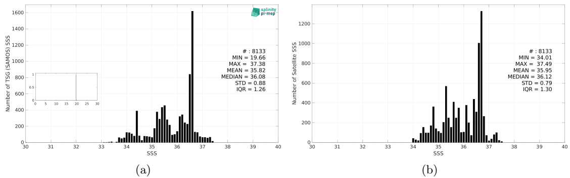
Figure 3: Histograms of SSS from TSG (SAMOS) (a) and Aquarius SSS L3 CAP v5 - 7-Day running (JPL) (b) considering all match-up pairs per bins of 0.1 over the South Atlantic Ocean Pi-MEP region and for the full satellite product period.
