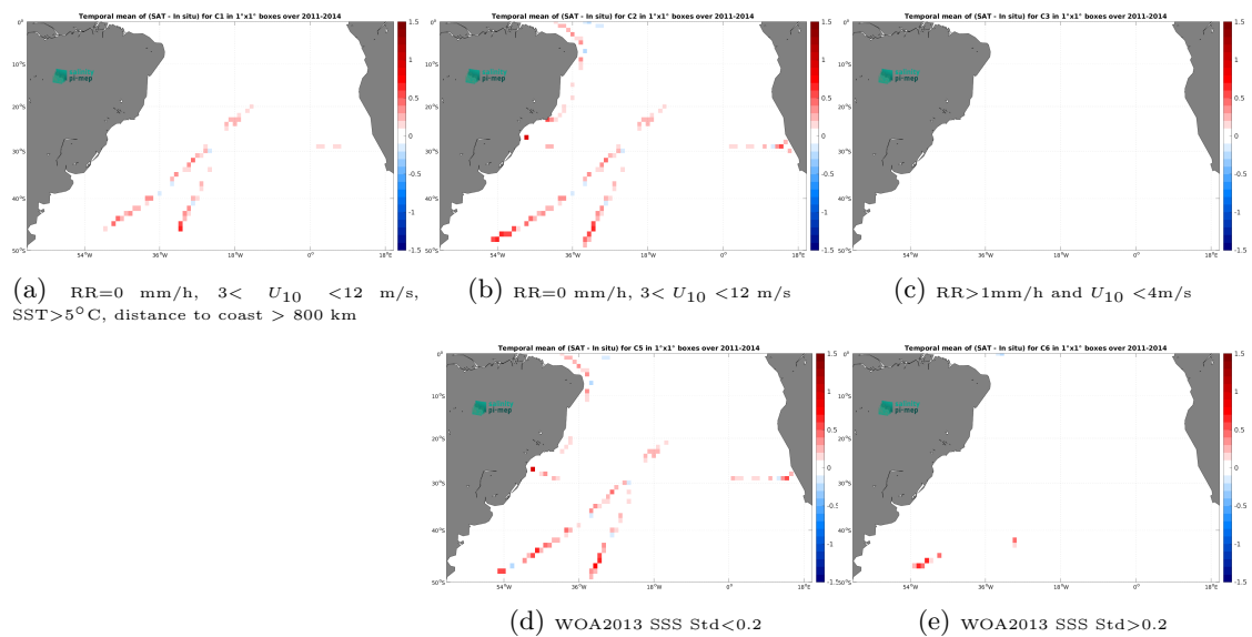
Figure 14: Temporal mean gridded over spatial boxes of size 1^\circ \times 1^\circ of \Delta\text{SSS} (Aquarius SSS L3 CAP v5 - 7-Day running (JPL) - TSG (SAMOS)) for 5 different subdatasets corresponding to:RR=0 mm/h, 3 < U_{10} < 12 m/s, SST >5^\circ\text{C} , distance to coast > 800 km (a), RR=0 mm/h, 3 < U_{10} < 12 m/s (b), RR >1 mm/h and U_{10} < 4 m/s (c), WOA2013 SSS Std <0.2 (d), WOA2013 SSS Std >0.2 (e).
