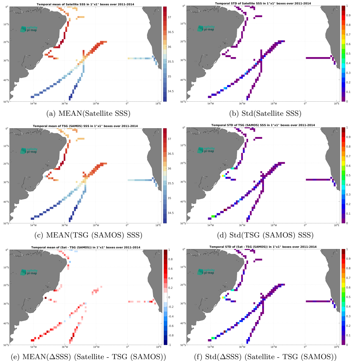
Figure 7: Temporal mean (left) and Std (right) of SSS from Aquarius SSS L3 CAP v5 - 7-Day running (JPL) (top), TSG (SAMOS) (middle), and of \Delta SSS (Satellite - TSG (SAMOS)). Only match-up pairs are used to generate these maps.
