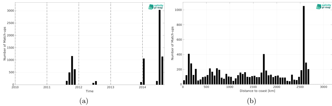
Figure 2: Number of match-ups between TSG (SAMOS) and Aquarius SSS L3 CAP v5 - 7-Day running (JPL) SSS as a function of time (a) and as function of the distance to coast (b) over the South Atlantic Ocean Pi-MEP region and for the full satellite product period.
