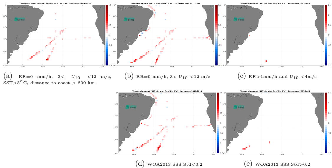
Figure 12: Temporal mean gridded over spatial boxes of size 1^\circ \times 1^\circ of \Delta\text{SSS} (Aquarius SSS L3 CAP v5 - 7-Day running (JPL) - TSG (SAMOS)) for 5 different subdatasets corresponding to:RR=0 mm/h, 3 < U_{10} < 12 m/s, SST >5^\circ\text{C} , distance to coast > 800 km (a), RR=0 mm/h, 3 < U_{10} < 12 m/s (b), RR >1 mm/h and U_{10} < 4 m/s (c), WOA2013 SSS Std <0.2 (d), WOA2013 SSS Std >0.2 (e).
