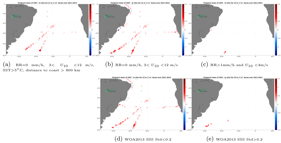
Figure 12: Temporal mean gridded over spatial boxes of size 1^\circ \times 1^\circ of \Delta\text{SSS} (Aquarius SSS L3 CAP v5 - 7-Day running (JPL) - TSG (SAMOS)) for 5 different subdatasets corresponding to:RR=0 mm/h, 3 < U_{10} < 12 m/s, SST >5^\circ\text{C} , distance to coast > 800 km (a), RR=0 mm/h, 3 < U_{10} < 12 m/s (b), RR >1 mm/h and U_{10} < 4 m/s (c), WOA2013 SSS Std <0.2 (d), WOA2013 SSS Std >0.2 (e).
