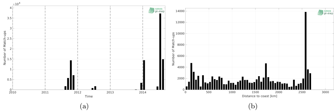
Figure 1: Number of match-ups between TSG (SAMOS) and Aquarius SSS L3 CAP v5 - 7-Day running (JPL) SSS as a function of time (a) and as function of the distance to coast (b) over the South Atlantic Ocean Pi-MEP region and for the full satellite product period.
