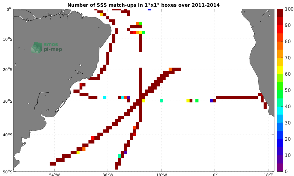
Figure 4: Number of SSS match-ups between TSG (SAMOS) SSS and the Aquarius SSS L3 CAP v5 - 7-Day running (JPL) SSS product for the South Atlantic Ocean Pi-MEP region over 1^\circ \times 1^\circ boxes and for the full satellite product period.
