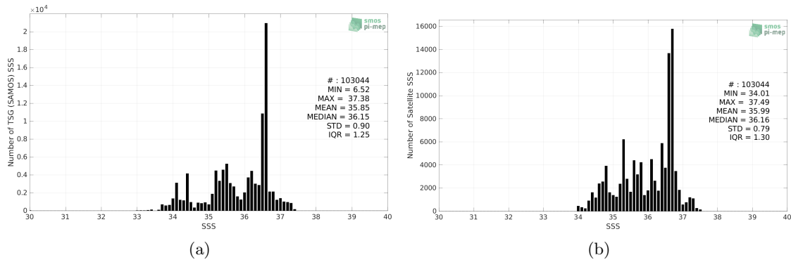
Figure 2: Histograms of SSS from TSG (SAMOS) (a) and Aquarius SSS L3 CAP v5 - 7-Day running (JPL) (b) considering all match-up pairs per bins of 0.1 over the South Atlantic Ocean Pi-MEP region and for the full satellite product period.
