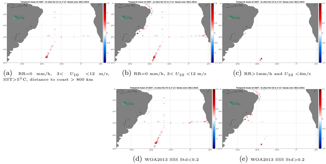
Figure 12: Temporal mean gridded over spatial boxes of size 1^\circ \times 1^\circ of \Delta SSS (Aquarius-L3-JPL-V5-7DAY-RUNNING - TSG-SAMOS) for 5 different subdatasets corresponding to: RR=0 mm/h, 3 < U_{10} < 12 m/s, SST > 5^\circ C , distance to coast > 800 km (a), RR=0 mm/h, 3 < U_{10} < 12 m/s (b), RR > 1 mm/h and U_{10} < 4 m/s (c), WOA2013 SSS Std < 0.2 (d), WOA2013 SSS Std > 0.2 (e).
