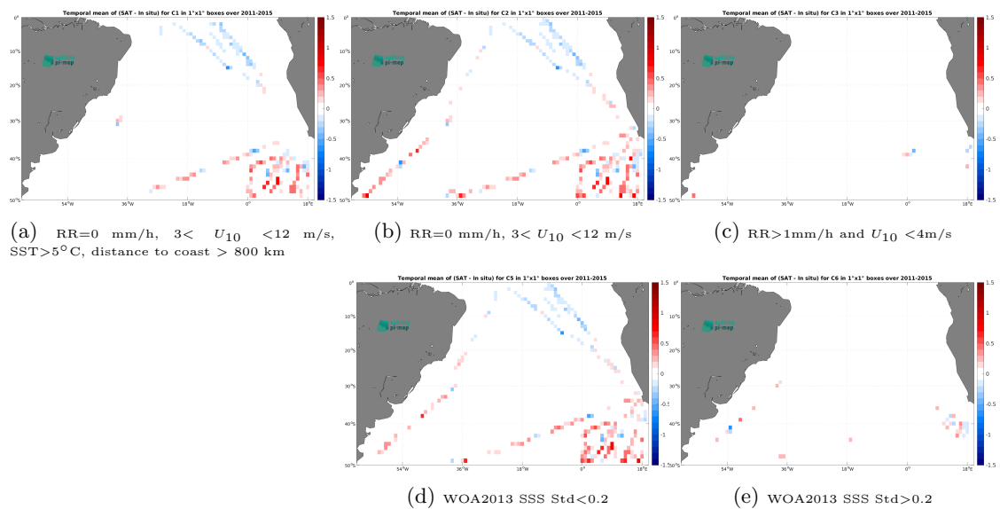
Figure 14: Temporal mean gridded over spatial boxes of size 1^\circ \times 1^\circ of \Delta SSS (Aquarius SSS L3 CAP v5 - 7-Day running (JPL) - TSG (Polarstern)) for 5 different subdatasets corresponding to:RR=0 mm/h, 3 < U_{10} < 12 m/s, SST >5^\circ\text{C} , distance to coast > 800 km (a), RR=0 mm/h, 3 < U_{10} < 12 m/s (b), RR >1 mm/h and U_{10} < 4 m/s (c), WOA2013 SSS Std <0.2 (d), WOA2013 SSS Std >0.2 (e).
