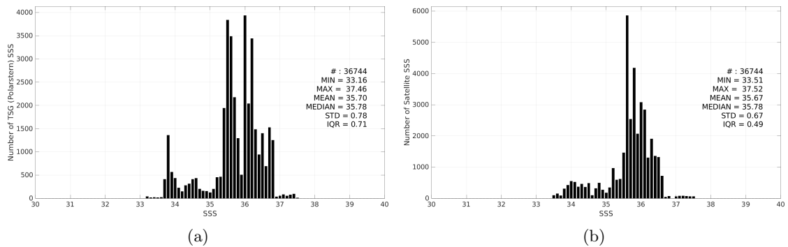
Figure 3: Histograms of SSS from TSG (Polarstern) (a) and Aquarius SSS L3 CAP v5 - 7-Day running (JPL) (b) considering all match-up pairs per bins of 0.1 over the South Atlantic Ocean Pi-MEP region and for the full satellite product period.
