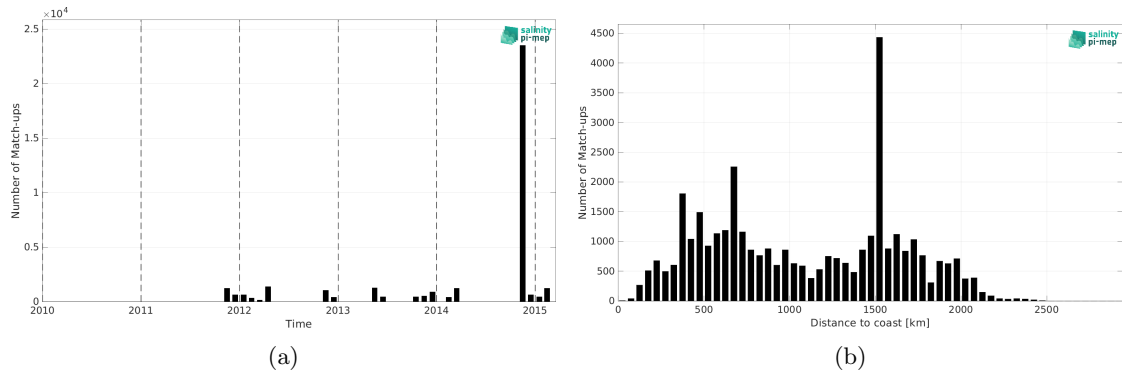
Figure 2: Number of match-ups between TSG (Polarstern) and Aquarius SSS L3 CAP v5 - 7-Day running (JPL) SSS as a function of time (a) and as function of the distance to coast (b) over the South Atlantic Ocean Pi-MEP region and for the full satellite product period.
