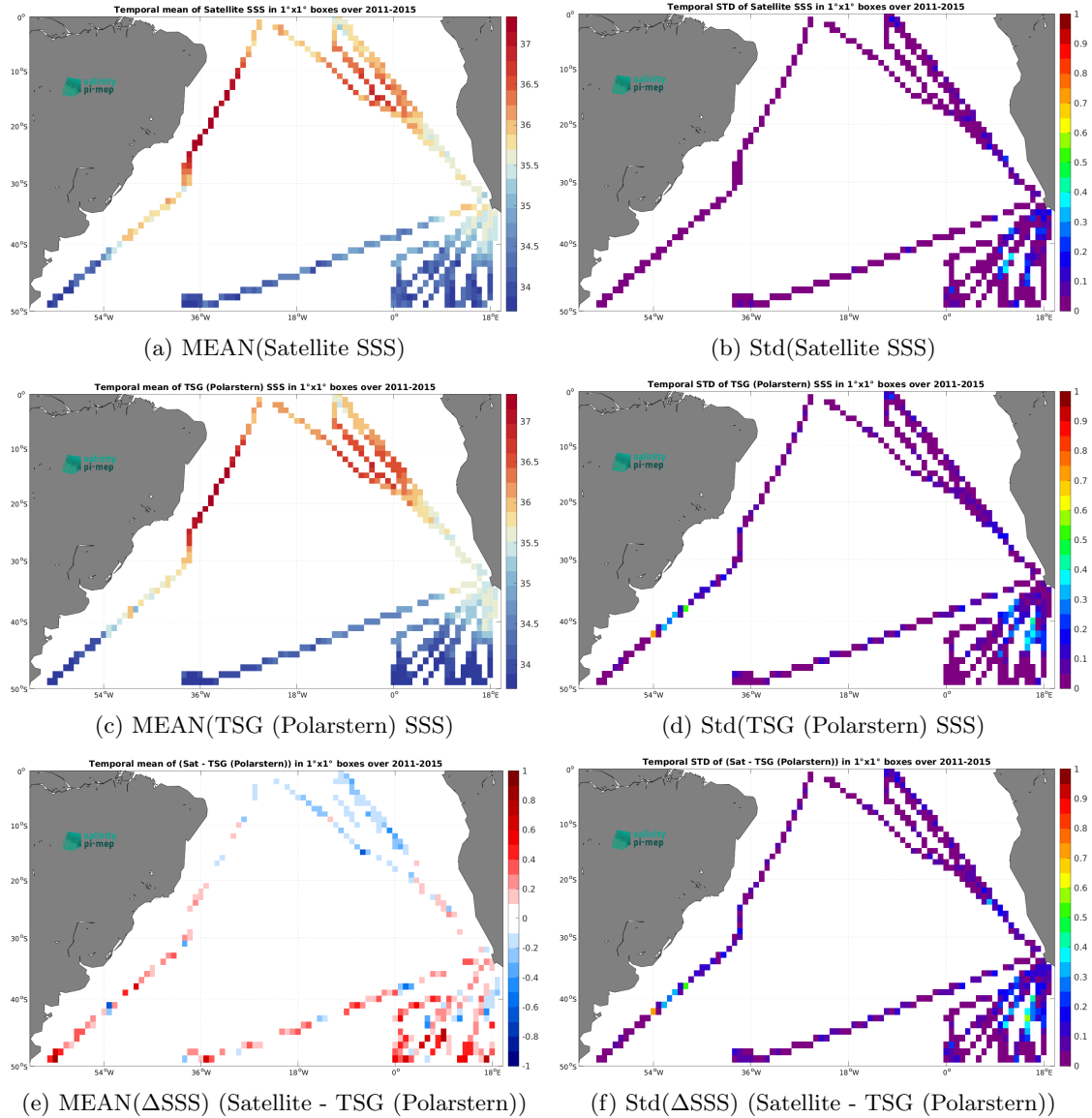
Figure 7: Temporal mean (left) and Std (right) of SSS from Aquarius SSS L3 CAP v5 - 7-Day running (JPL) (top), TSG (Polarstern) (middle), and of \Delta SSS (Satellite - TSG (Polarstern)). Only match-up pairs are used to generate these maps.
