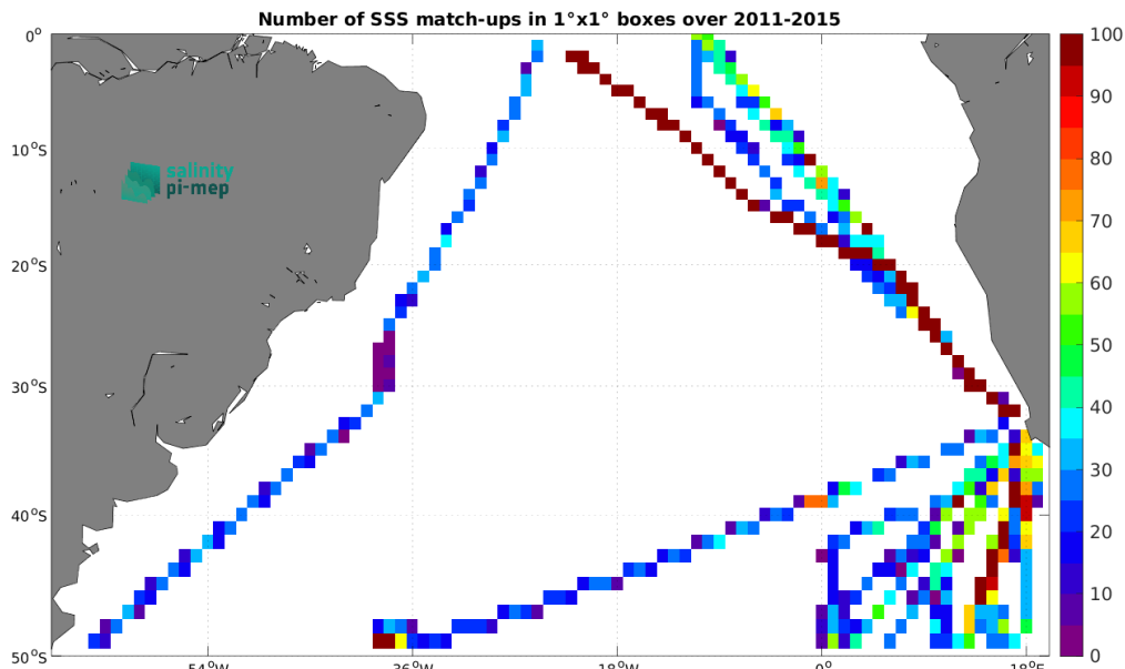
Figure 5: Number of SSS match-ups between TSG (Polarstern) SSS and the Aquarius SSS L3 CAP v5 - 7-Day running (JPL) SSS product for the South Atlantic Ocean Pi-MEP region over 1^\circ \times 1^\circ boxes and for the full satellite product period.
