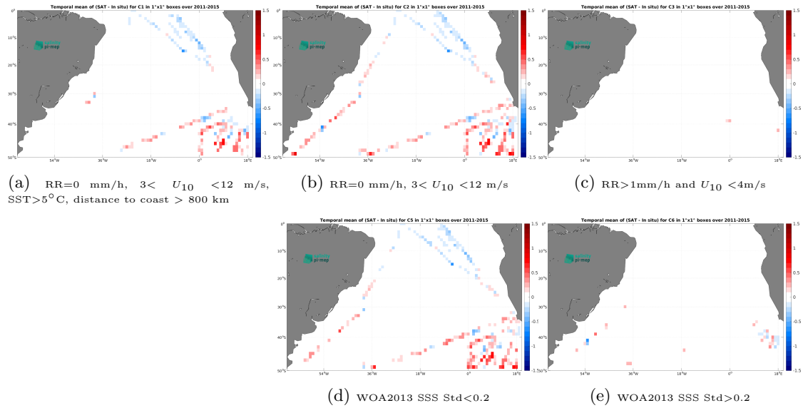
Figure 12: Temporal mean gridded over spatial boxes of size 1^\circ \times 1^\circ of \Delta\text{SSS} (Aquarius SSS L3 CAP v5 - 7-Day running (JPL) - TSG (Polarstern)) for 5 different subdatasets corresponding to:RR=0 mm/h, 3 < U_{10} < 12 m/s, SST >5^\circ\text{C} , distance to coast > 800 km (a), RR=0 mm/h, 3 < U_{10} < 12 m/s (b), RR >1 mm/h and U_{10} < 4 m/s (c), WOA2013 SSS Std <0.2 (d), WOA2013 SSS Std >0.2 (e).
