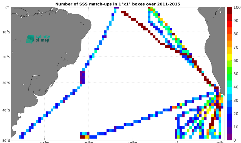
Figure 4: Number of SSS match-ups between TSG (Polarstern) SSS and the Aquarius SSS L3 CAP v5 - 7-Day running (JPL) SSS product for the South Atlantic Ocean Pi-MEP region over 1^\circ \times 1^\circ boxes and for the full satellite product period.
