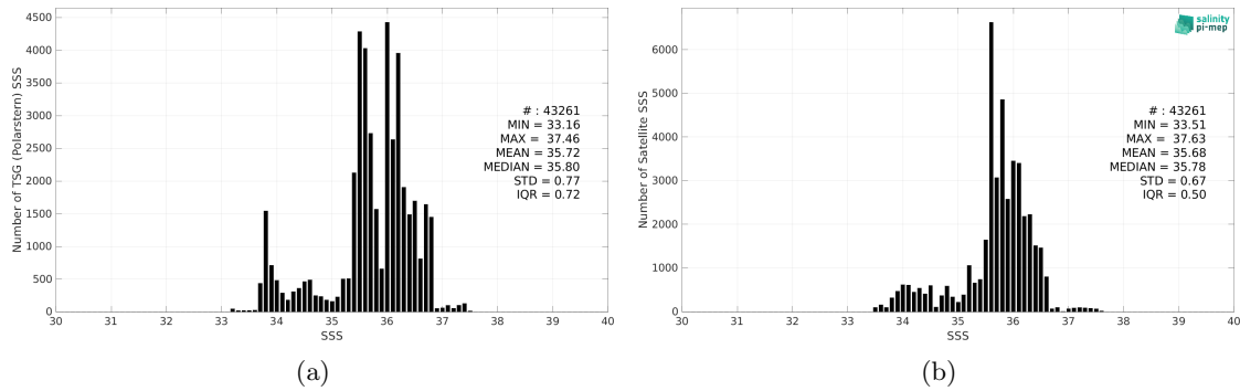
Figure 2: Histograms of SSS from TSG (Polarstern) (a) and Aquarius SSS L3 CAP v5 - 7-Day running (JPL) (b) considering all match-up pairs per bins of 0.1 over the South Atlantic Ocean Pi-MEP region and for the full satellite product period.
