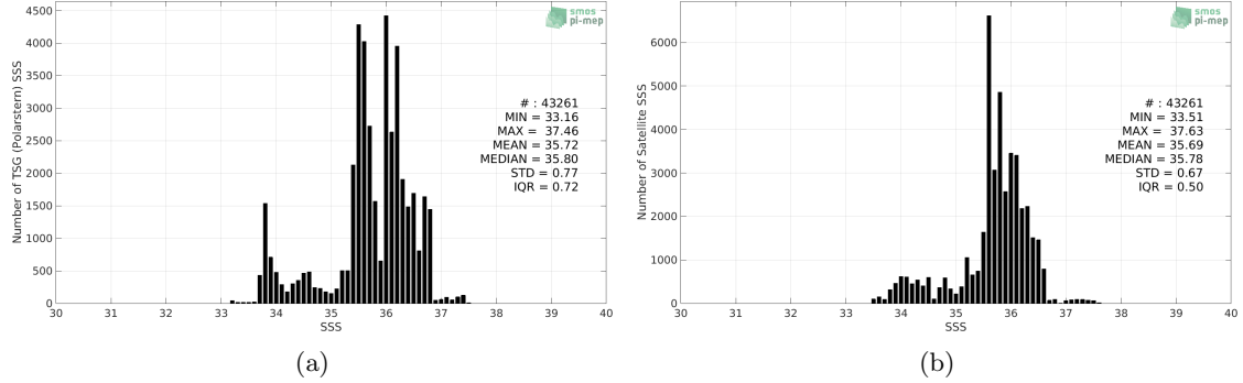
Figure 2: Histograms of SSS from TSG (Polarstern) (a) and Aquarius SSS L3 CAP v5 - 7-Day running (JPL) (b) considering all match-up pairs per bins of 0.1 over the South Atlantic Ocean Pi-MEP region and for the full satellite product period.
