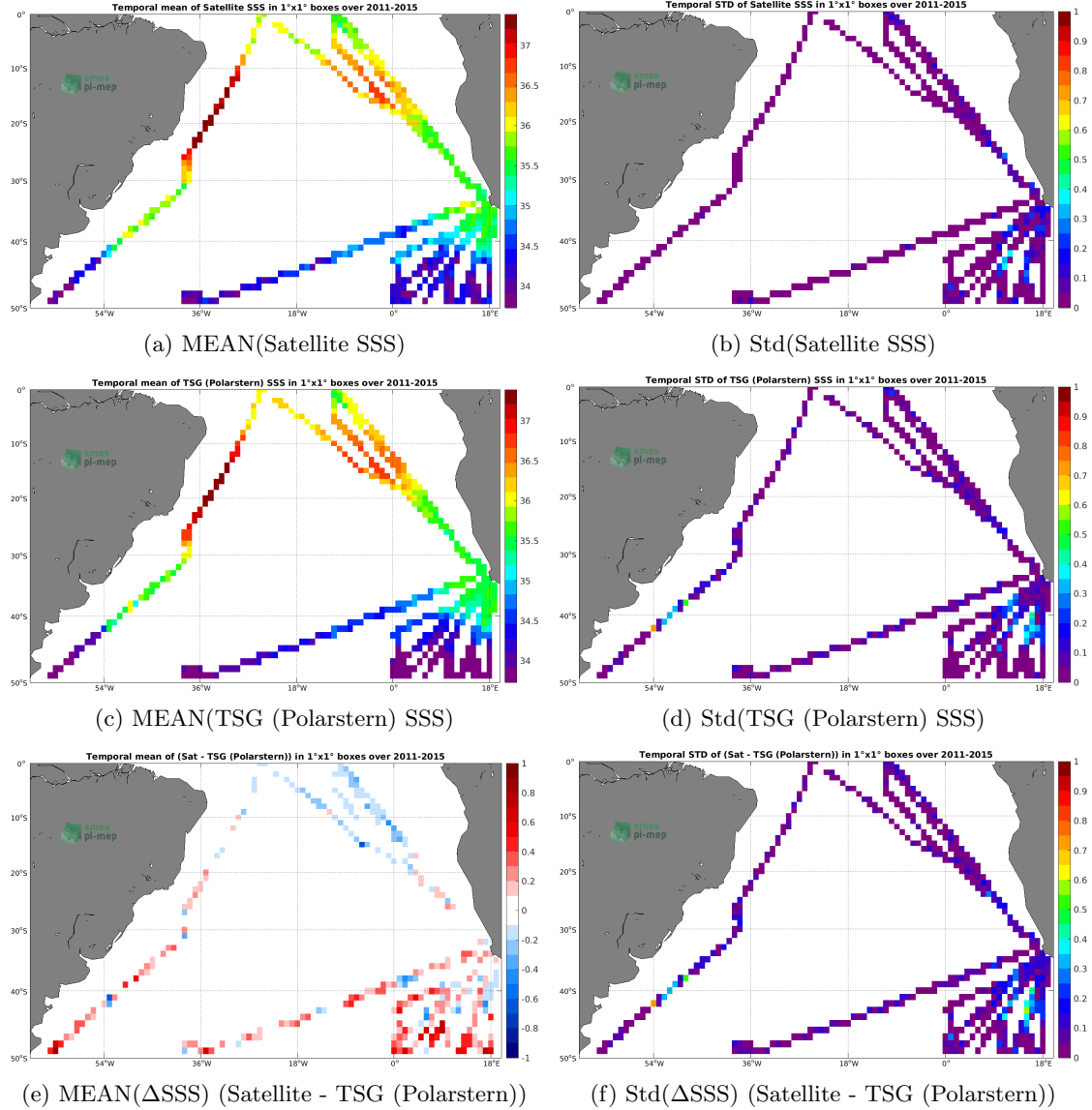
Figure 6: Temporal mean (left) and Std (right) of SSS from Aquarius SSS L3 CAP v5 - 7-Day running (JPL) (top), TSG (Polarstern) (middle), and of \Delta SSS (Satellite - TSG (Polarstern)). Only match-up pairs are used to generate these maps.
