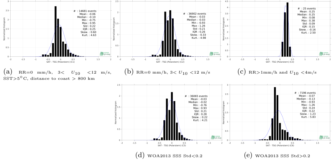
Figure 13: Normalized histogram of \Delta SSS (Aquarius SSS L3 CAP v5 - 7-Day running (JPL) - TSG (Polarstern)) for 5 different subdatasets corresponding to: RR=0 mm/h, 3 < U_{10} < 12 m/s, SST>5°C, distance to coast > 800 km (a), RR=0 mm/h, 3 < U_{10} < 12 m/s (b), RR>1mm/h and U_{10} < 4 m/s (c), WOA2013 SSS Std<0.2 (d), WOA2013 SSS Std>0.2 (e).
