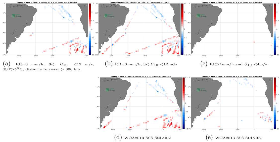
Figure 12: Temporal mean gridded over spatial boxes of size 1^\circ \times 1^\circ of \Delta SSS (Aquarius SSS L3 CAP v5 - 7-Day running (JPL) - TSG (Polarstern)) for 5 different subdatasets corresponding to: RR=0 mm/h, 3 < U_{10} < 12 m/s, SST > 5^\circ C , distance to coast > 800 km (a), RR=0 mm/h, 3 < U_{10} < 12 m/s (b), RR > 1 mm/h and U_{10} < 4 m/s (c), WOA2013 SSS Std < 0.2 (d), WOA2013 SSS Std > 0.2 (e).
