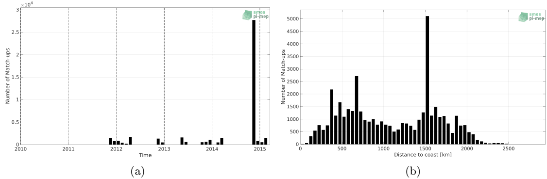
Figure 1: Number of match-ups between TSG (Polarstern) and Aquarius SSS L3 CAP v5 - 7-Day running (JPL) SSS as a function of time (a) and as function of the distance to coast (b) over the South Atlantic Ocean Pi-MEP region and for the full satellite product period.
