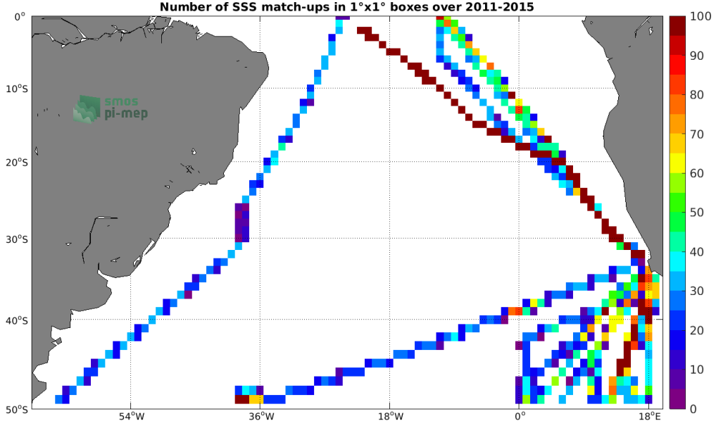
Figure 4: Number of SSS match-ups between TSG (Polarstern) SSS and the Aquarius SSS L3 CAP v5 - 7-Day running (JPL) SSS product for the South Atlantic Ocean Pi-MEP region over 1^\circ \times 1^\circ boxes and for the full satellite product period.
