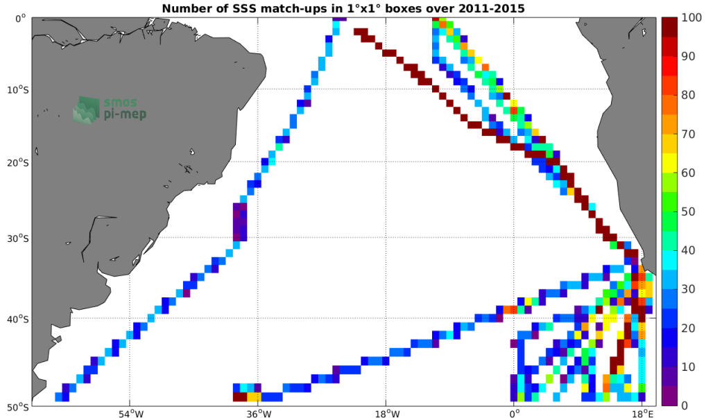
Figure 4: Number of SSS match-ups between TSG-POLARSTERN SSS and the Aquarius-L3-JPL-V5-7DAY-RUNNING SSS product for the South Atlantic Ocean Pi-MEP region over 1^\circ \times 1^\circ boxes and for the full satellite product period.
