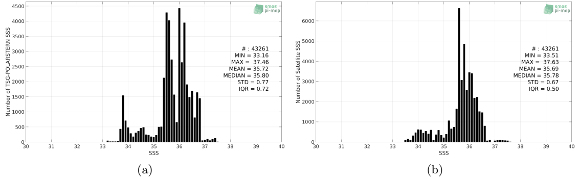
Figure 2: Histograms of SSS from TSG-POLARSTERN (a) and Aquarius-L3-JPL-V5-7DAY-RUNNING (b) considering all match-up pairs per bins of 0.1 over the South Atlantic Ocean Pi-MEP region and for the full satellite product period.
