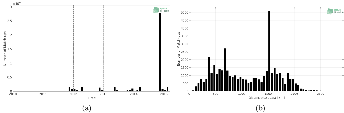
Figure 1: Number of match-ups between TSG-POLARSTERN and Aquarius-L3-JPL-V5-7DAY-RUNNING SSS as a function of time (a) and as function of the distance to coast (b) over the South Atlantic Ocean Pi-MEP region and for the full satellite product period.
