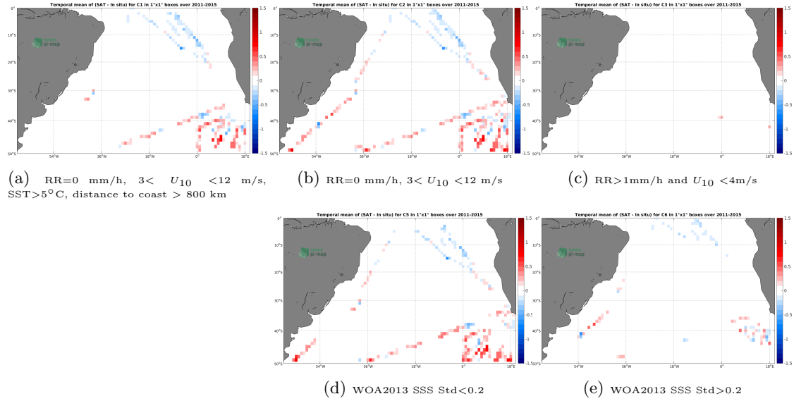
Figure 12: Temporal mean gridded over spatial boxes of size 1^\circ \times 1^\circ of \Delta SSS (Aquarius-L3-JPL-V5-7DAY-RUNNING - TSG-POLARSTERN) for 5 different subdatasets corresponding to: RR=0 mm/h, 3 < U_{10} < 12 m/s, SST > 5^\circ C , distance to coast > 800 km (a), RR=0 mm/h, 3 < U_{10} < 12 m/s (b), RR > 1 mm/h and U_{10} < 4 m/s (c), WOA2013 SSS Std < 0.2 (d), WOA2013 SSS Std > 0.2 (e).
