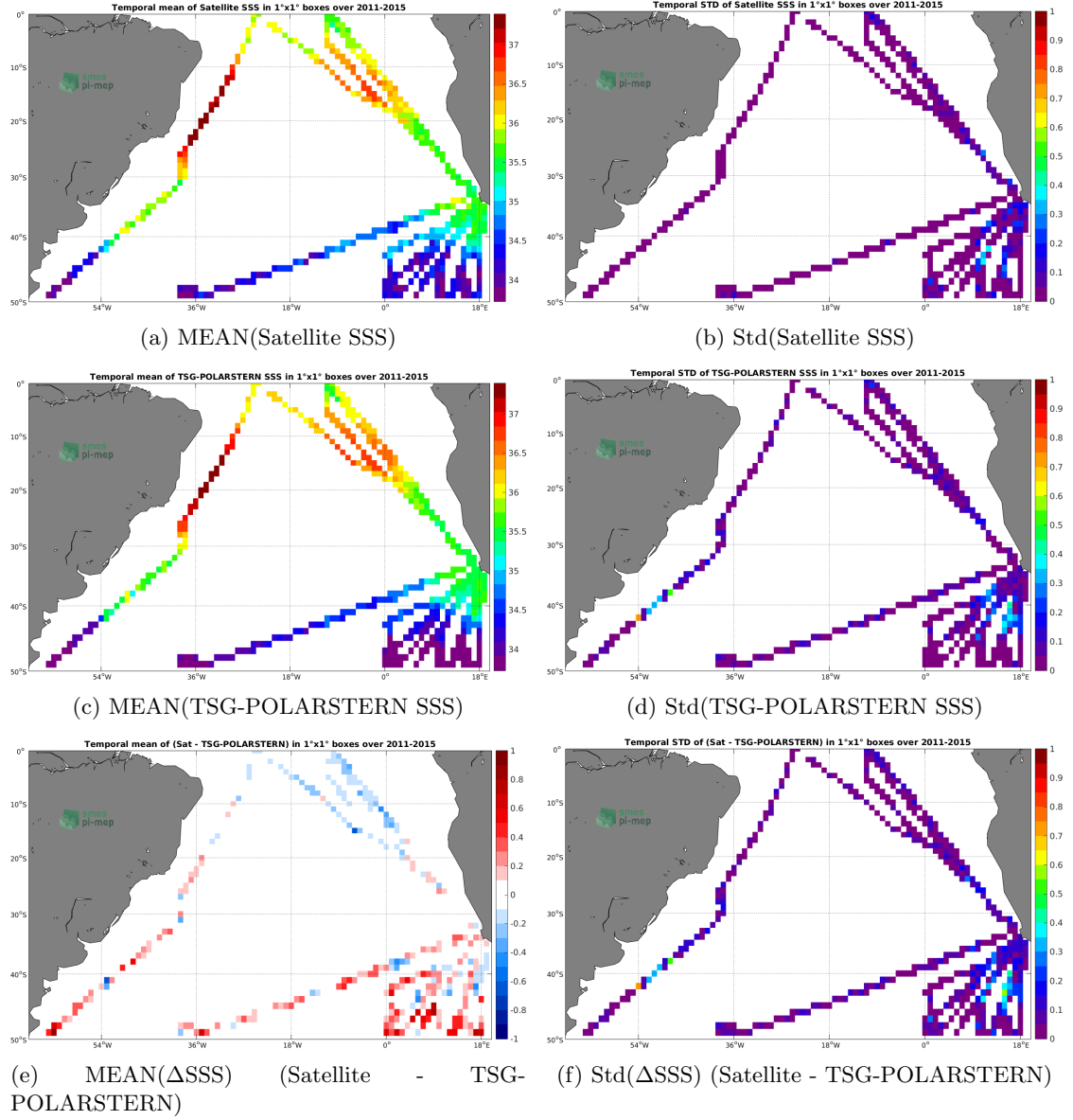
Figure 6: Temporal mean (left) and Std (right) of SSS from Aquarius-L3-JPL-V5-7DAY-RUNNING (top), TSG-POLARSTERN (middle), and of \Delta SSS (Satellite - TSG-POLARSTERN). Only match-up pairs are used to generate these maps.
