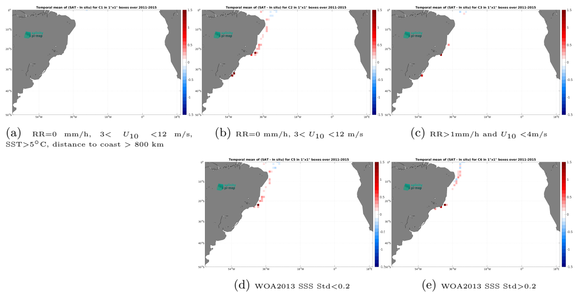
Figure 14: Temporal mean gridded over spatial boxes of size 1^\circ \times 1^\circ of \Delta SSS (Aquarius SSS L3 CAP v5 - 7-Day running (JPL) - TSG (LEGOS-DM)) for 5 different subdatasets corresponding to:RR=0 mm/h, 3 < U_{10} < 12 m/s, SST >5^\circ\text{C} , distance to coast > 800 km (a), RR=0 mm/h, 3 < U_{10} < 12 m/s (b), RR >1 mm/h and U_{10} < 4 m/s (c), WOA2013 SSS Std <0.2 (d), WOA2013 SSS Std >0.2 (e).
