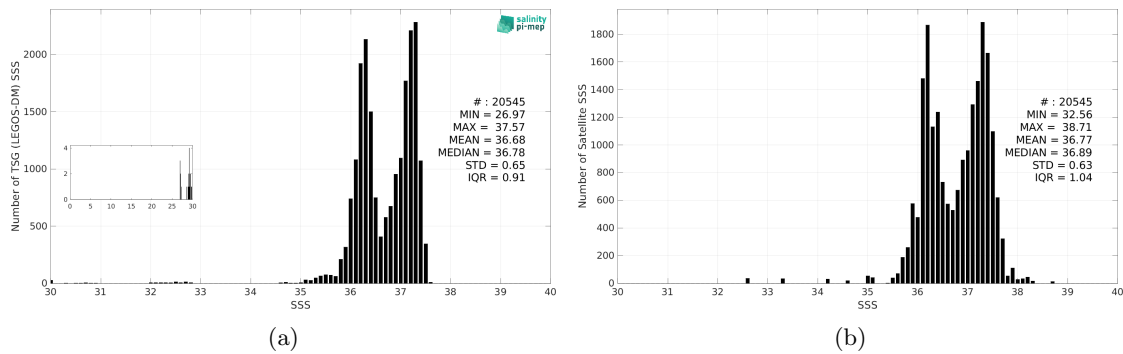
Figure 3: Histograms of SSS from TSG (LEGOS-DM) (a) and Aquarius SSS L3 CAP v5 - 7-Day running (JPL) (b) considering all match-up pairs per bins of 0.1 over the South Atlantic Ocean Pi-MEP region and for the full satellite product period.
