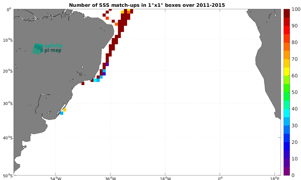
Figure 5: Number of SSS match-ups between TSG (LEGOS-DM) SSS and the Aquarius SSS L3 CAP v5 - 7-Day running (JPL) SSS product for the South Atlantic Ocean Pi-MEP region over 1^\circ \times 1^\circ boxes and for the full satellite product period.
