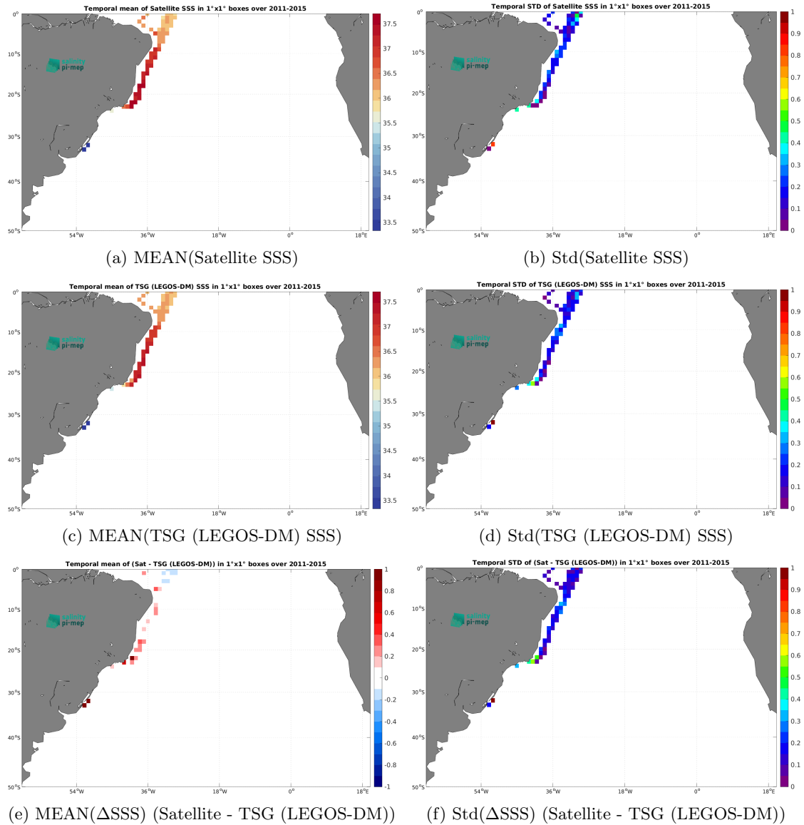
Figure 7: Temporal mean (left) and Std (right) of SSS from Aquarius SSS L3 CAP v5 - 7-Day running (JPL) (top), TSG (LEGOS-DM) (middle), and of \Delta SSS (Satellite - TSG (LEGOS-DM)). Only match-up pairs are used to generate these maps.
