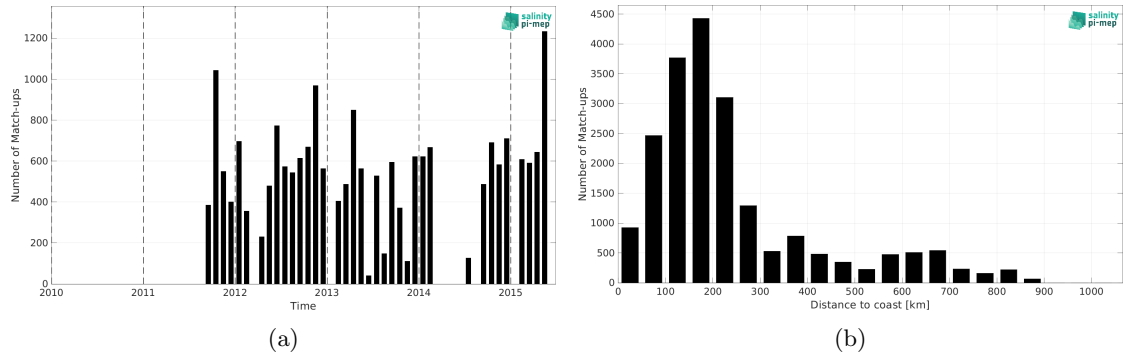
Figure 2: Number of match-ups between TSG (LEGOS-DM) and Aquarius SSS L3 CAP v5 - 7-Day running (JPL) SSS as a function of time (a) and as function of the distance to coast (b) over the South Atlantic Ocean Pi-MEP region and for the full satellite product period.
