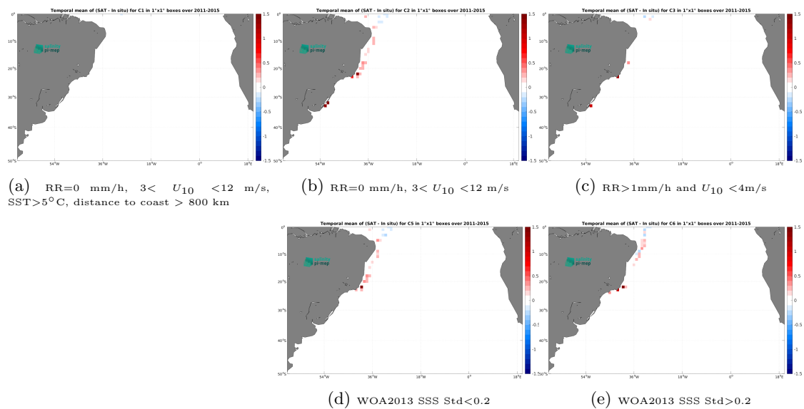
Figure 14: Temporal mean gridded over spatial boxes of size 1^\circ \times 1^\circ of \Delta SSS (Aquarius SSS L3 CAP v5 - 7-Day running (JPL) - TSG (LEGOS-DM)) for 5 different subdatasets corresponding to:RR=0 mm/h, 3 < U_{10} < 12 m/s, SST >5^\circ\text{C} , distance to coast > 800 km (a), RR=0 mm/h, 3 < U_{10} < 12 m/s (b), RR >1 mm/h and U_{10} < 4 m/s (c), WOA2013 SSS Std <0.2 (d), WOA2013 SSS Std >0.2 (e).
