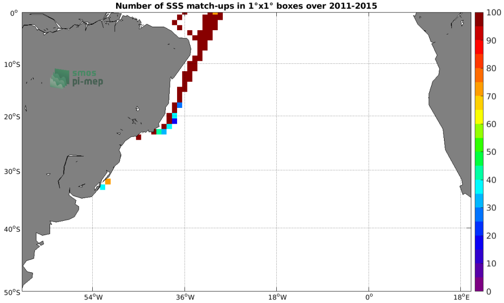
Figure 4: Number of SSS match-ups between TSG (LEGOS-DM) SSS and the Aquarius SSS L3 CAP v5 - 7-Day running (JPL) SSS product for the South Atlantic Ocean Pi-MEP region over 1^\circ \times 1^\circ boxes and for the full satellite product period.
