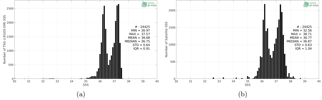
Figure 2: Histograms of SSS from TSG (LEGOS-DM) (a) and Aquarius SSS L3 CAP v5 - 7-Day running (JPL) (b) considering all match-up pairs per bins of 0.1 over the South Atlantic Ocean Pi-MEP region and for the full satellite product period.
