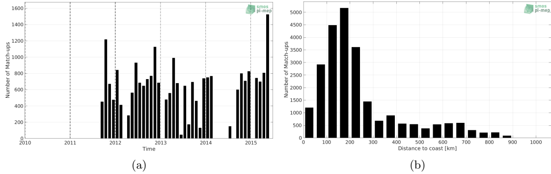
Figure 1: Number of match-ups between TSG (LEGOS-DM) and Aquarius SSS L3 CAP v5 - 7-Day running (JPL) SSS as a function of time (a) and as function of the distance to coast (b) over the South Atlantic Ocean Pi-MEP region and for the full satellite product period.
