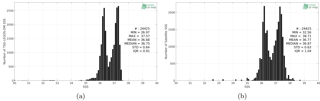
Figure 2: Histograms of SSS from TSG-LEGOS-DM (a) and Aquarius-L3-JPL-V5-7DAY-RUNNING (b) considering all match-up pairs per bins of 0.1 over the South Atlantic Ocean Pi-MEP region and for the full satellite product period.
