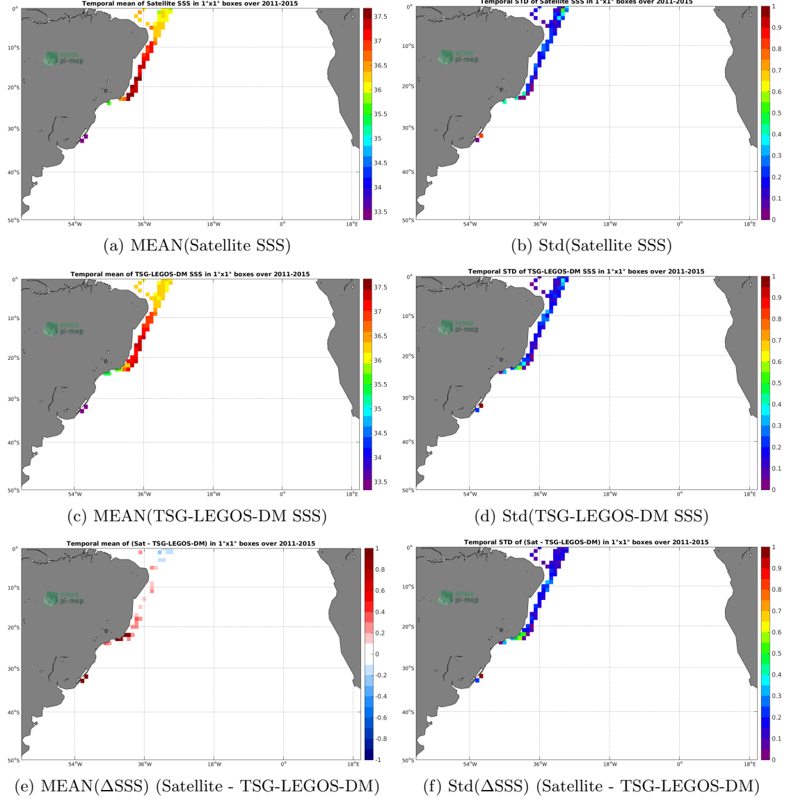
Figure 6: Temporal mean (left) and Std (right) of SSS from Aquarius-L3-JPL-V5-7DAY-RUNNING (top), TSG-LEGOS-DM (middle), and of \Delta SSS (Satellite - TSG-LEGOS-DM). Only match-up pairs are used to generate these maps.
