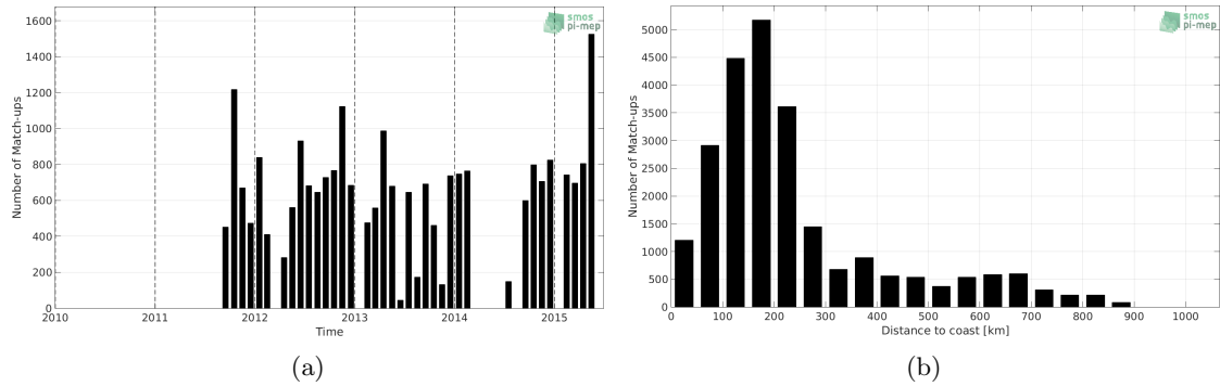
Figure 1: Number of match-ups between TSG-LEGOS-DM and Aquarius-L3-JPL-V5-7DAY-RUNNING SSS as a function of time (a) and as function of the distance to coast (b) over the South Atlantic Ocean Pi-MEP region and for the full satellite product period.
