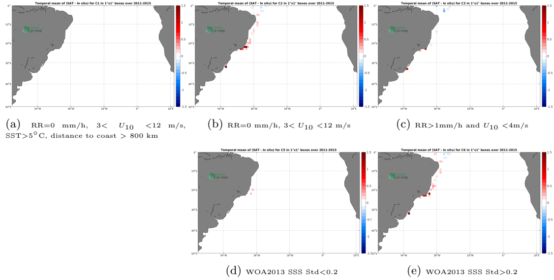
Figure 12: Temporal mean gridded over spatial boxes of size 1^\circ \times 1^\circ of \Delta SSS (Aquarius-L3-JPL-V5-7DAY-RUNNING - TSG-LEGOS-DM) for 5 different subdatasets corresponding to: RR=0 mm/h, 3 < U_{10} < 12 m/s, SST > 5^\circ\text{C} , distance to coast > 800 km (a), RR=0 mm/h, 3 < U_{10} < 12 m/s (b), RR > 1\text{mm/h} and U_{10} < 4\text{m/s} (c), WOA2013 SSS Std < 0.2 (d), WOA2013 SSS Std > 0.2 (e).
