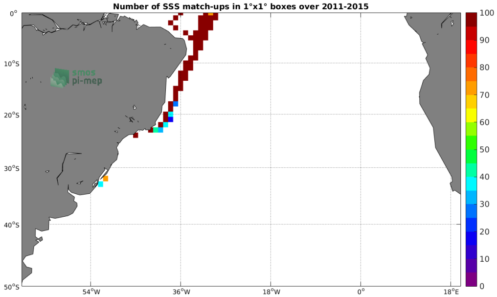
Figure 4: Number of SSS match-ups between TSG-LEGOS-DM SSS and the Aquarius-L3-JPL-V5-7DAY-RUNNING SSS product for the South Atlantic Ocean Pi-MEP region over 1^\circ \times 1^\circ boxes and for the full satellite product period.
