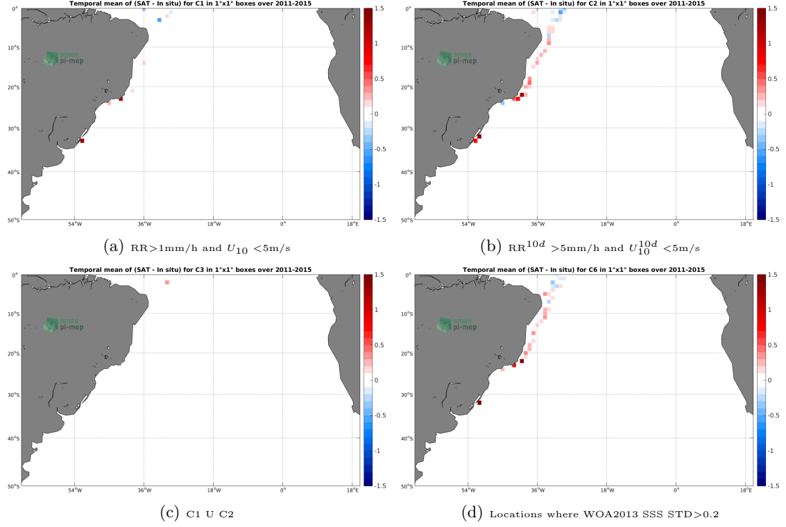
Figure 12: Temporal mean gridded over spatial boxes of size 1^\circ \times 1^\circ of \Delta SSS (Aquarius-L3-JPL-V5-7DAY-RUNNING - TSG-LEGOS-DM) for 4 different subdatasets corresponding to: RR > 1\text{mm/h} and U_{10} < 5\text{m/s} (a), RR^{10d} > 5\text{mm/h} and U_{10}^{10d} < 5\text{m/s} (b), C1 U C2 (c), Locations where WOA2013 SSS STD > 0.2 (d).
