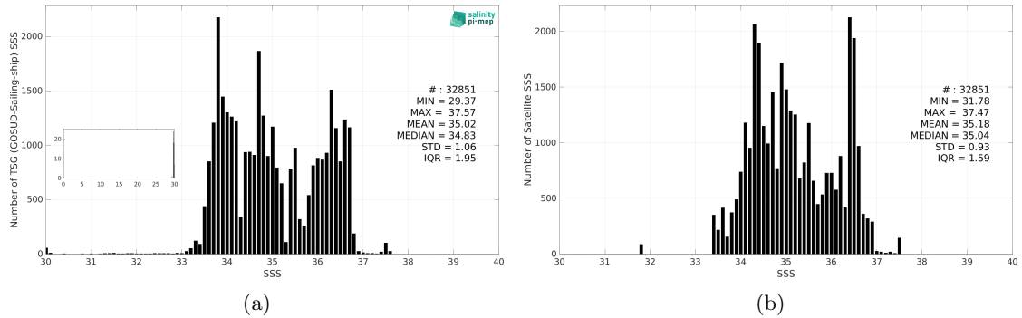
Figure 3: Histograms of SSS from TSG (GOSUD-Sailing-ship) (a) and Aquarius SSS L3 CAP v5 - 7-Day running (JPL) (b) considering all match-up pairs per bins of 0.1 over the South Atlantic Ocean Pi-MEP region and for the full satellite product period.
