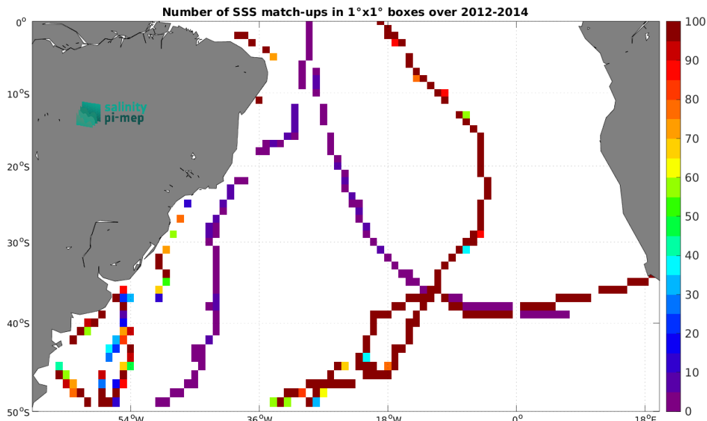
Figure 5: Number of SSS match-ups between TSG (GOSUD-Sailing-ship) SSS and the Aquarius SSS L3 CAP v5 - 7-Day running (JPL) SSS product for the South Atlantic Ocean Pi-MEP region over 1^\circ \times 1^\circ boxes and for the full satellite product period.
