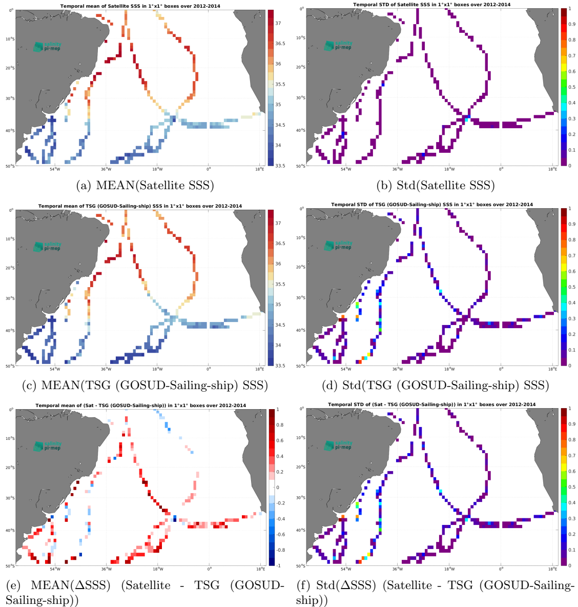
Figure 7: Temporal mean (left) and Std (right) of SSS from Aquarius SSS L3 CAP v5 - 7-Day running (JPL) (top), TSG (GOSUD-Sailing-ship) (middle), and of \Delta SSS (Satellite - TSG (GOSUD-Sailing-ship)). Only match-up pairs are used to generate these maps.
