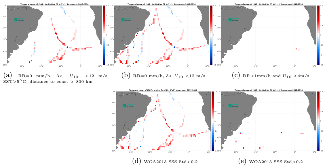
Figure 14: Temporal mean gridded over spatial boxes of size 1^\circ \times 1^\circ of \Delta\text{SSS} (Aquarius SSS L3 CAP v5 - 7-Day running (JPL) - TSG (GOSUD-Sailing-ship)) for 5 different subdatasets corresponding to:RR=0 mm/h, 3 < U_{10} < 12 m/s, SST>5°C, distance to coast > 800 km (a), RR=0 mm/h, 3 < U_{10} < 12 m/s (b), RR>1mm/h and U_{10} < 4 m/s (c), WOA2013 SSS Std<0.2 (d), WOA2013 SSS Std>0.2 (e).
