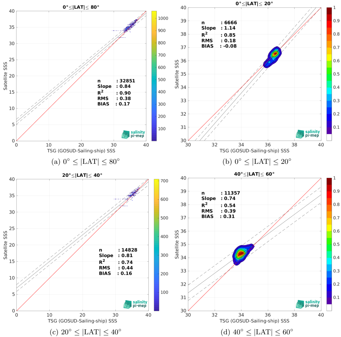
Figure 10: Contour maps of the concentration of Aquarius SSS L3 CAP v5 - 7-Day running (JPL) SSS (y-axis) versus TSG (GOSUD-Sailing-ship) SSS (x-axis) at match-up pairs for different latitude bands. For each plot, the red line shows x=y . The black thin and dashed lines indicate a linear fit through the data cloud and the \pm 95\% confidence levels, respectively. The number match-up pairs n , the slope and R^2 coefficient of the linear fit, the root mean square (RMS) and the mean bias between satellite and in situ data are indicated for each latitude band in each plots.
