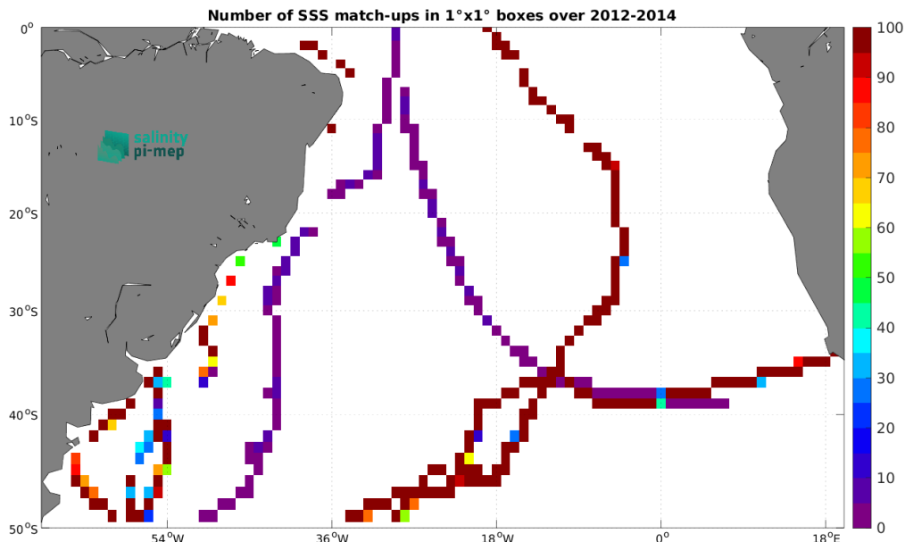
Figure 4: Number of SSS match-ups between TSG (GOSUD-Sailing-ship) SSS and the Aquarius SSS L3 CAP v5 - 7-Day running (JPL) SSS product for the South Atlantic Ocean Pi-MEP region over 1^\circ \times 1^\circ boxes and for the full satellite product period.
