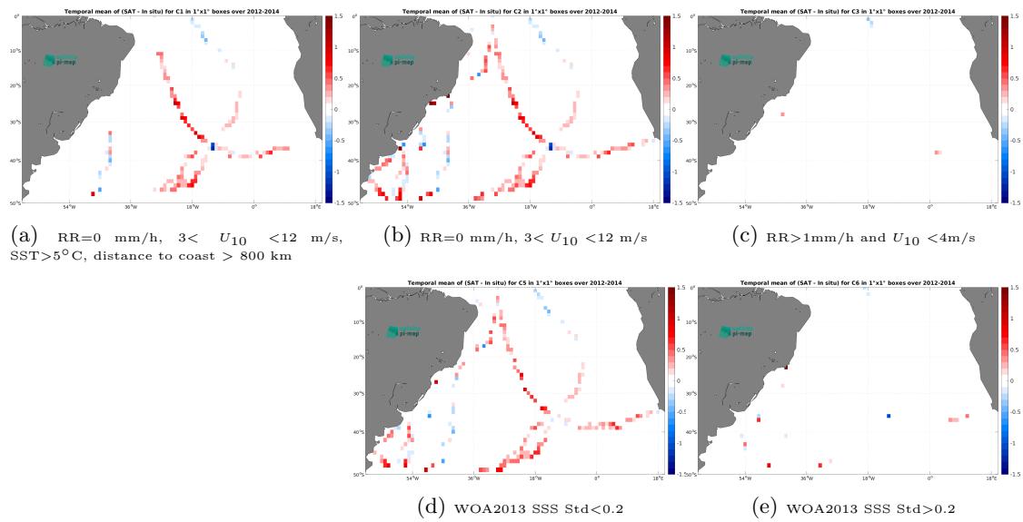
Figure 12: Temporal mean gridded over spatial boxes of size 1^\circ \times 1^\circ of \Delta\text{SSS} (Aquarius SSS L3 CAP v5 - 7-Day running (JPL) - TSG (GOSUD-Sailing-ship)) for 5 different subdatasets corresponding to:RR=0 mm/h, 3 < U_{10} < 12 m/s, SST >5^\circ\text{C} , distance to coast > 800 km (a), RR=0 mm/h, 3 < U_{10} < 12 m/s (b), RR >1 mm/h and U_{10} < 4 m/s (c), WOA2013 SSS Std <0.2 (d), WOA2013 SSS Std >0.2 (e).
