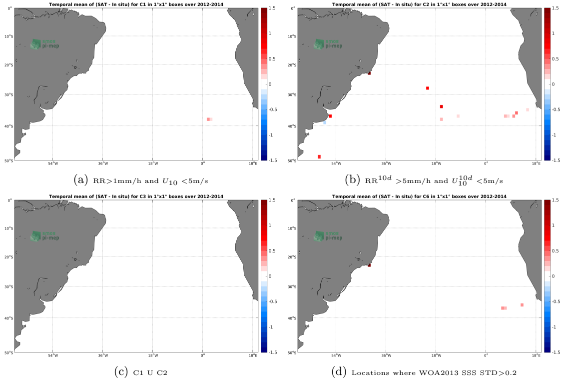
Figure 12: Temporal mean gridded over spatial boxes of size 1^\circ \times 1^\circ of \Delta SSS (Aquarius-L3-JPL-V5-7DAY-RUNNING - TSG-GOSUD-Sailing-ship) for 4 different subdatasets corresponding to: RR > 1mm/h and U_{10} < 5\text{m/s} (a), RR^{10d} > 5\text{mm/h} and U_{10}^{10d} < 5\text{m/s} (b), C1 U C2 (c), Locations where WOA2013 SSS STD > 0.2 (d).
