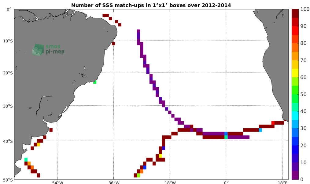
Figure 4: Number of SSS match-ups between TSG-GOSUD-Sailing-ship SSS and the Aquarius-L3-JPL-V5-7DAY-RUNNING SSS product for the South Atlantic Ocean Pi-MEP region over 1^\circ \times 1^\circ boxes and for the full satellite product period.
