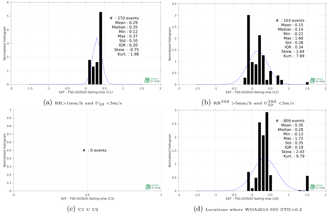
Figure 13: Normalized histogram of \Delta SSS (Aquarius-L3-JPL-V5-7DAY-RUNNING - TSG-GOSUD-Sailing-ship) for 6 different subdatasets corresponding to: RR > 1\text{mm/h} and U_{10} < 5\text{m/s} (a), RR^{10d} > 5\text{mm/h} and U_{10}^{10d} < 5\text{m/s} (b), C1 U C2 (c), Locations where WOA2013 SSS STD > 0.2 (d).
