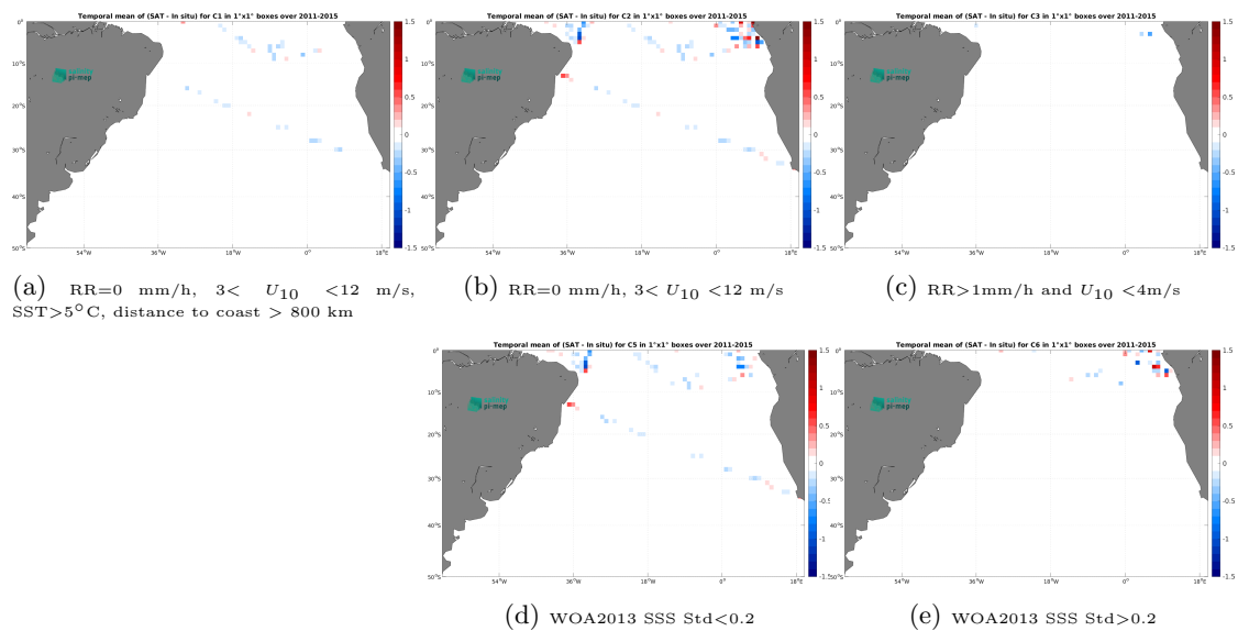
Figure 14: Temporal mean gridded over spatial boxes of size 1^\circ \times 1^\circ of \Delta\text{SSS} (Aquarius SSS L3 CAP v5 - 7-Day running (JPL) - TSG (GOSUD-Research-vessel)) for 5 different subdatasets corresponding to:RR=0 mm/h, 3 < U_{10} < 12 m/s, SST >5^\circ\text{C} , distance to coast > 800 km (a), RR=0 mm/h, 3 < U_{10} < 12 m/s (b), RR >1 mm/h and U_{10} < 4 m/s (c), WOA2013 SSS Std <0.2 (d), WOA2013 SSS Std >0.2 (e).
