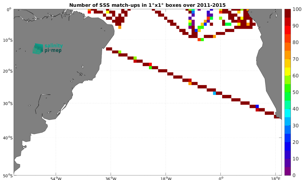
Figure 4: Number of SSS match-ups between TSG (GOSUD-Research-vessel) SSS and the Aquarius SSS L3 CAP v5 - 7-Day running (JPL) SSS product for the South Atlantic Ocean Pi-MEP region over 1^\circ \times 1^\circ boxes and for the full satellite product period.
