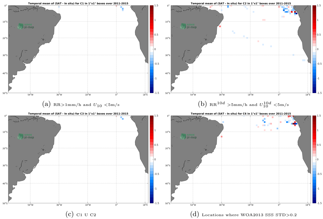
Figure 12: Temporal mean gridded over spatial boxes of size 1^\circ \times 1^\circ of \Delta SSS (Aquarius-L3-JPL-V5-7DAY-RUNNING - TSG-GOSUD-Research-vessel) for 4 different subdatasets corresponding to: RR > 1\text{mm/h} and U_{10} < 5\text{m/s} (a), RR^{10d} > 5\text{mm/h} and U_{10}^{10d} < 5\text{m/s} (b), C1 U C2 (c), Locations where WOA2013 SSS STD > 0.2 (d).
