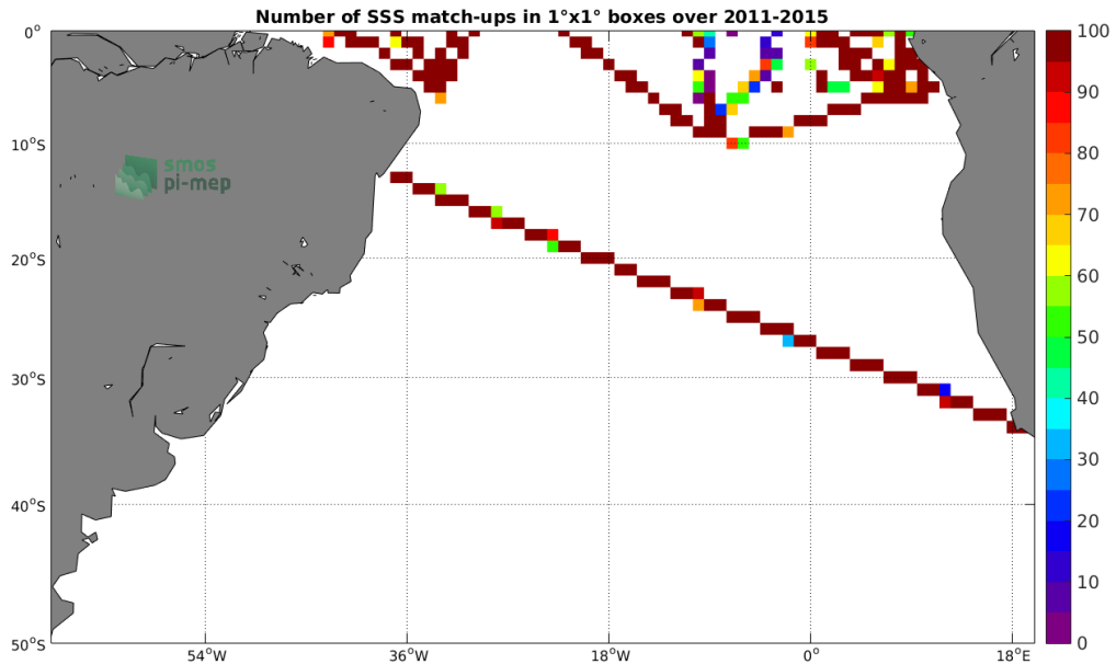
Figure 4: Number of SSS match-ups between TSG-GOSUD-Research-vessel SSS and the Aquarius-L3-JPL-V5-7DAY-RUNNING SSS product for the South Atlantic Ocean Pi-MEP region over 1^\circ \times 1^\circ boxes and for the full satellite product period.
